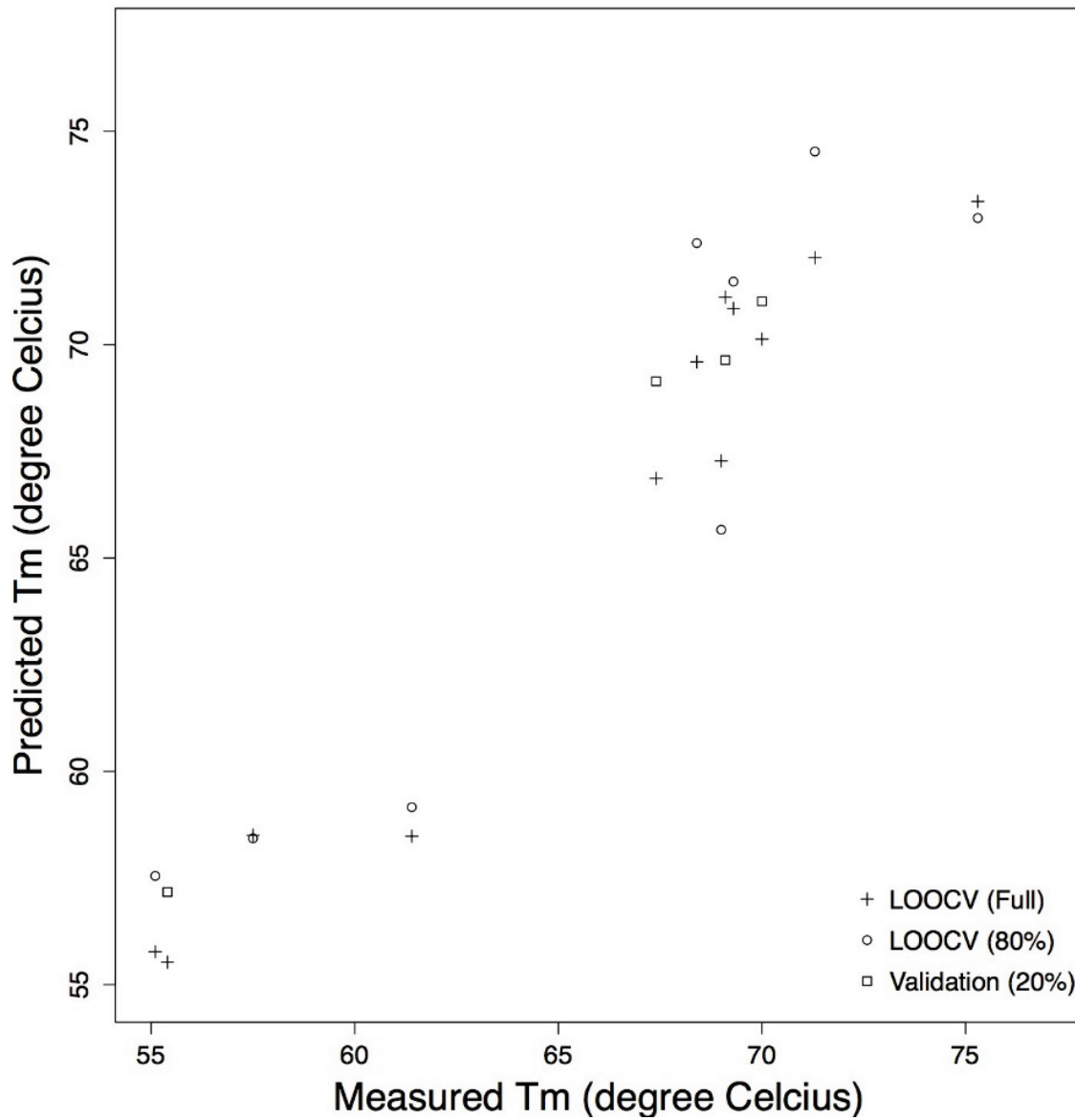
Figure S2. Plot of measured thermostability of enterotoxin variants versus predicted thermostability using iSAR algorithm.
