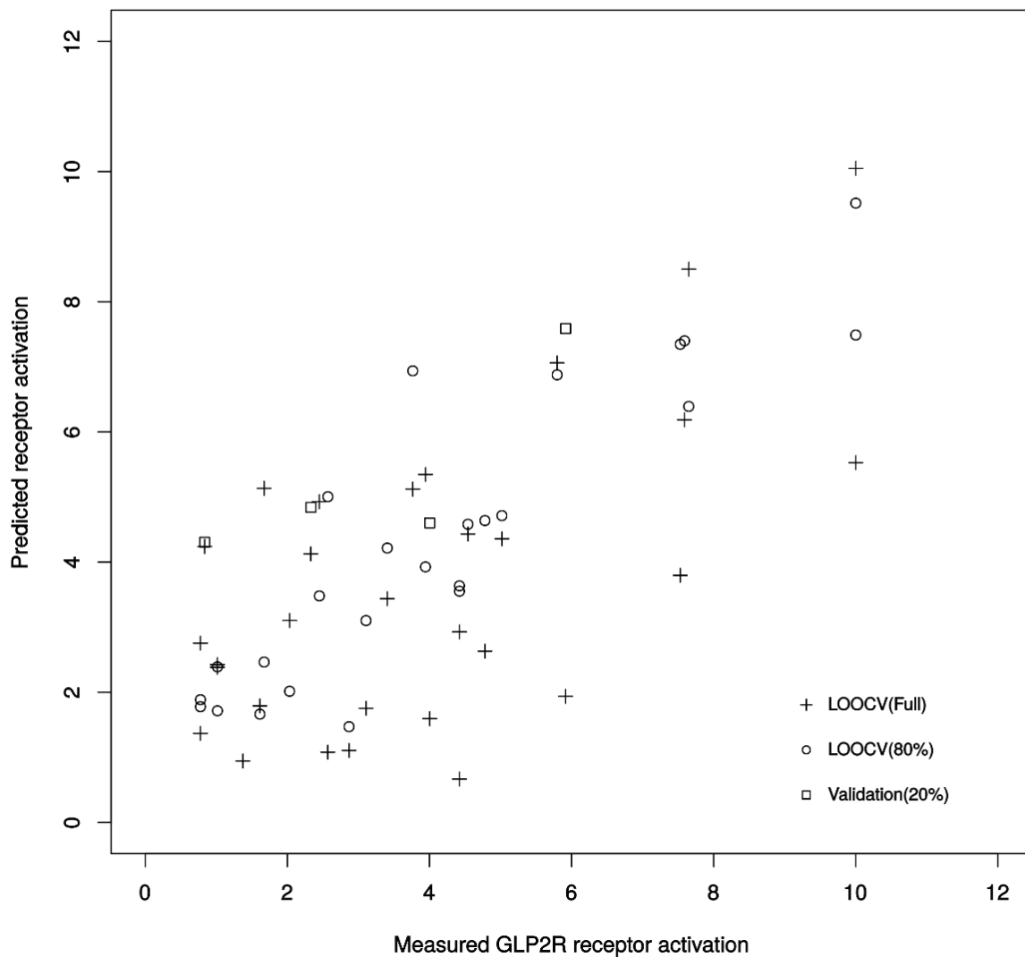
Figure S3. Plot of measured GLP2R receptor activation of GLP2 variants versus predicted receptor activation using iSAR algorithm
