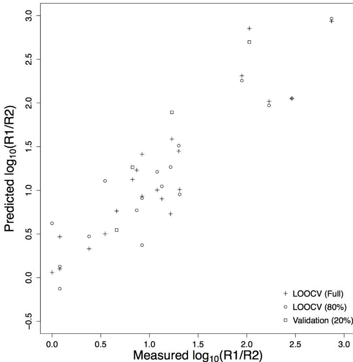
Figure S1. Plot of measured affinity of TNF variants versus predicted affinity using iSAR algorithm.
