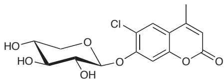
6-chloro-4-methylumbelliferyl xyloside
