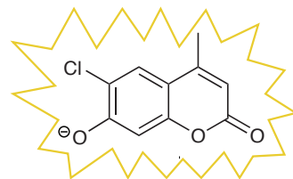
6-chloro-4-methylumbelliferone
