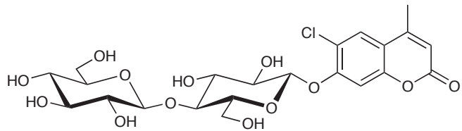
6-chloro-4-methylumbelliferyl cellobioside
