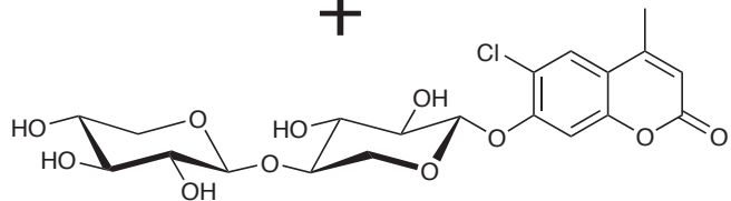
6-chloro-4-methylumbelliferyl xylobioside
