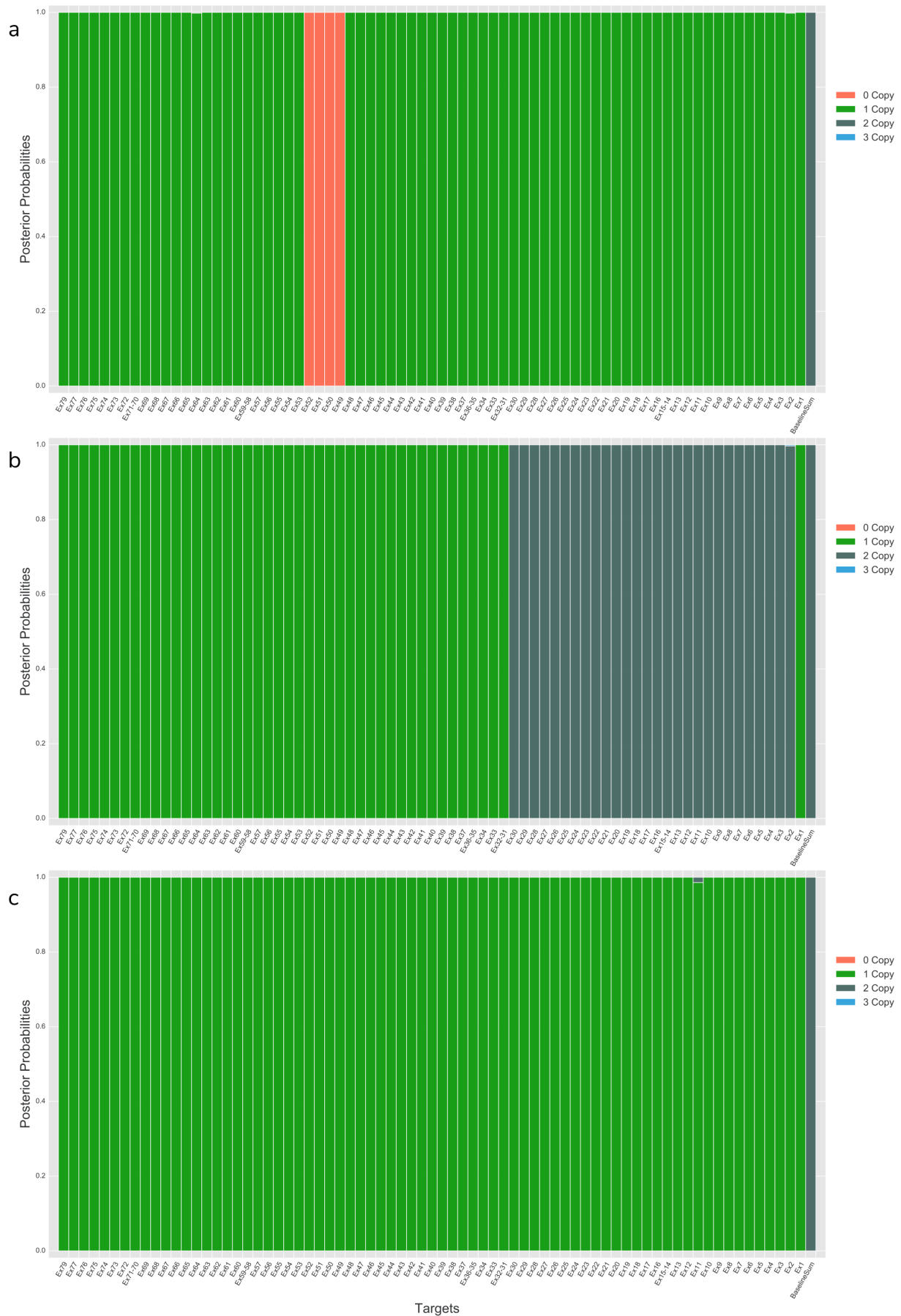
Figure S7: CNV identification in male subjects Results for male research and volunteer subjects using geneCNV trained on 38 female subject samples (a) Coriell subject NA04100 (EX49-52 deletion). (b) Coriell subject NA23086 (EX2-30DUP). (c) Volunteer subject with no known CNVs.
