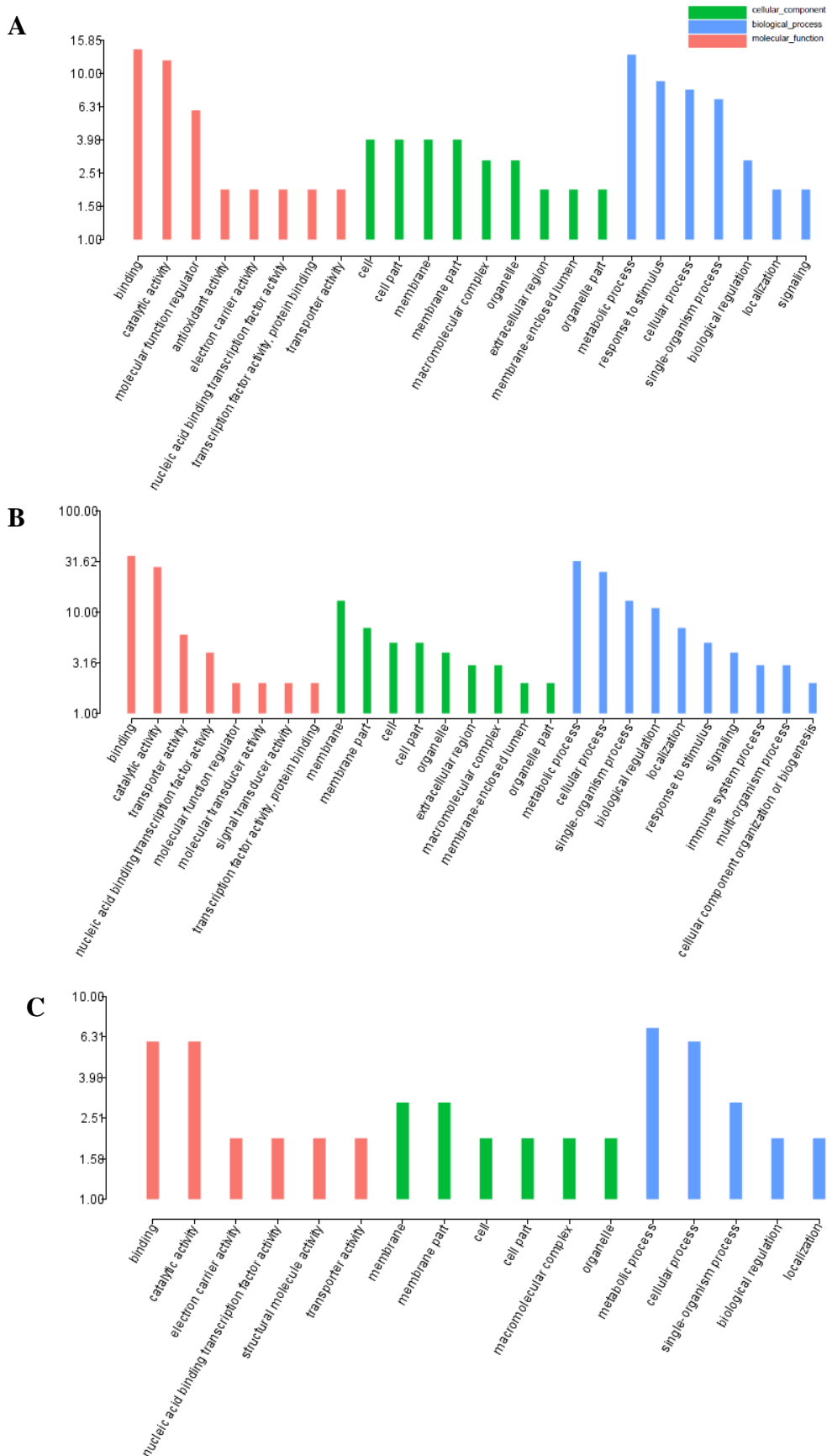
Supplementary Figure S5. GO annotation for DEGs. All the Type I (A), Type II (B), and Type III (C) DEGs were categorized by their GO annotations into different functional groups of three main categories: biological process, cellular component, and molecular function. The y-axis indicates the percentage of genes in a category.
