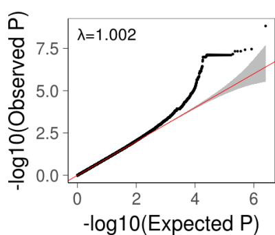
SNP
