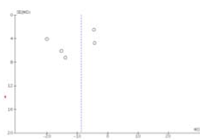
Funnel plot of procedural time
