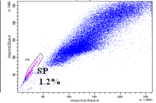
Gate showing SP cells and population outside gated area represents NSP cell
