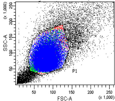
FSC vs SSC for debris exclusion
