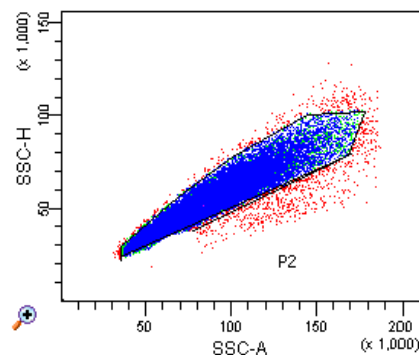
Gate showing single cells excluding doublets and aggregates
