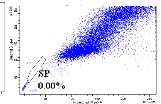
Gate showing SP cells and population outside gated area represents NSP cell
