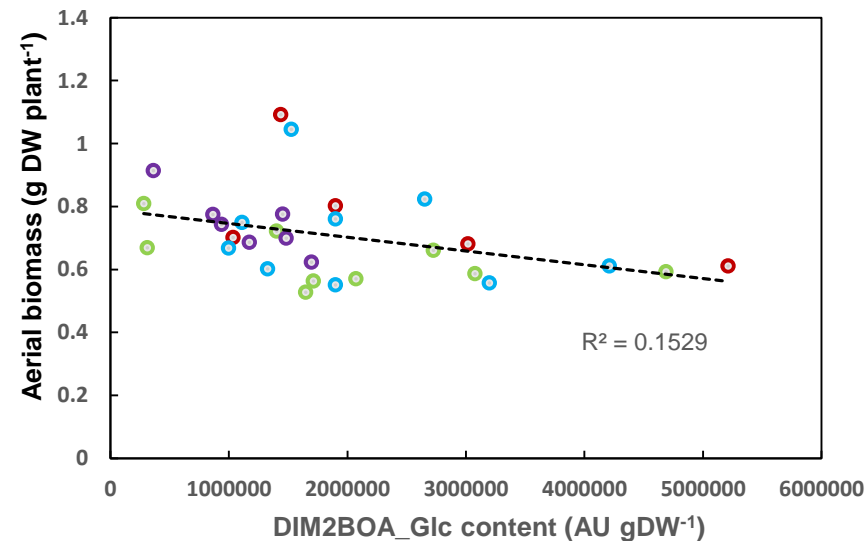
Supplementary Figure S3: Metabolites directly correlated with aerial biomass in the normal sowing or early sowing condition in Figures 4A or 4B networks. Biomass-metabolite biplots for the genotype lsmeans. Genotypes are colored according to their group (European, green; lodent, purple; Lancaster, red; Stiff Stalk, blue). The regression line and R^2 value correspond to all genotypes.
