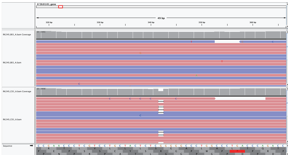
Figure S1: A single-base deletion in exon 1 of the HLA-A gene of patient RK249. IGV screenshots were taken at the position for the WGS data (upper) and the TruSight HLA Sequencing Panel data (lower). In each of the screenshots, the upper and lower tracks correspond to the normal and tumor samples, respectively.
