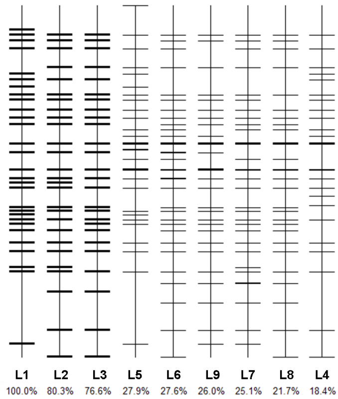
S2 Fig. DGGE fingerprint sketch to order the samples according to their similarities comparing with L1 which represents the bacterial community of original activated sludge.
