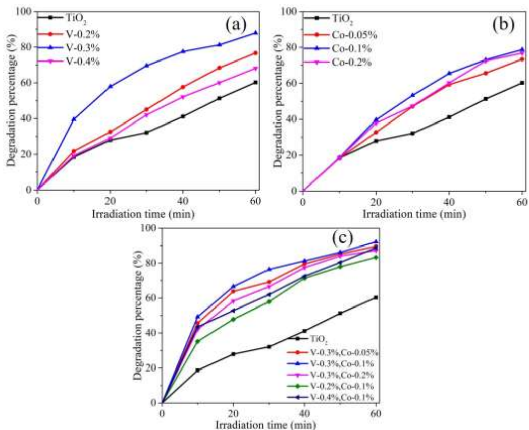
Figure S1. Degradation percentage of MB by V and Co doped TiO 2 samples prepared at pH 1.5 and sintered at 500 °C. (a) V-TiO 2 of different doping quantities; (b) Co-TiO 2 of different doping quantities; (c) (V, Co)-TiO 2 of different doping quantities.
