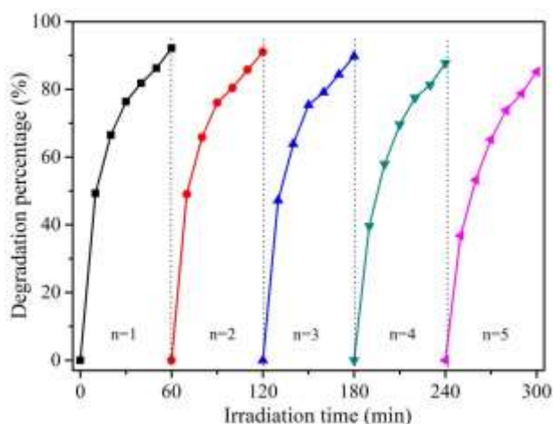
Figure.S2. Five recyclable visible-light catalytic degradation experiments using (V, Co)-TiO 2 photocatalyst in 0.01g L -1 MB solution.
