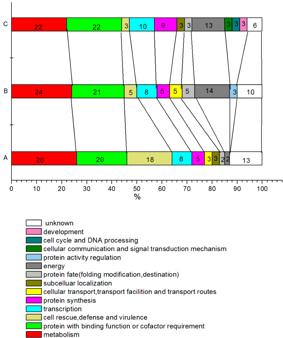
Figure S1. Functional categorization of identified up- and down-regulated proteins in Chlorella pyrenoidosa after treatment with mitochondrial respiratory electron transport chain (mRET) inhibitors. (A) Salicylhydroxamic acid (SHAM) treatment; (B) antimycin A treatment; (C) sodium azide (NaN 3 ) treatment. This classification is based on homologies.
