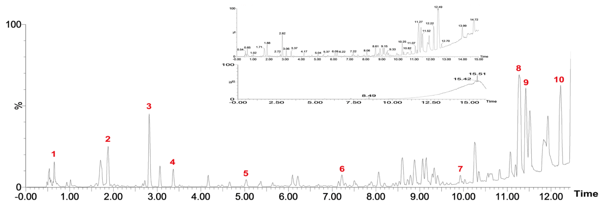
Supplementary Figure S1. Chromatographic peaks of Spirulina platensis ethanol extract in UPLC.
