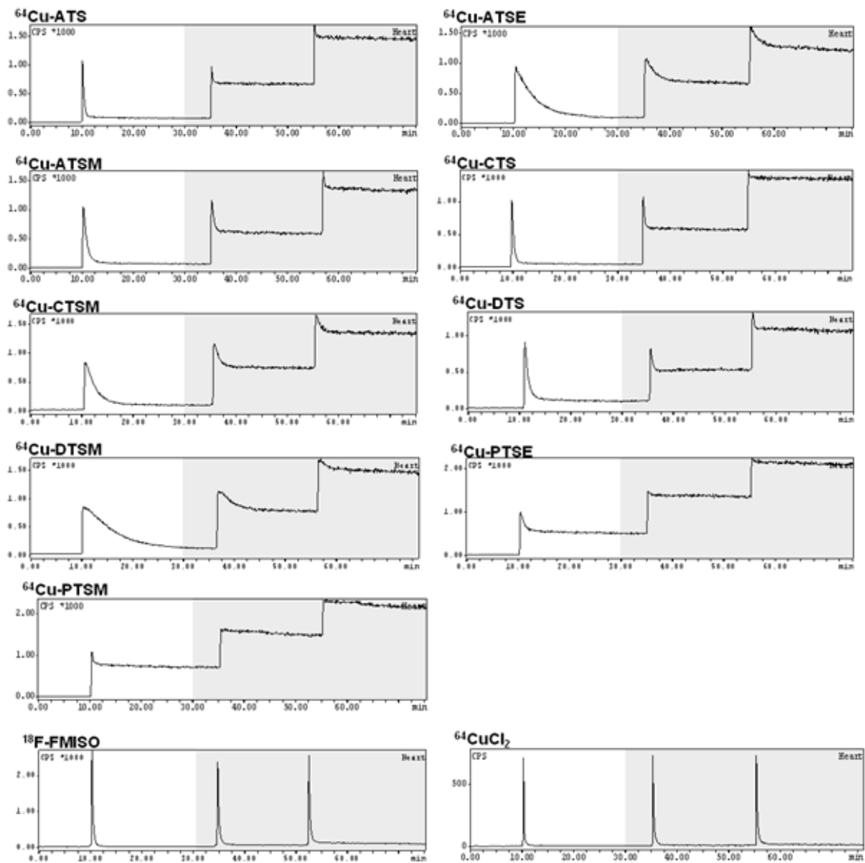
Supplemental Figure 1. Representative time-activity curves showing the myocardial clearance/accumulation of all ^{64}\text{Cu} -BTSCs tested, ^{18}\text{F} -fluoromisonidazole (FMISO), and ^{64}\text{CuCl}_2 during normoxia (white background) and then hypoxia (gray background). Each spike represents a 1-MBq bolus.
