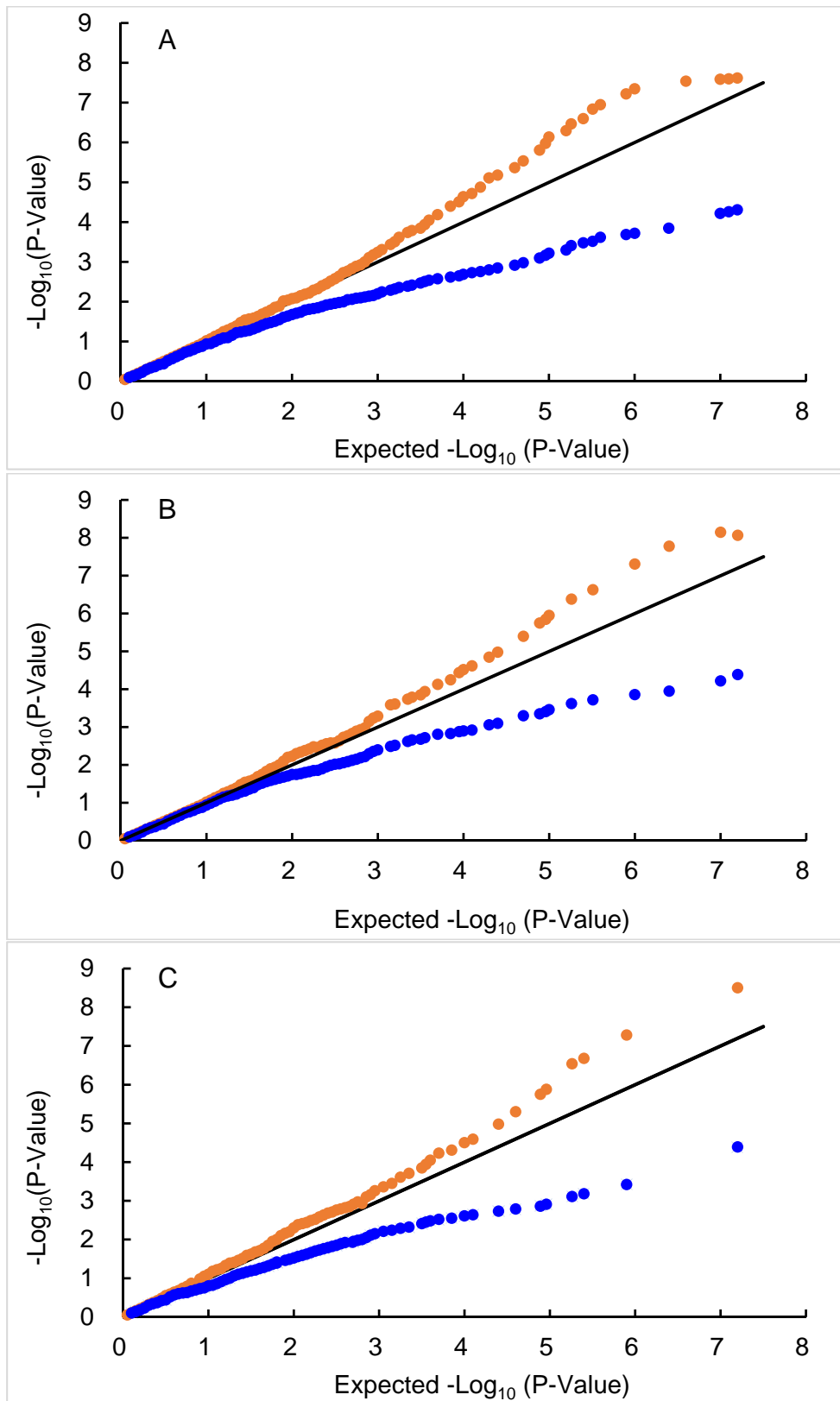
Figure S2 | Quantile-quantile plots of the GLM and MLM from association mapping in the whole panel (A), melo group (B), and agrestis group (C). ● GLM; ● MLM
