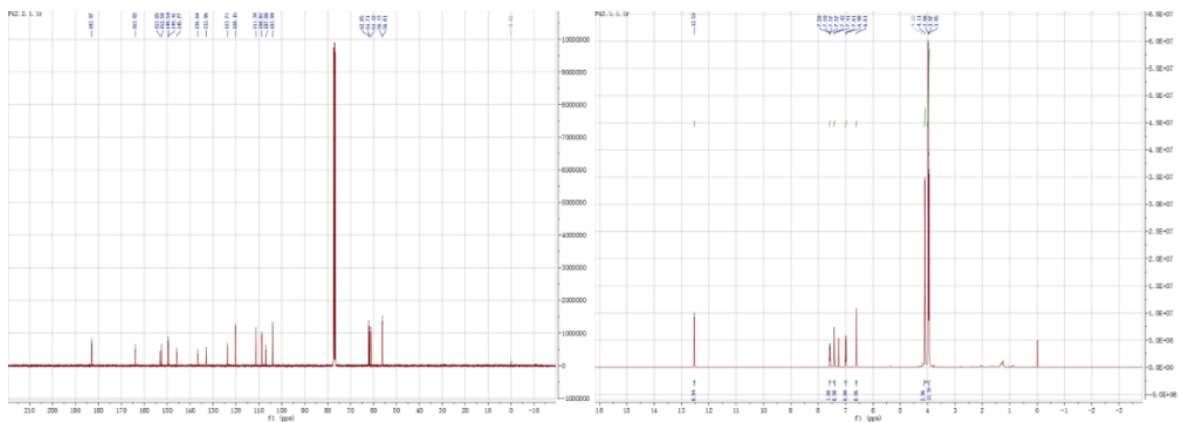
Figure S5. ^{13}\text{C} - and ^1\text{H} -NMR spectrum of 5-hydroxy-6,7,8,3',4'-pentamethoxyflavone.
