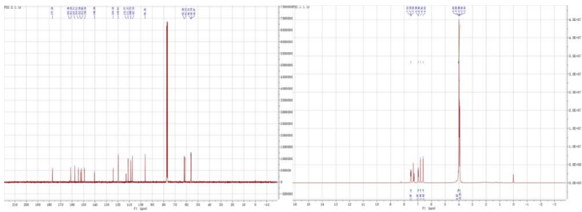
Figure S4. ^{13}\text{C} - and ^1\text{H} -NMR spectrum of sinensetin.
