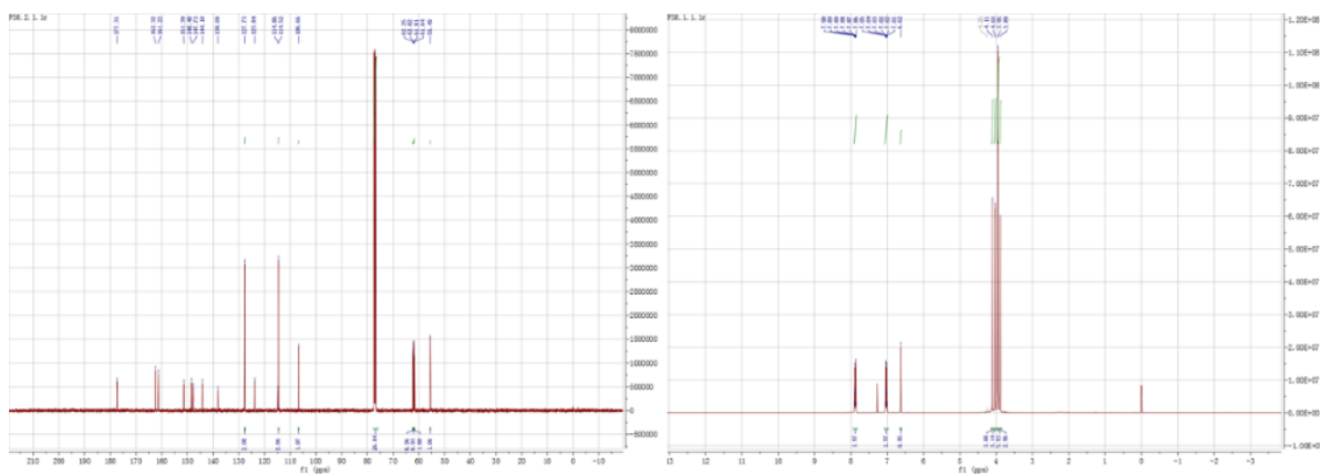
Figure S3. ^{13}\text{C} - and ^1\text{H} -NMR spectrum of tangeretin.
