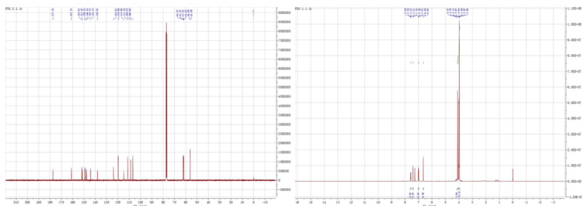
Figure S2. ^{13}\text{C} - and ^1\text{H} -NMR spectrum of nobiletin.
