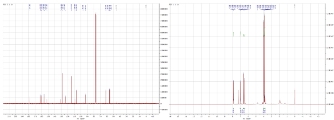
Figure S1. ^{13}\text{C} - and ^1\text{H} -NMR spectrum of 5,6,7,4'-tetramethoxyflavone.
