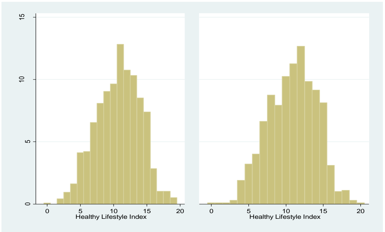
Supplementary Figure 1. Distribution of HLIS for longitudinal cohort (n=1401) at baseline (left) and follow-up (right).
