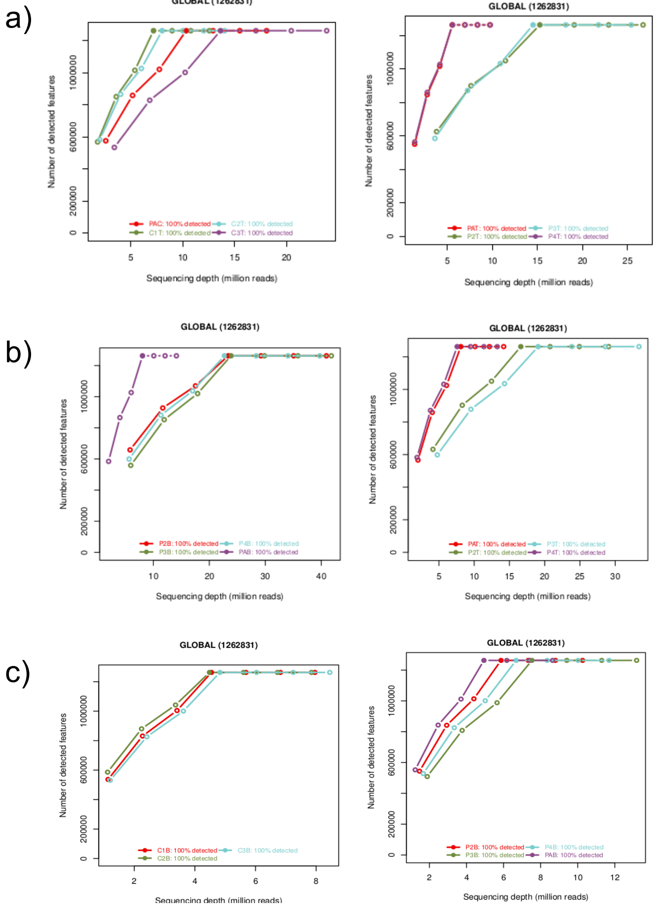
Supplementary Figure 6. Sequencing depth and quantification of expression. QC plots for sequencing depth in the NOISEq package. Graphs show the number of detected genes at the given sequencing depth. a) Control tumor vs. tumor sites. b) Tumor adjacent vs. tumor sites c) Tumor adjacent vs. buccal sites from healthy controls.
