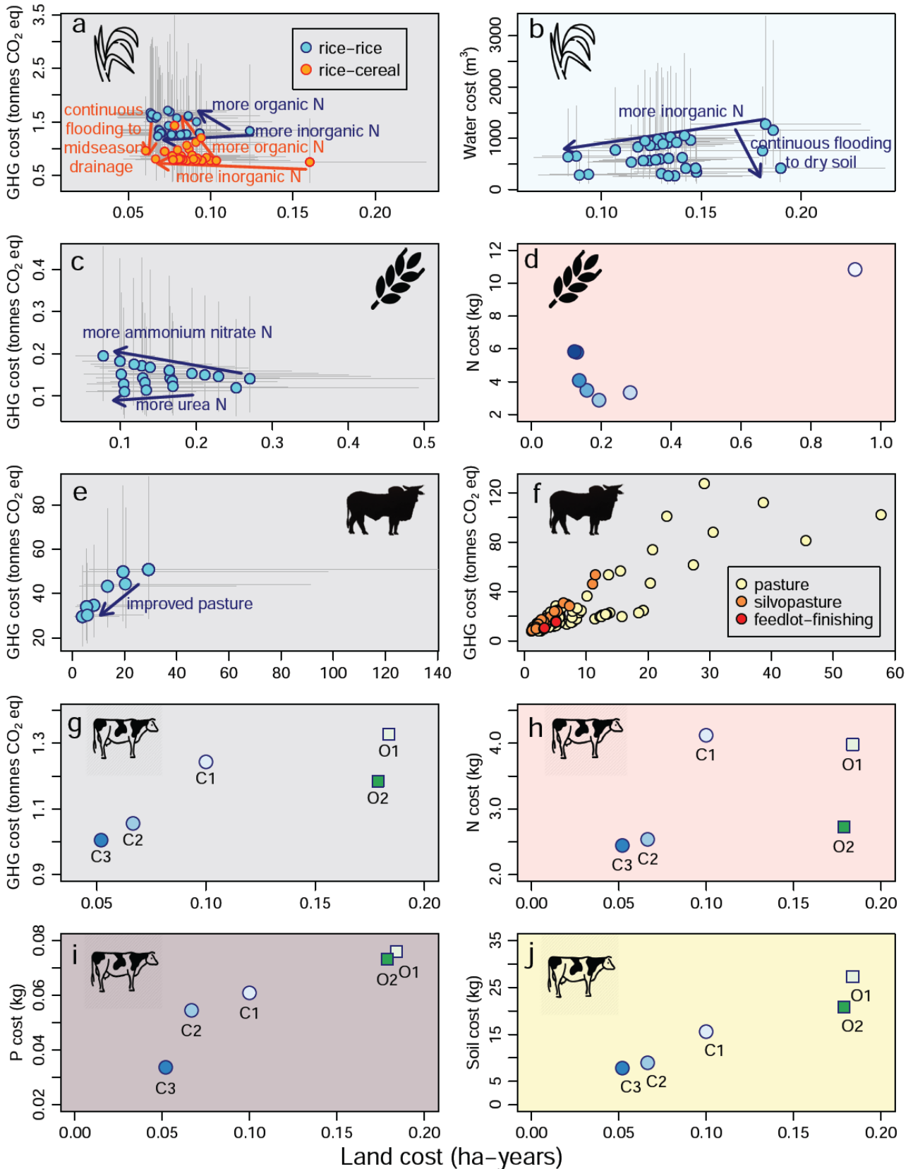
Supplementary Figure 1. Externality costs of alternative production systems against land cost for five externalities in four agricultural sectors, showing uncertainty for statistically derived estimates. Plots are modified versions of those in Fig. 2, with pale grey lines in a, b, c and e representing 95% confidence intervals around our GLMM-derived predictions. All other notation as in Fig. 2.
