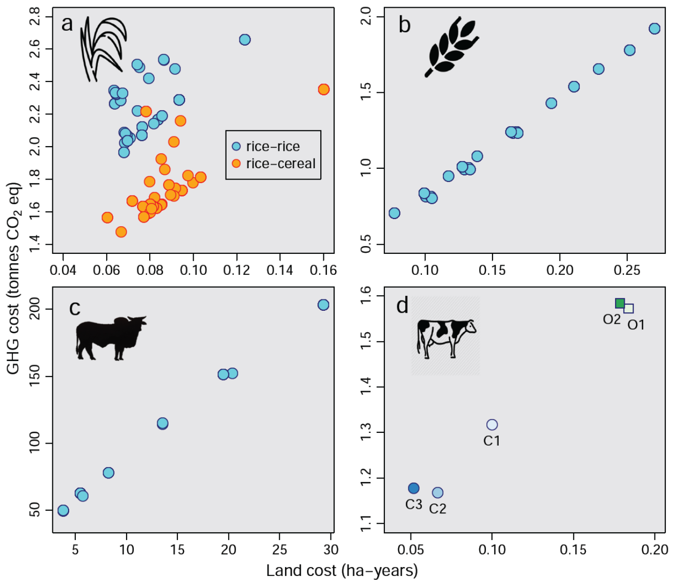
Supplementary Figure 3. Sensitivity tests of associations between overall GHG costs (including GHG opportunity costs of land use) and land costs. Plots are modified versions of those in Fig. 3, but show the effects of assuming either that carbon sequestration rates of recovering habitat are half those given in IPCC guidelines or that half of the area potentially freed from farming because of higher yield is retained under agriculture (Methods); these assumptions have identical effects. Notation as in Fig. 3. Spearman's rank correlation coefficients ( \rho values) are a. rice-rice: 0.07 (0.69), rice-cereal: 0.66 ( < 0.001 ), b. 0.97 ( < 0.001 ), c. 0.98 ( < 0.001 ) and d. 0.80 (0.13).
