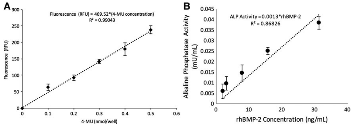
SUPPLEMENTARY FIG. S1. (A) Fluorescence activity as a function of substrate concentration for a constant amount of alkaline phosphatase enzyme. (B) Alkaline phosphatase activity (mU/mL) as a function of rhBMP-2 concentration and used for Figure 2B. Error bars indicate standard error of the mean ( n=3 ). rhBMP-2, recombinant human bone morphogenetic protein 2.
