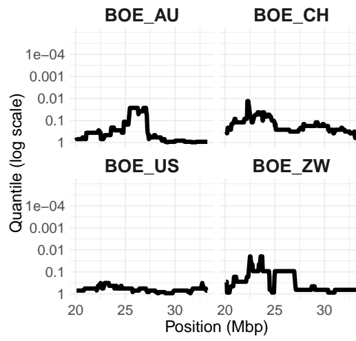
ROH
