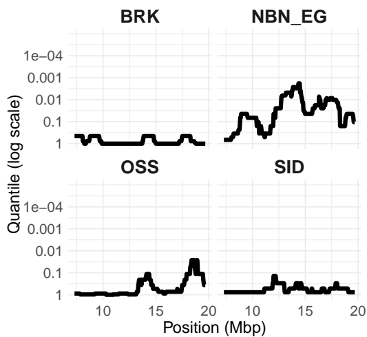
ROH
