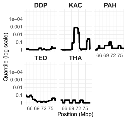
ROH
