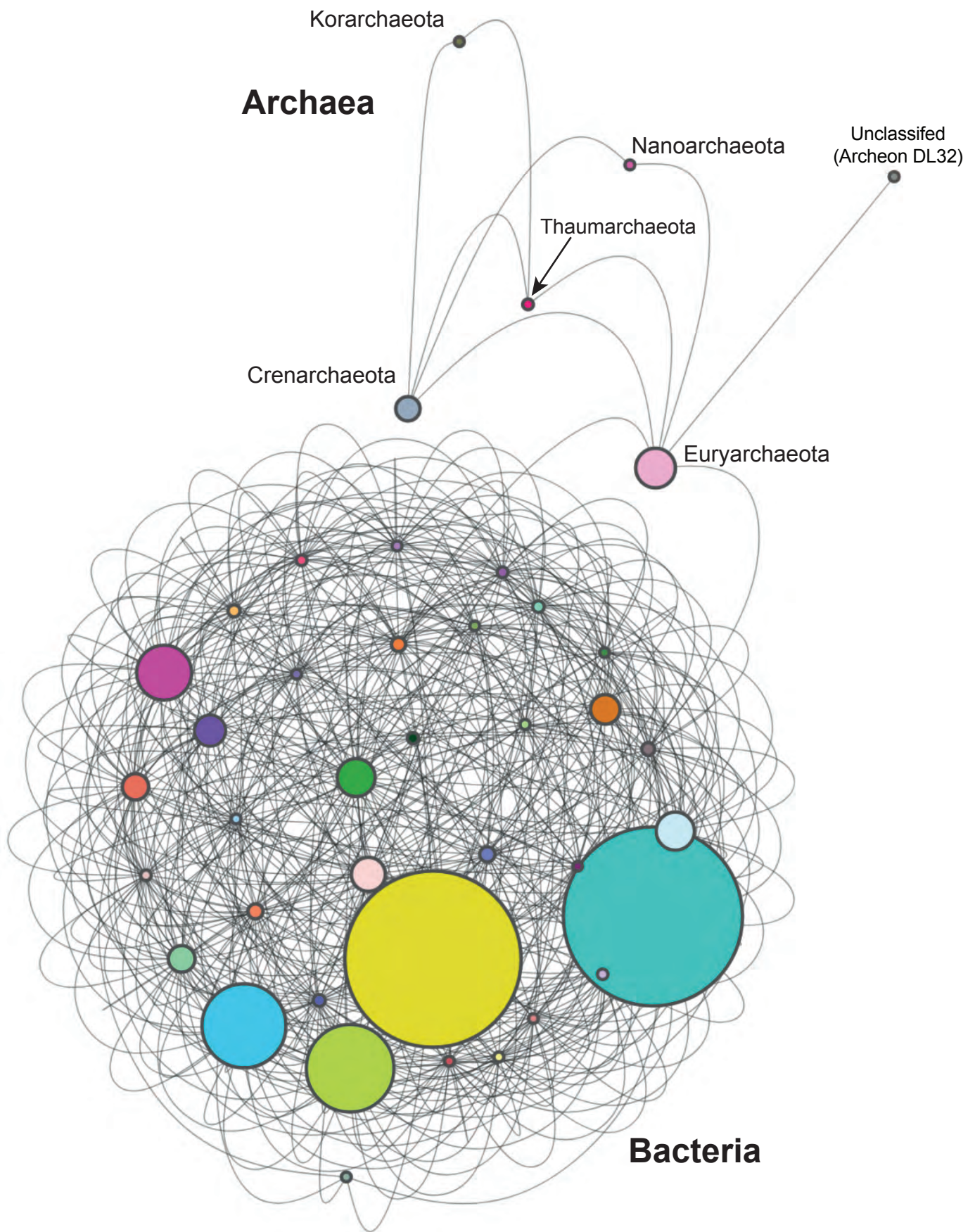
Figure S2. P -network of 2616 prokaryote genomes using D_2^S with k = 25 based on rRNA genes only, at t = 6 . An edge between two nodes represents one or more connections between isolates from the two phyla. Archaeal phyla (labelled) are clearly separated from bacterial phyla.
