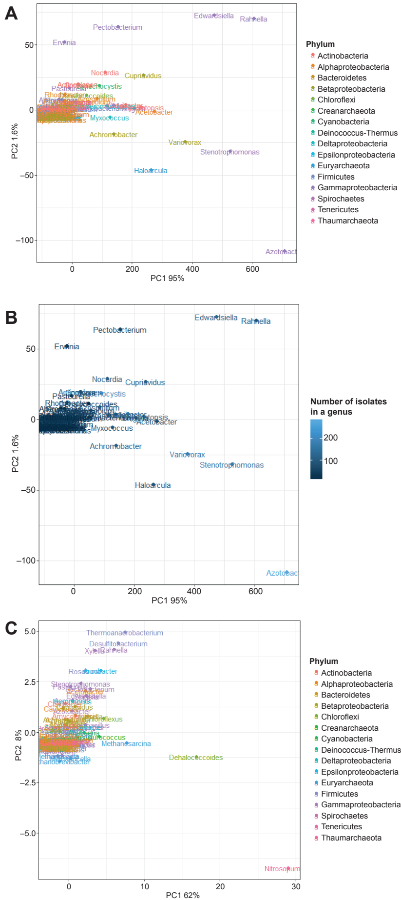
Figure S4. Principal component analysis (PCA) of core k -mers and their annotated COG categories, based on core k -mers in each (A) phylum and (B) genus. The PCA of core k -mers in each phylum performed on the normalised counts of COG categories in centred scale is shown in (C).
