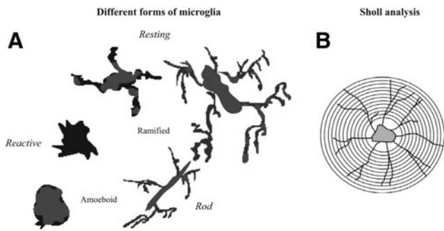
SUPPLEMENTARY FIG. S3. (A) Schematic illustration of microglia in different forms from resting to reactive. (B) Schematic illustration of the Sholl analysis of microglia/macrophages used in the present study.
