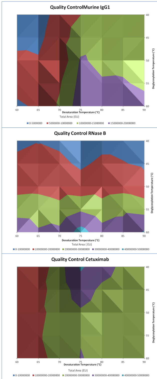
Supplementary Figure 2:
