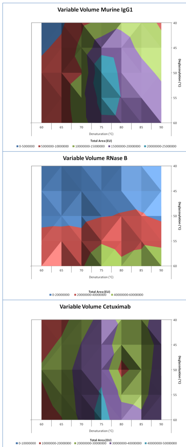
Supplementary Figure 1:
