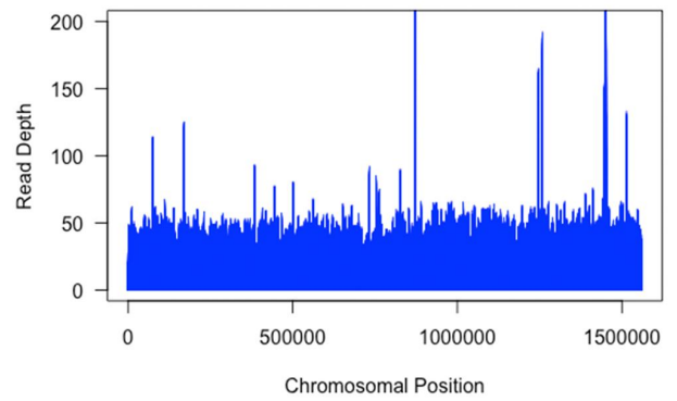
VL38 - chr32
