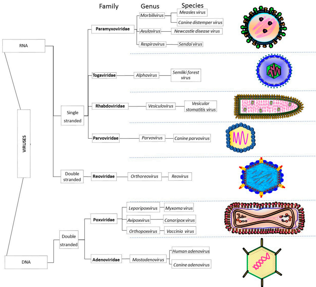
Supplementary Figure S1. Oncolytic viruses studied in dogs. The figure shows the different viruses that have been studied as oncolytics either in vitro or in vivo in dogs. Viruses are grouped according to their genus, family and type of nucleic acid. Representative virion structures for each viral family are shown.
