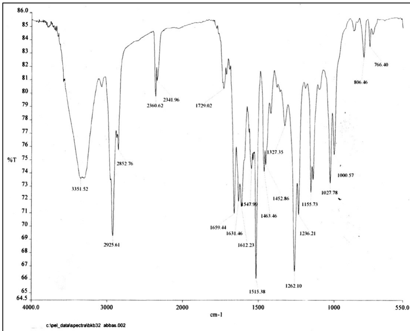
Figure 1S. IR spectrum of (-)-kunstleramide (1).
