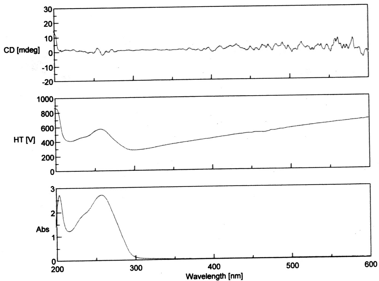
Figure 2S. CD spectrum of (-)- kunstleramide (1).
