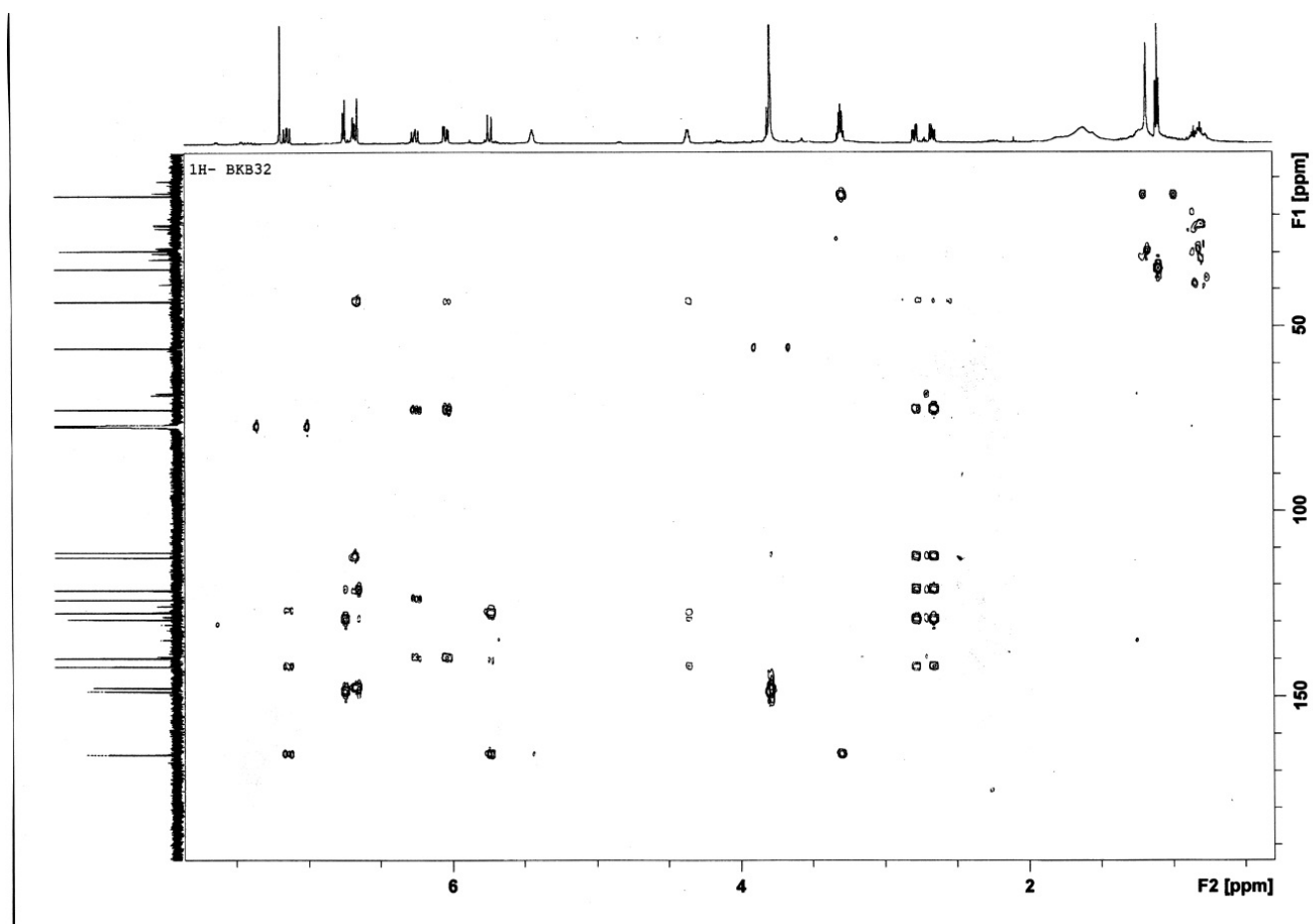
Figure 10S. HMBC spectrum of (-)-kunstleramide (1).
