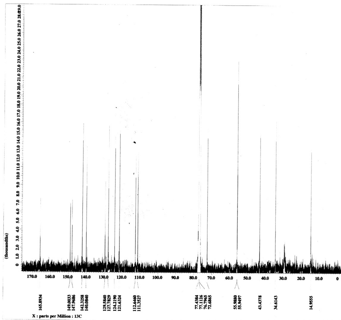
Figure 5S. ^{13}\text{C} -NMR spectrum of (-)- kunstleramide (1).
