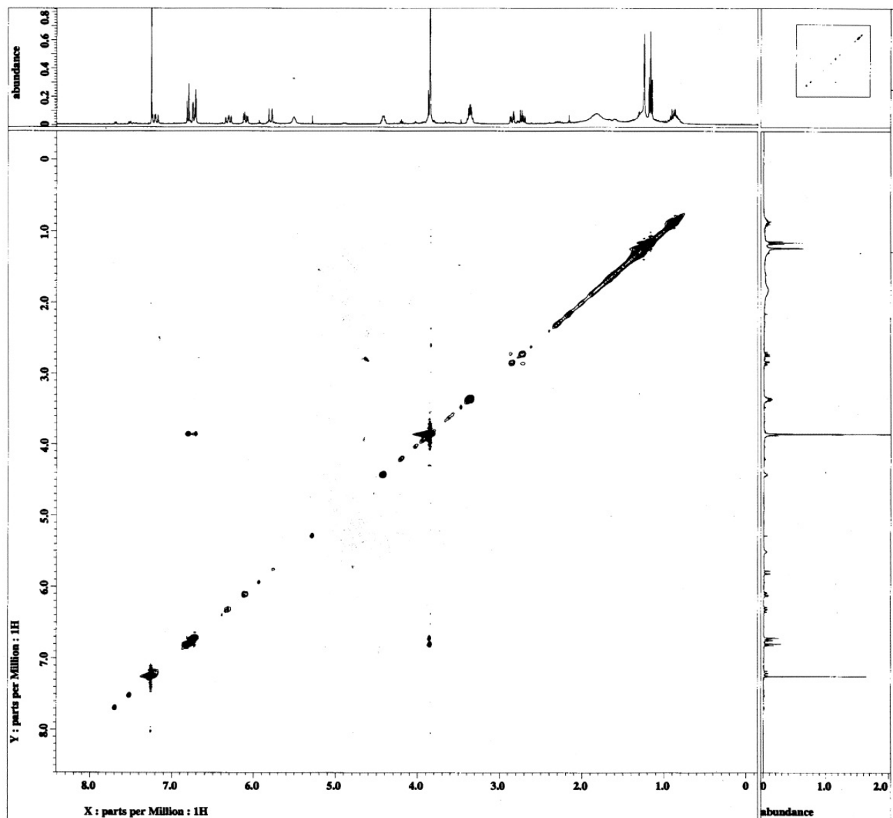
Figure 8S. NOESY spectrum of (-)-kustleramide (1).
