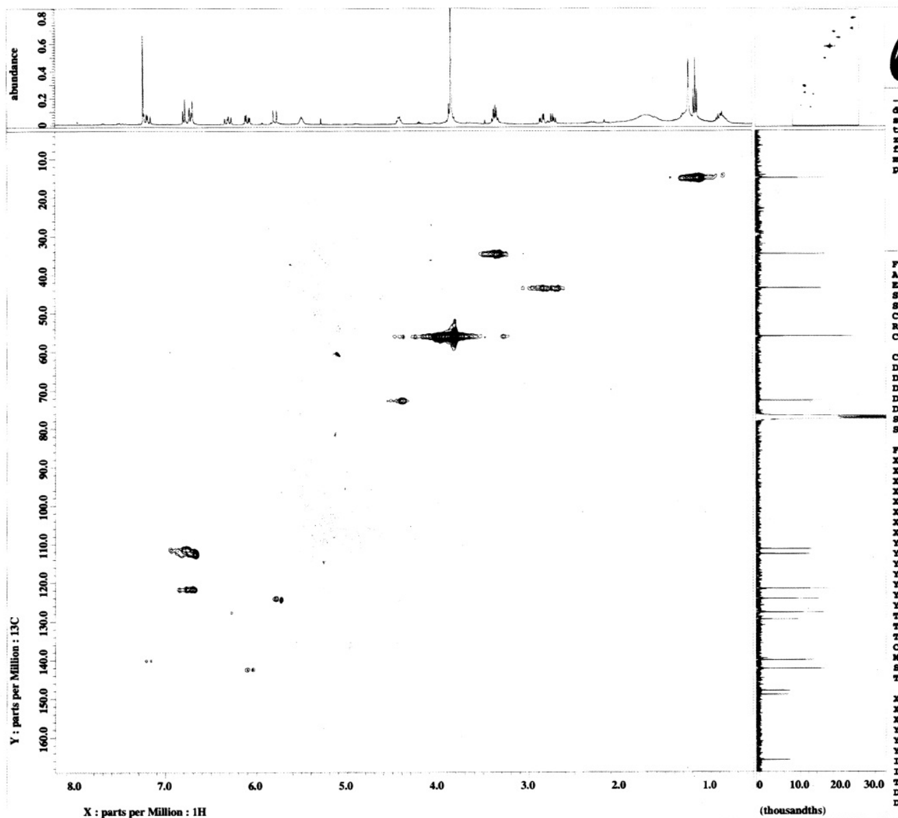
Figure 9S. HMQC spectrum of (-)-kunstleramide (1).
