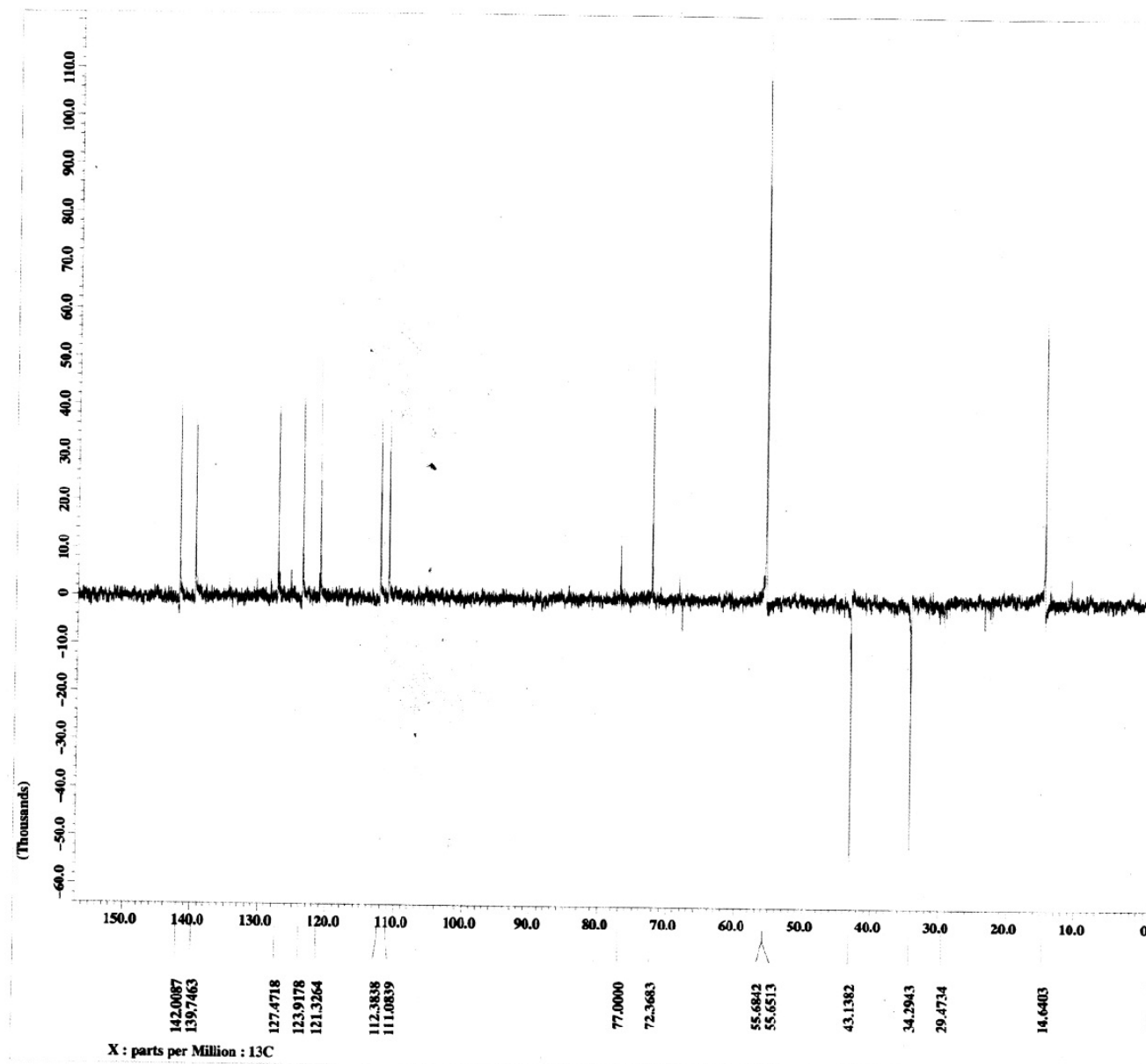
Figure 6S. DEPT of (-)-kunstleramide (1).
