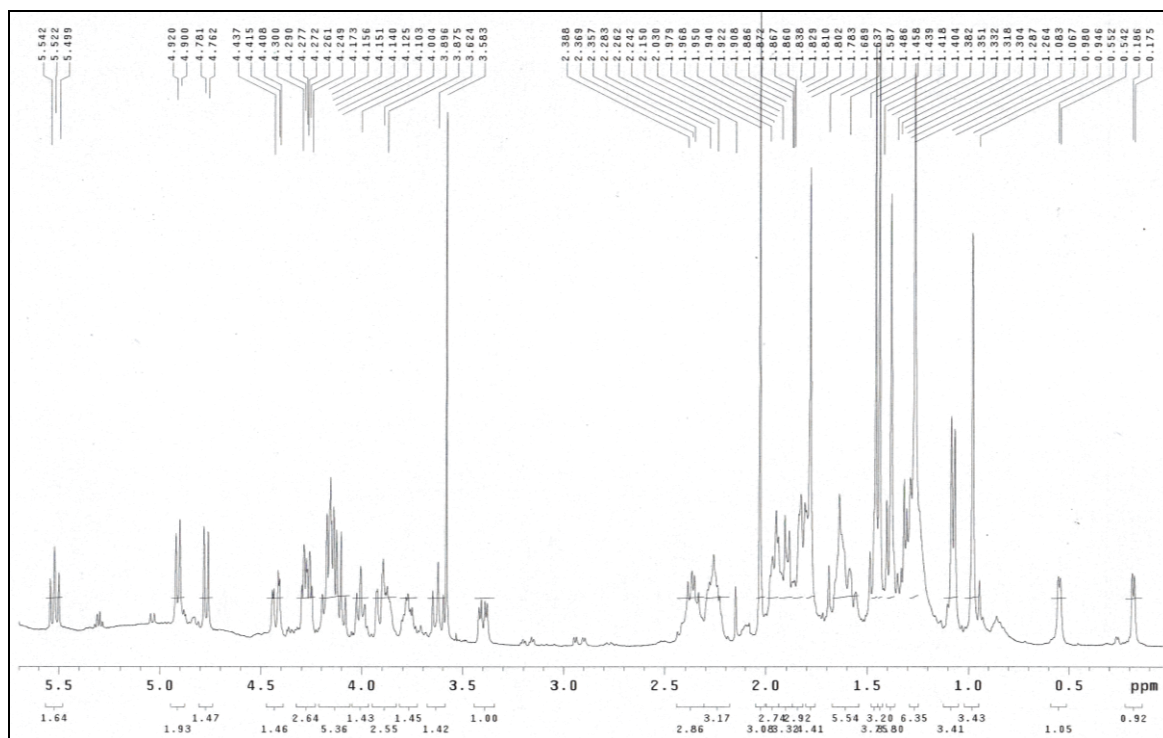
Figure S2. ^{13}\text{C-NMR} of compound 1 .
