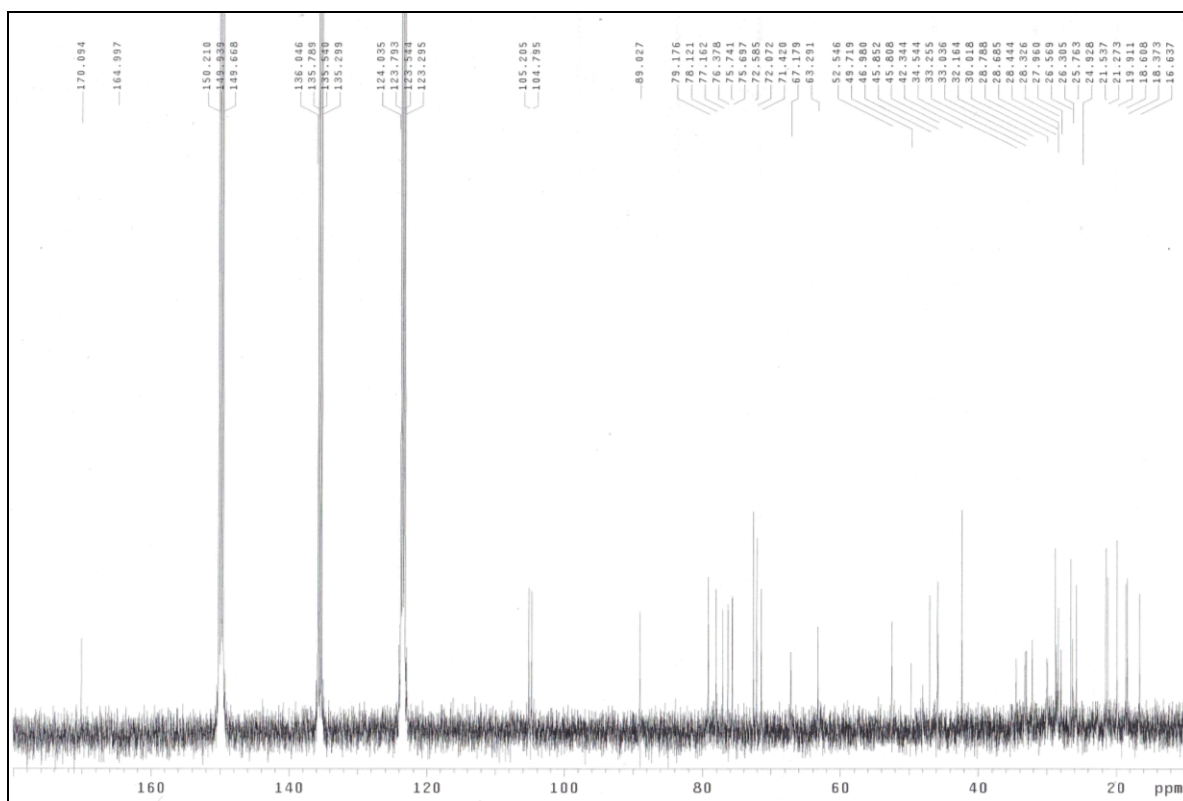
Figure S2. ^{13}\text{C-NMR} of compound 1 .
