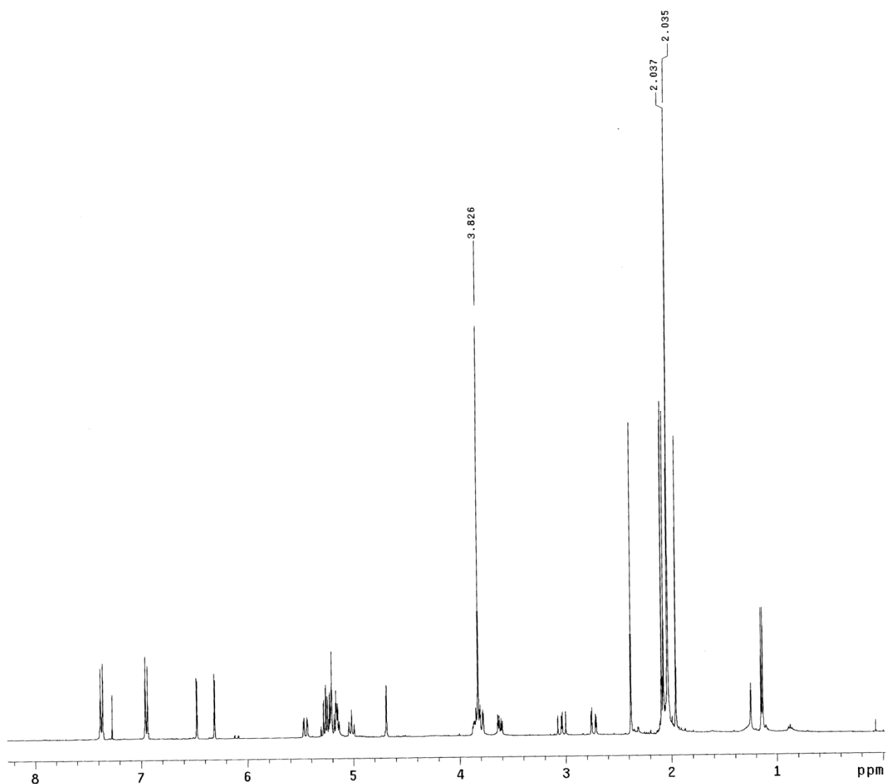
Figure S2. ^1\text{H-NMR} ( \text{CDCl}_3 , 400MHz) compound 2a.
