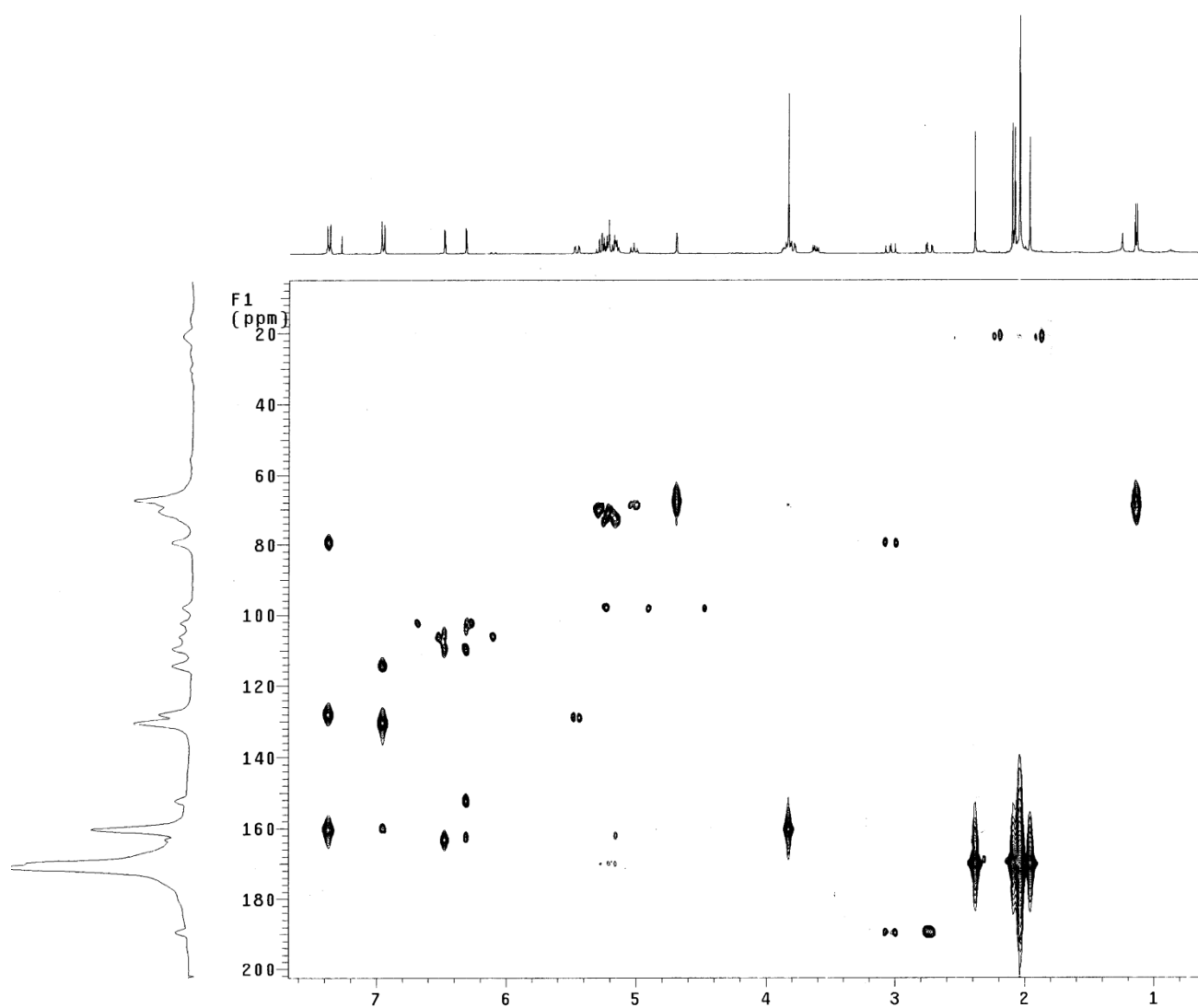
Figure S6. HMBC (CDCl 3 , 400MHz) compound 2a.
