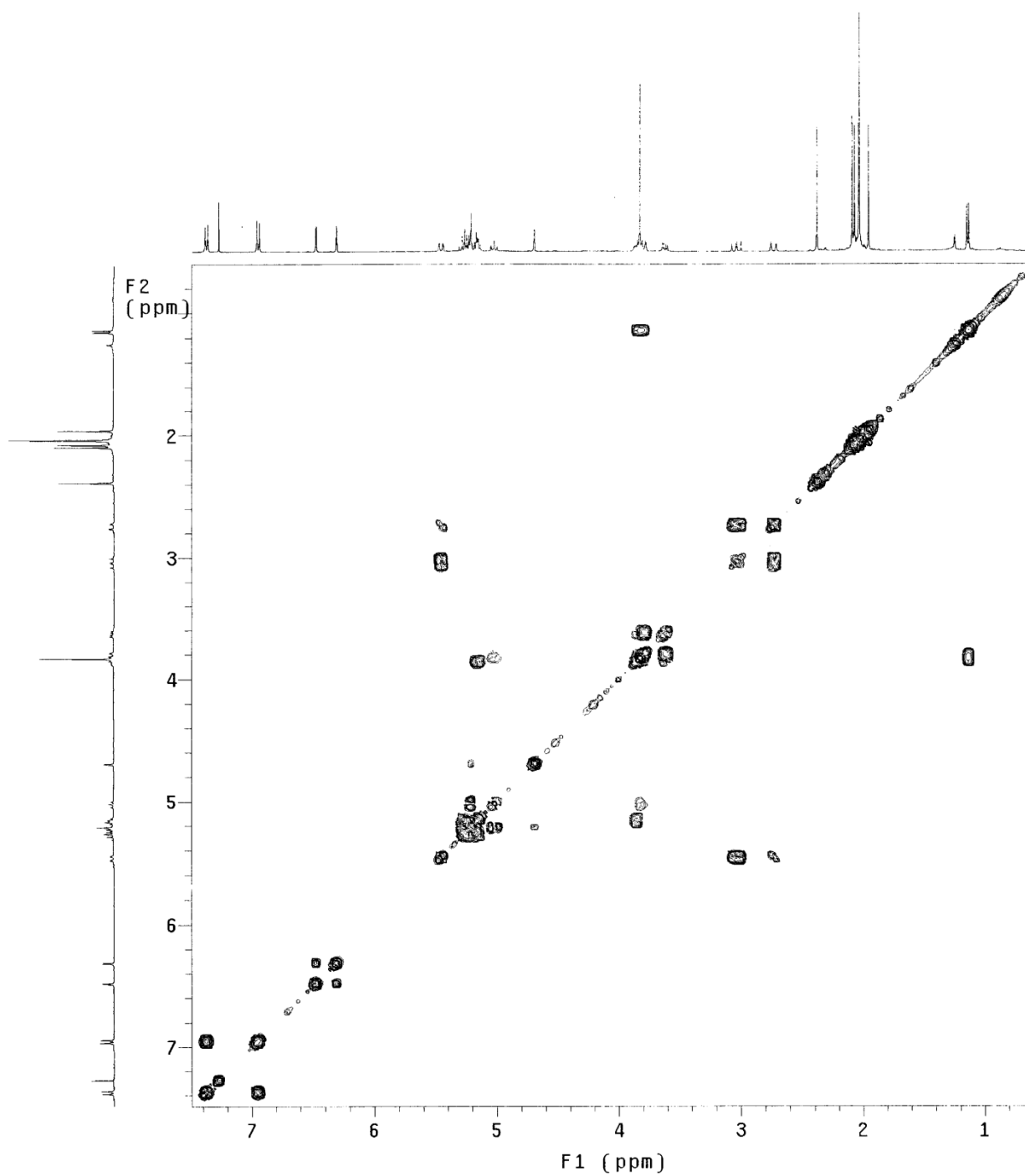
Figure S4. ^1\text{H} - ^1\text{H} COSY ( \text{CDCl}_3 , 400MHz) compound 2a.
