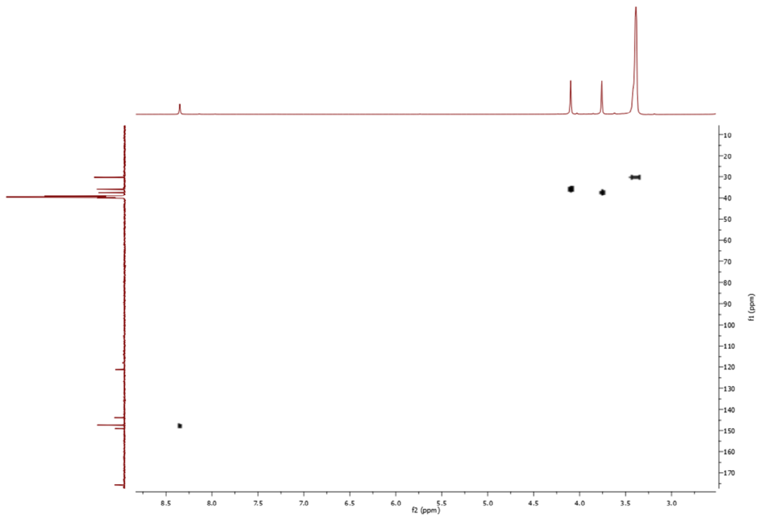
Figure S3. HSQC spectrum of 6-selenocaffeine, recorded in DMSO-d 6 .
