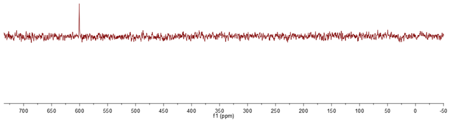
Figure S4. ^{77}\text{Se} -NMR spectrum of 6-selenocaffeine, recorded in DMSO- d_6 .
