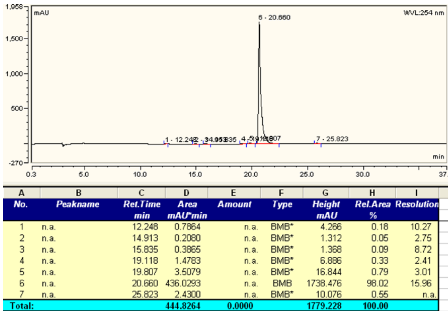
Figure S6. HPLC-DAD chromatogram of 6-selenocaffeine.
