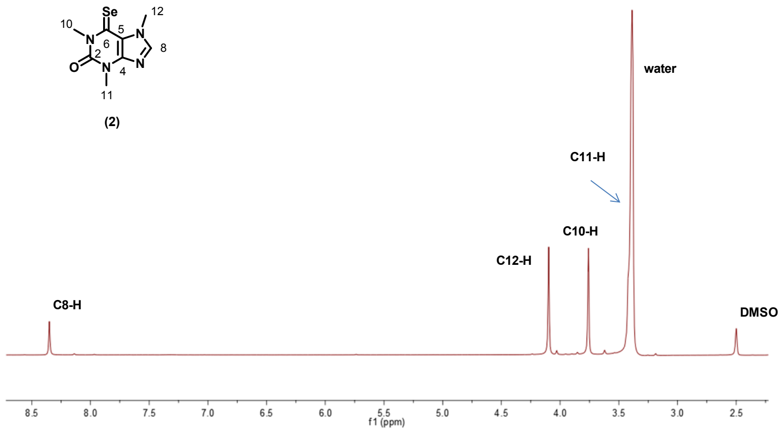
Figure S1. ^1\text{H} -NMR spectrum of 6-selenocaffeine, recorded in \text{DMSO-d}_6 .
