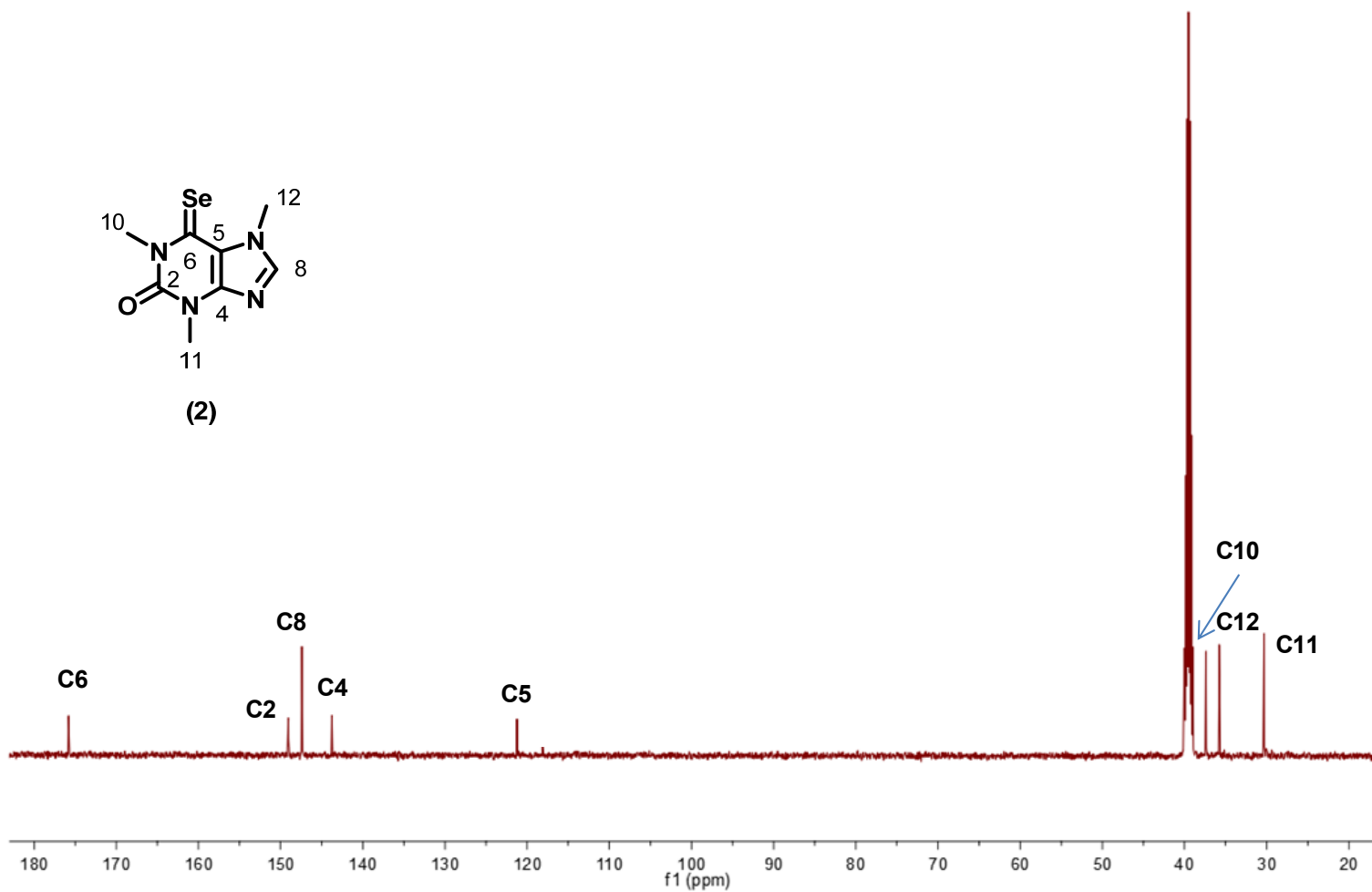
Figure S2. ^{13}\text{C} -NMR spectrum of 6-selenocaffeine, recorded in \text{DMSO-d}_6 .
