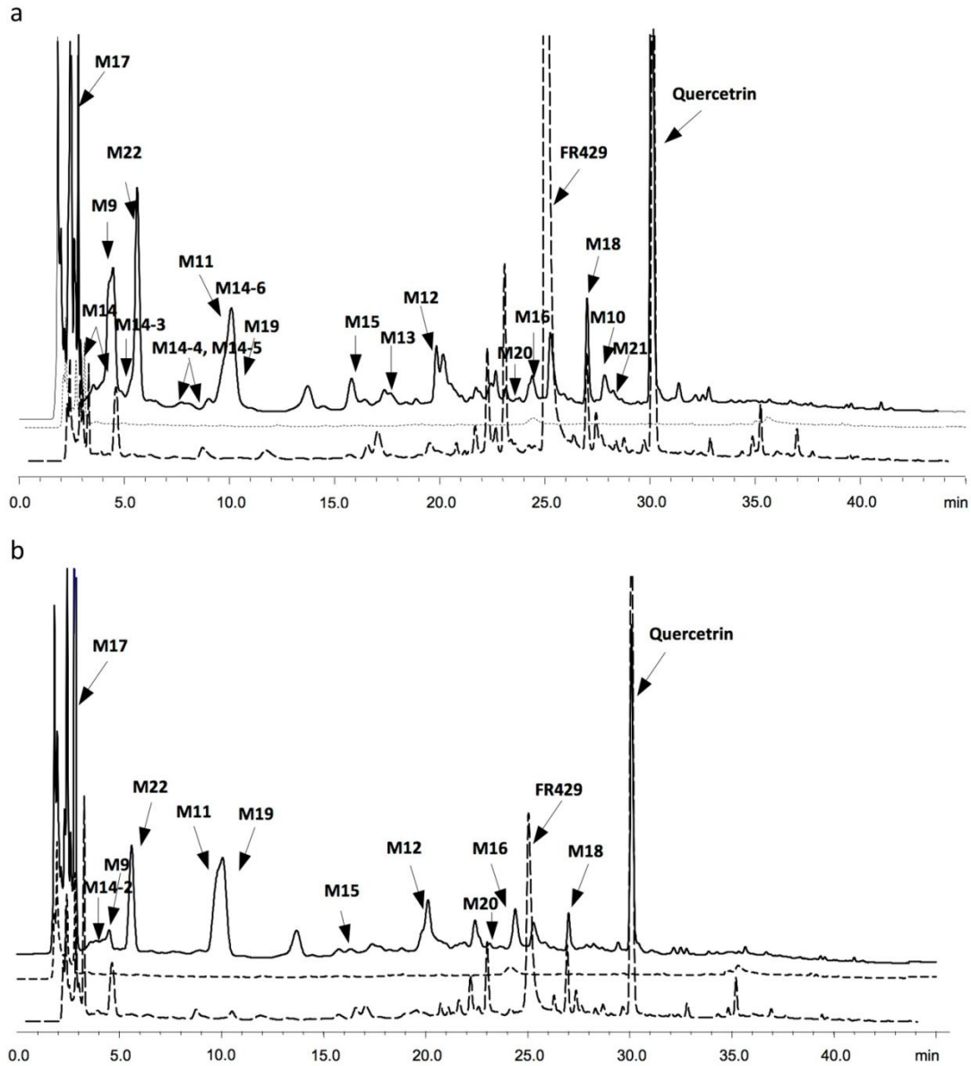
Figure S1. HPLC chromatogram of metabolites in the incubation of extracts of P. capitatum in the intestinal bacteria in vitro (a) HPLC of metabolites of EtOAc fraction; (b): HPLC of metabolites of ethanol extracts; —: incubation for 24 h; ----: negative control for 24 h; - - - -: incubation for 0 h.
