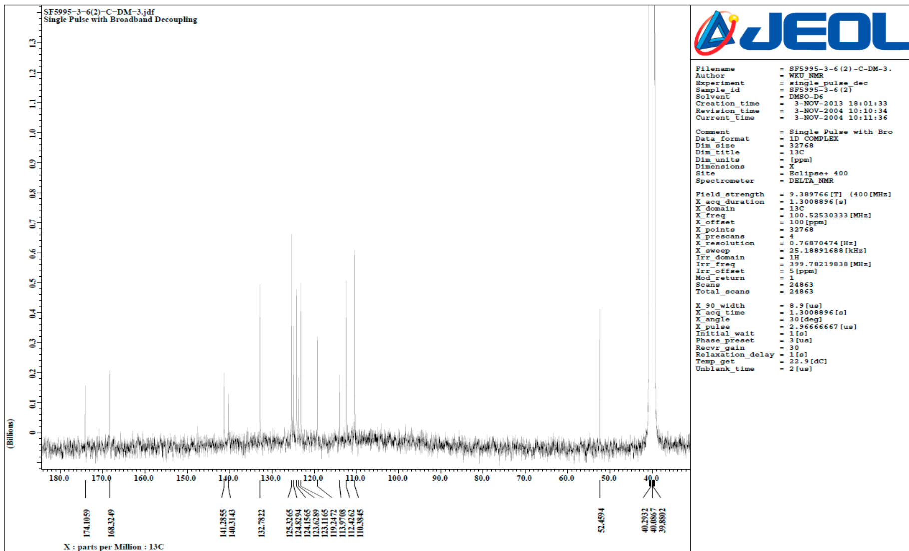
Figure S2. ^{13}\text{C} -NMR spectrum of compound 1 at 100 MHz in \text{CD}_3\text{OD}-d_6 .
