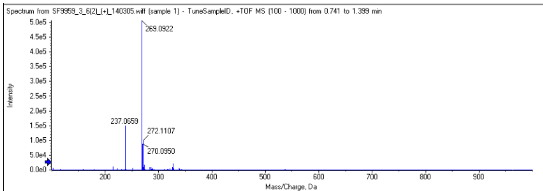
Figure S3. HR-ESIMS of compound 1.
