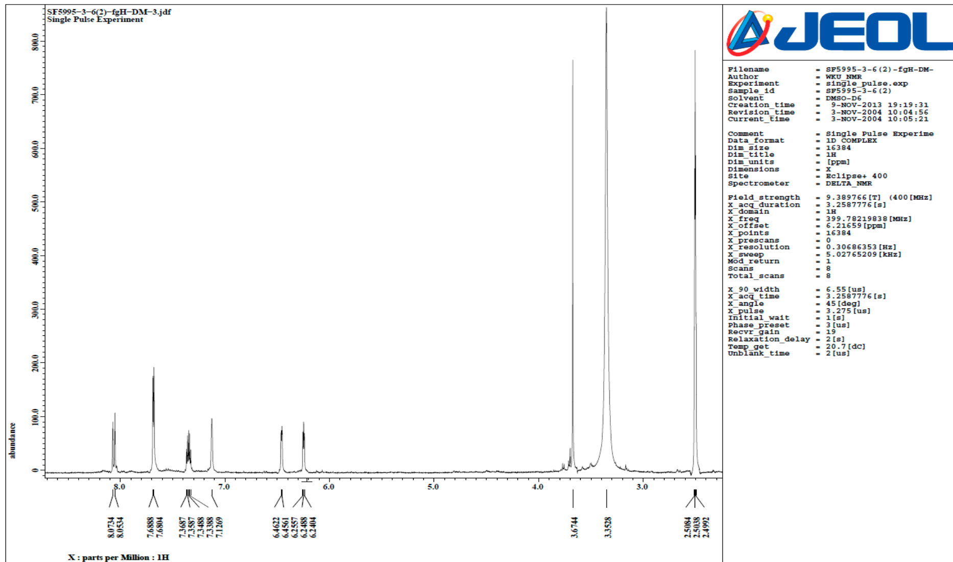
Figure S1. ^1\text{H} -NMR spectrum of compound 1 at 400 MHz in \text{CD}_3\text{OD}-d_6 .
