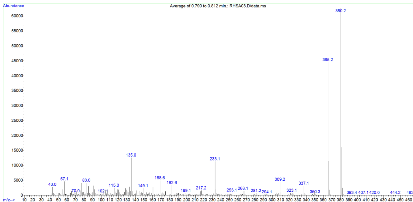
Figure S5. EIMS spectrum of 5c.
