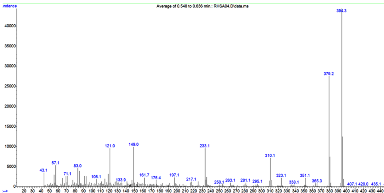
Figure S5. EIMS spectrum of 5c.
