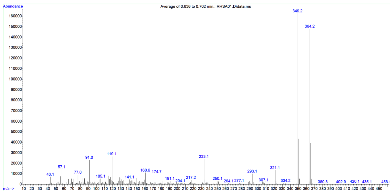
Figure S3. EIMS spectrum of 5a .
