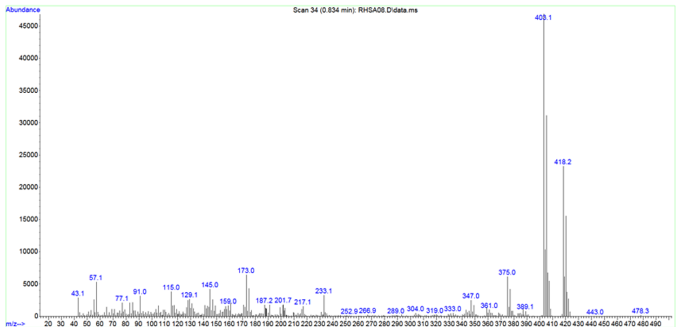
Figure S7. EIMS spectrum of 5h.
