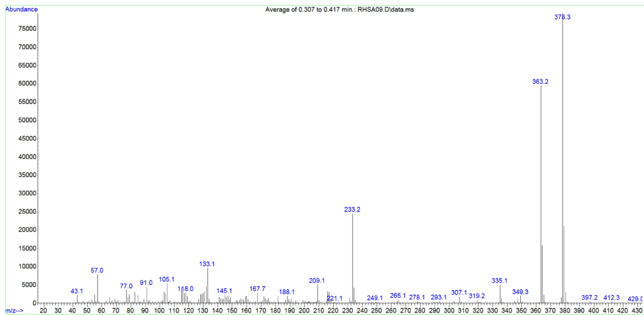
Figure S8. EIMS spectrum of 5i .
