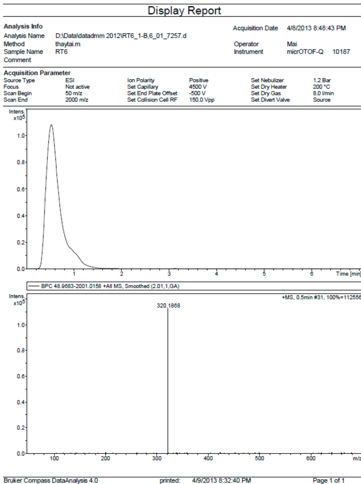
Figure S7. HRESIMS of compound 1.
