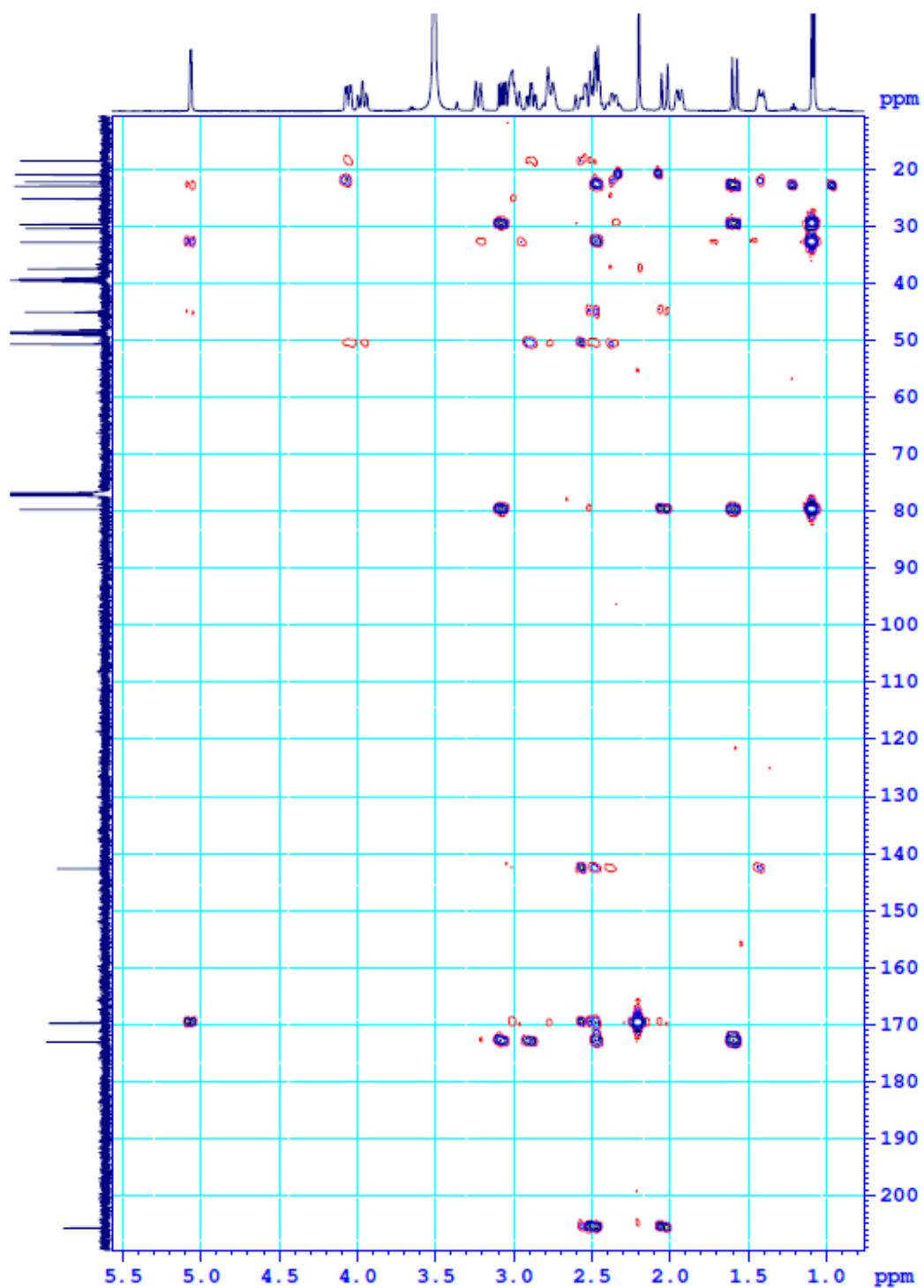
Figure S4. HMBC spectrum of compound 1.
