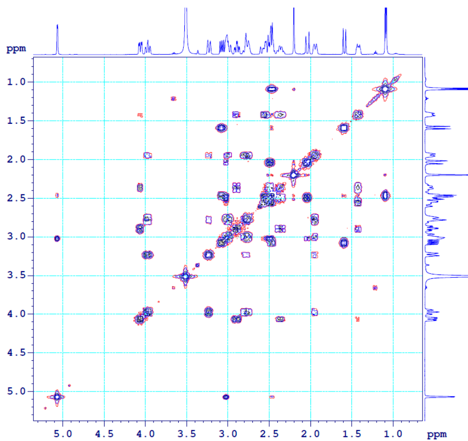
Figure S6. ROESY spectrum of compound 1.
