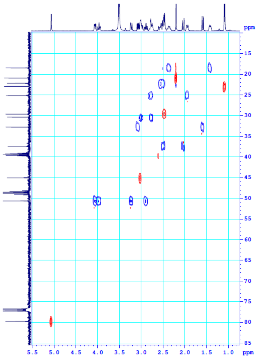
Figure S3. HMQC spectrum of compound 1.
