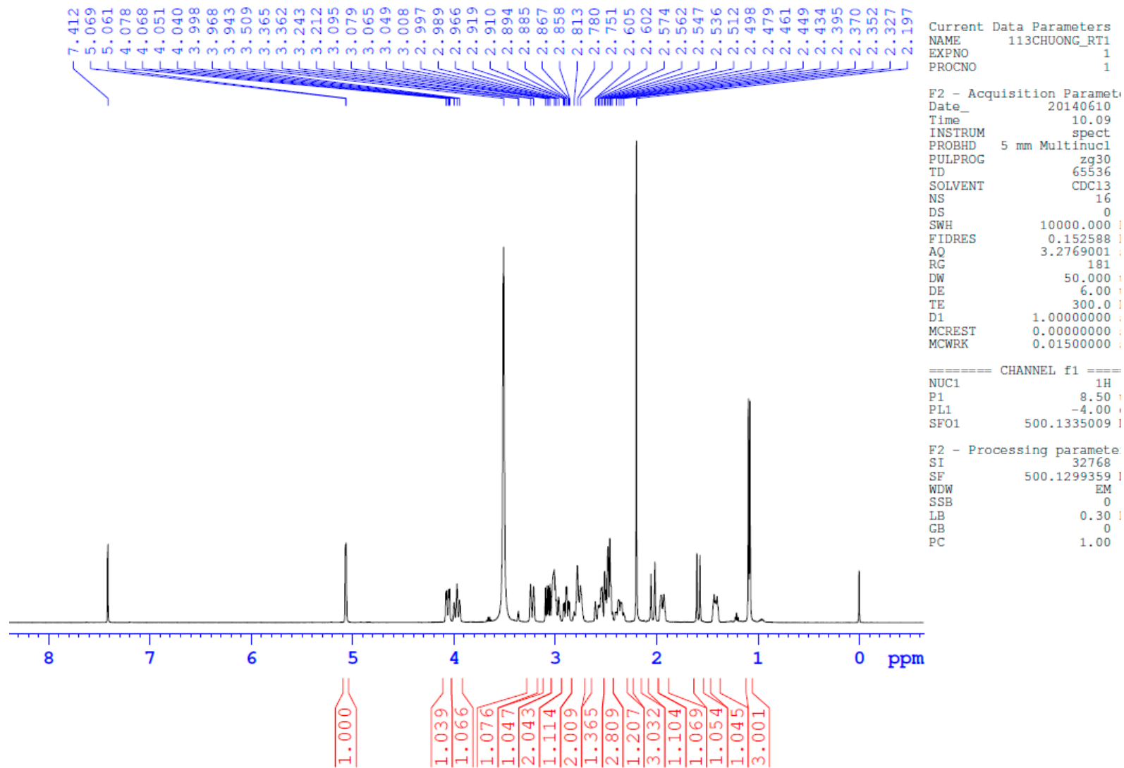
Figure S1. 1 H-NMR spectrum of compound 1.
