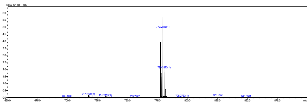
Figure S10. ^1\text{H} -NMR spectra of 7d.
