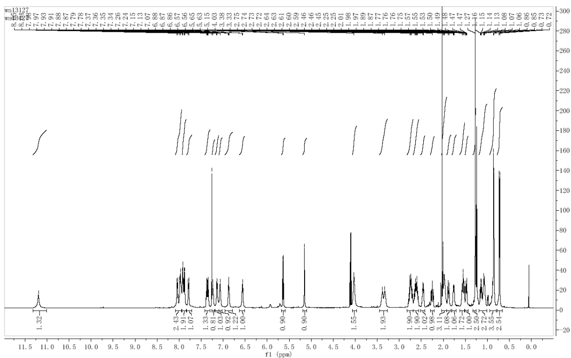
Figure S19. ^1\text{H} -NMR spectra of 8.
