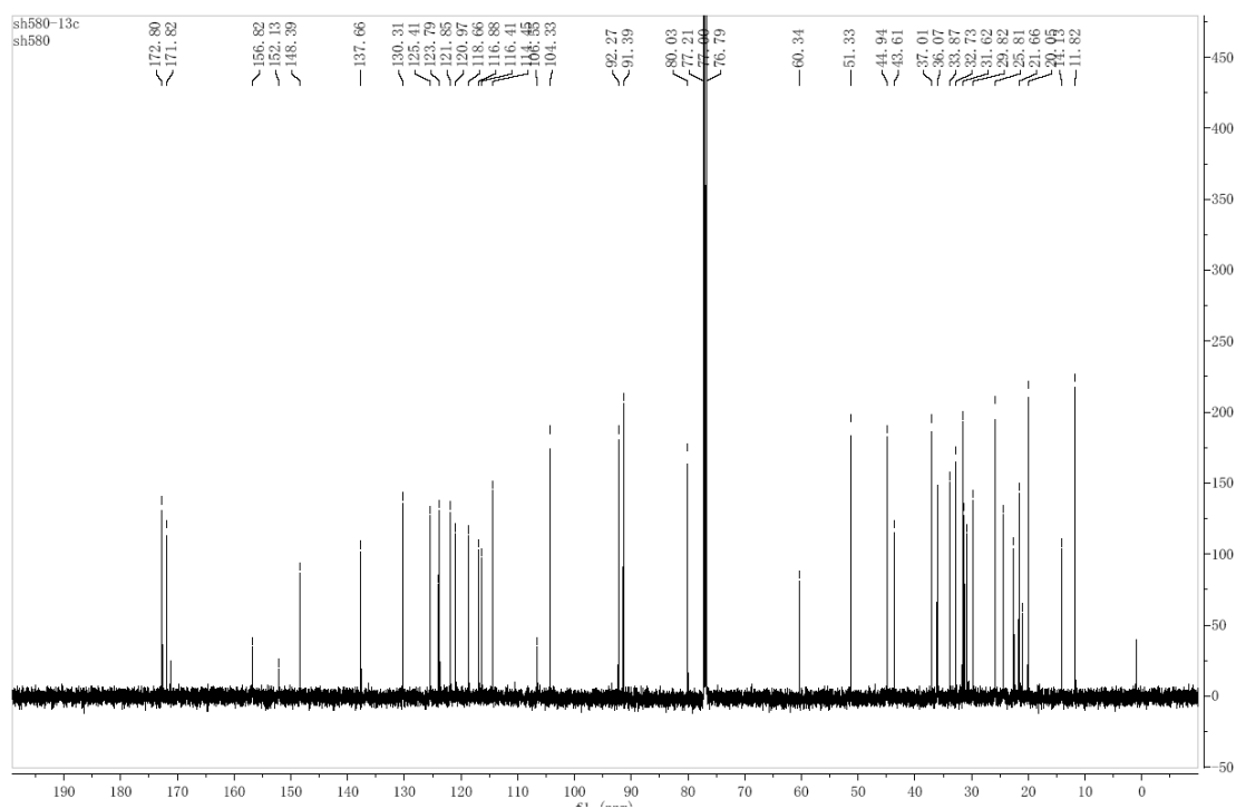
Figure S2. ^{13}\text{C-NMR} spectra of 7a.
