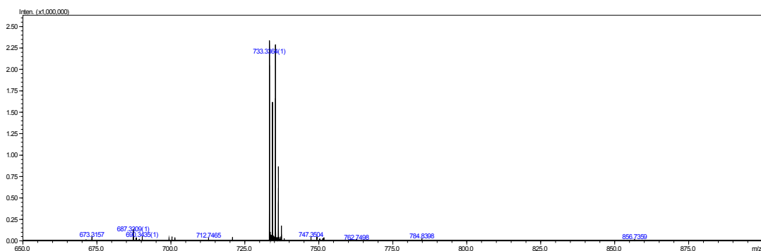
Figure S7. ^1\text{H} -NMR spectra of 7c.
