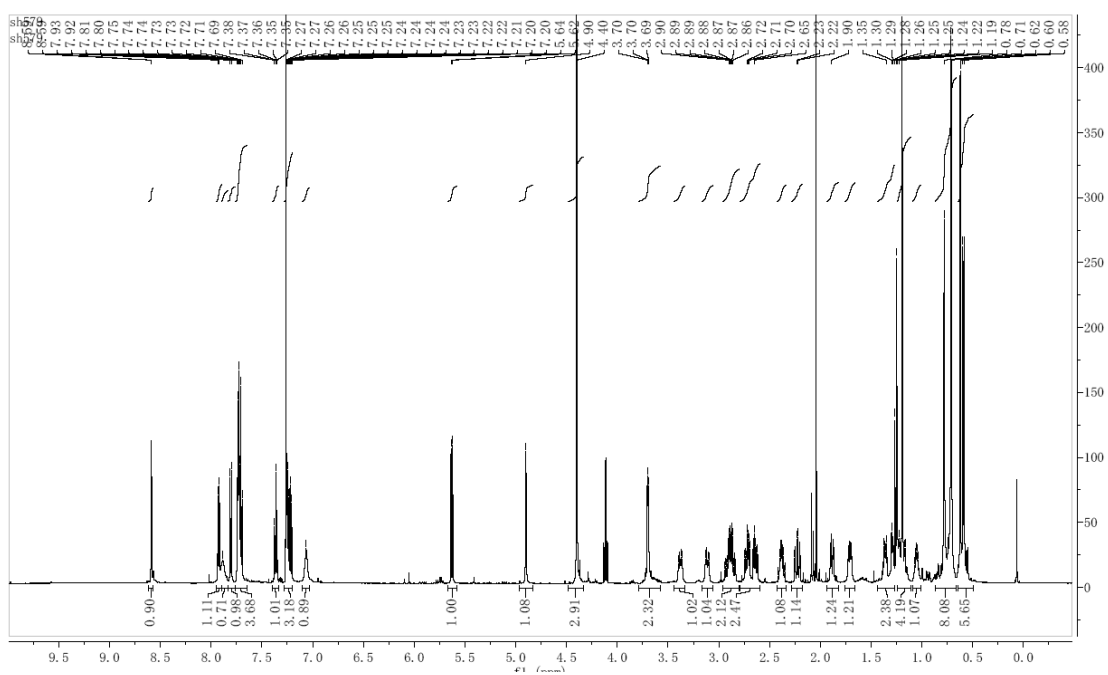
Figure S4. ^1\text{H-NMR} spectra of 7b.
