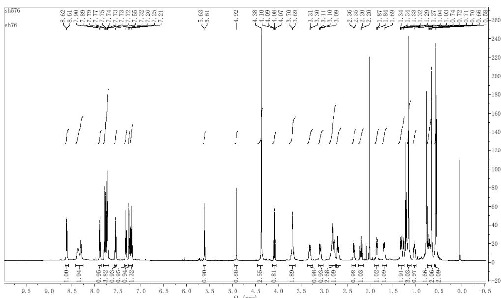
Figure S7. ^1\text{H} -NMR spectra of 7c.
