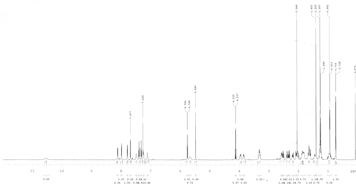
Figure S22. ^1\text{H} -NMR spectra of 9.
