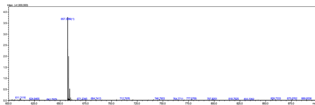
Figure S22. ^1\text{H} -NMR spectra of 9.
