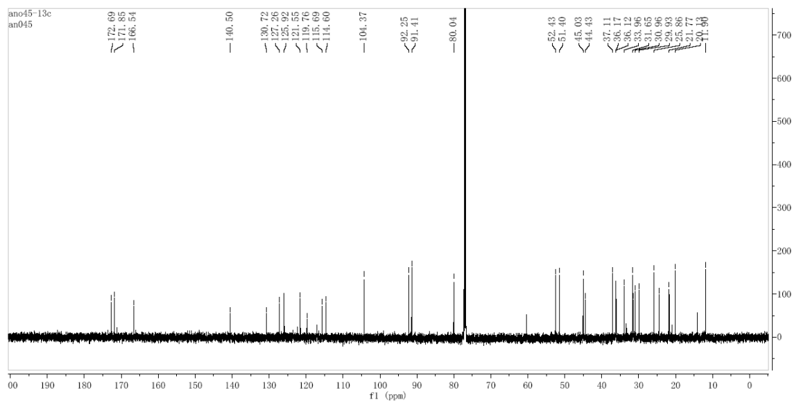
Figure S12. HRMS of 7c.
