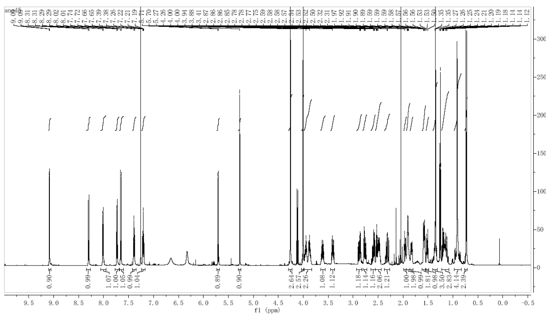
Figure S10. ^1\text{H} -NMR spectra of 7d.
