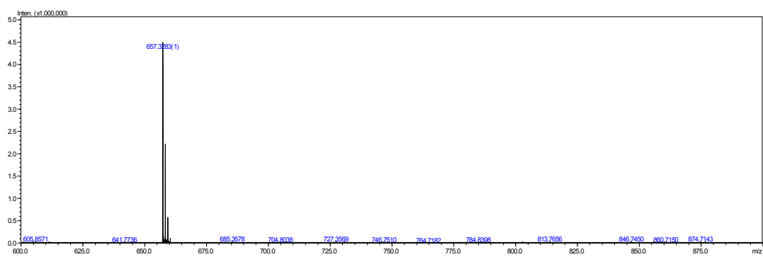
Figure S24. HRMS of 9.
