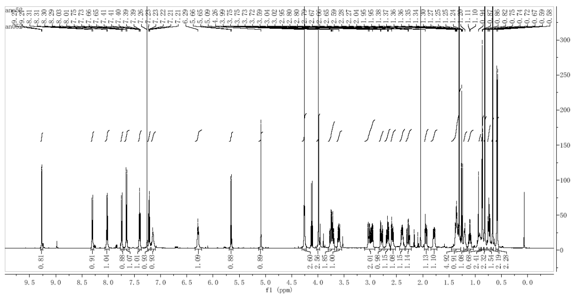
Figure S13. ^1\text{H} -NMR spectra of 7e.
