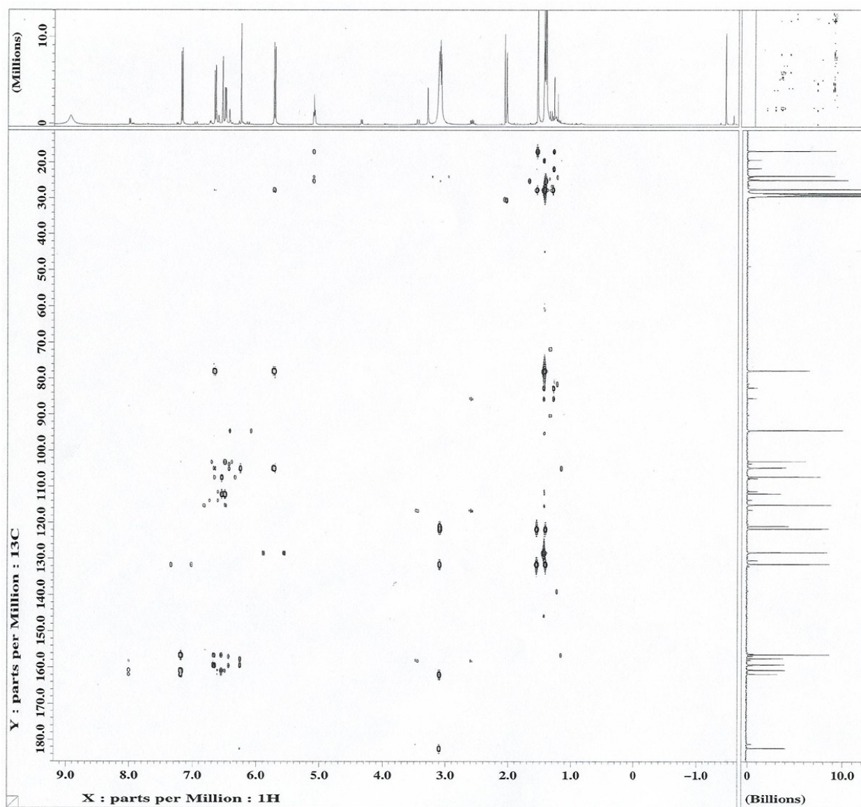
Figure S5. HMBC data of cudarflavone B.
