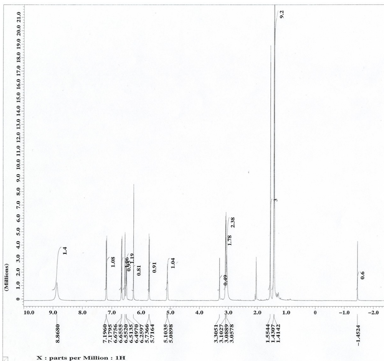
Figure S1. ^1\text{H} -NMR spectrum of cudarflavone B.
