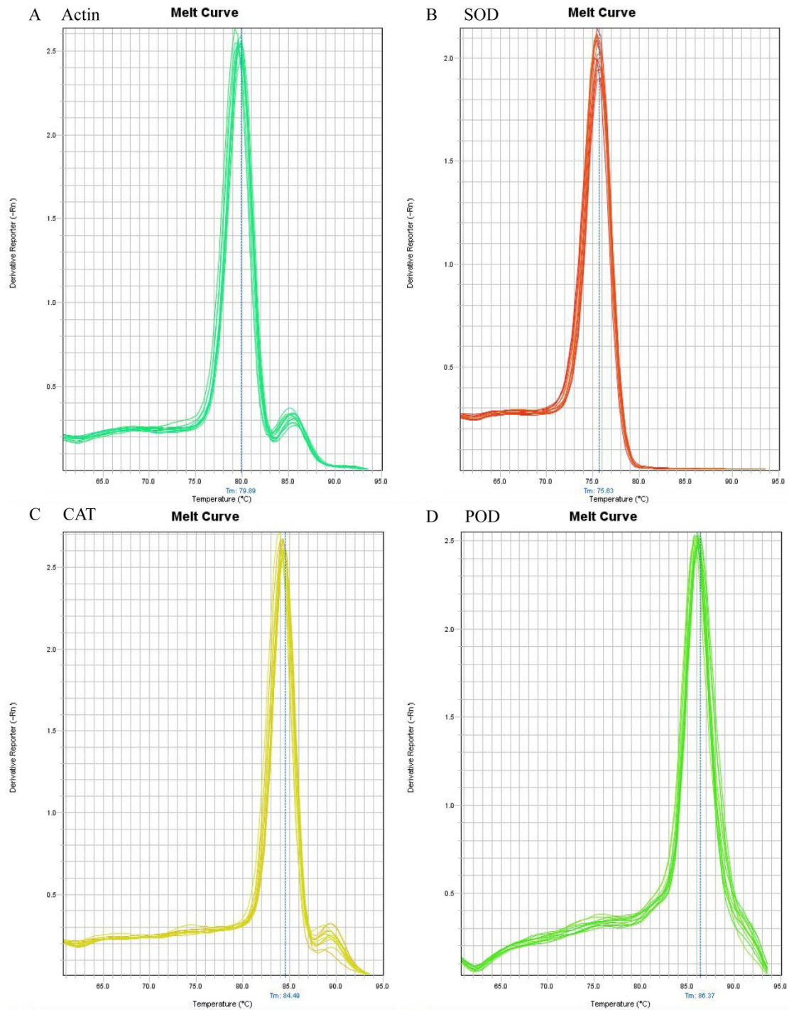
Figure S1. Dissociation curves for housekeeping gene ( \beta -actin) (A) and antioxidant genes SOD (B), CAT (C), and POD (D) with single peak.
