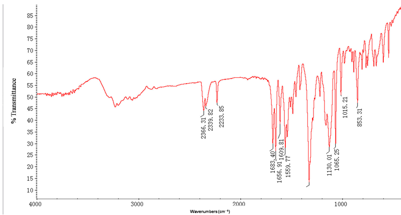
Figure S33. IR of compound 4h.
