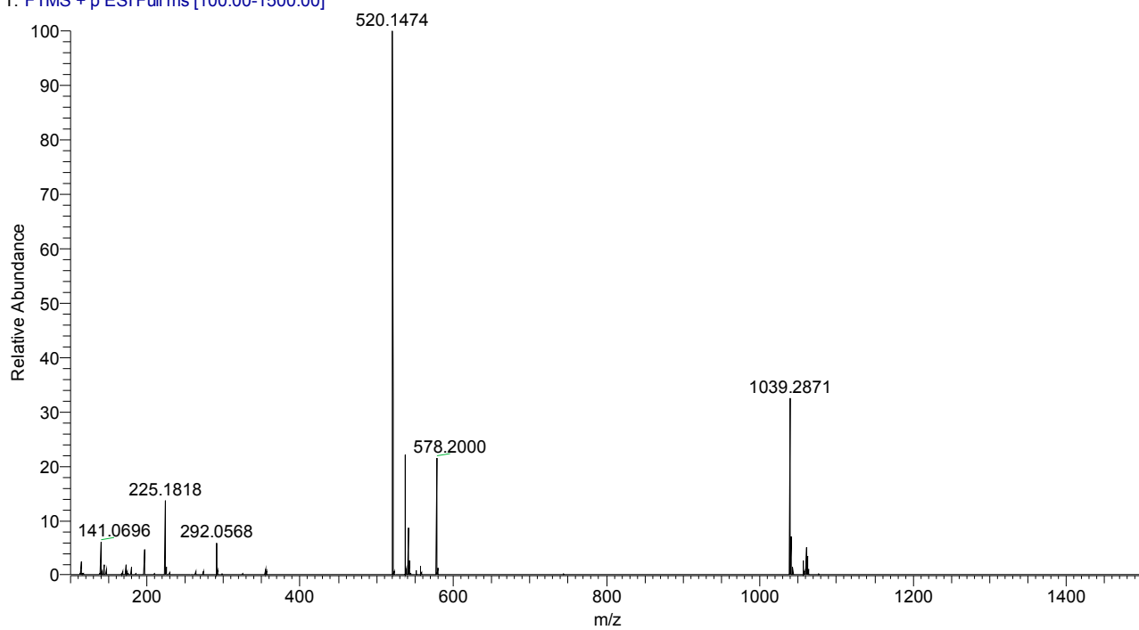
Figure S5. HR-ESI-MS of compound 3b.
