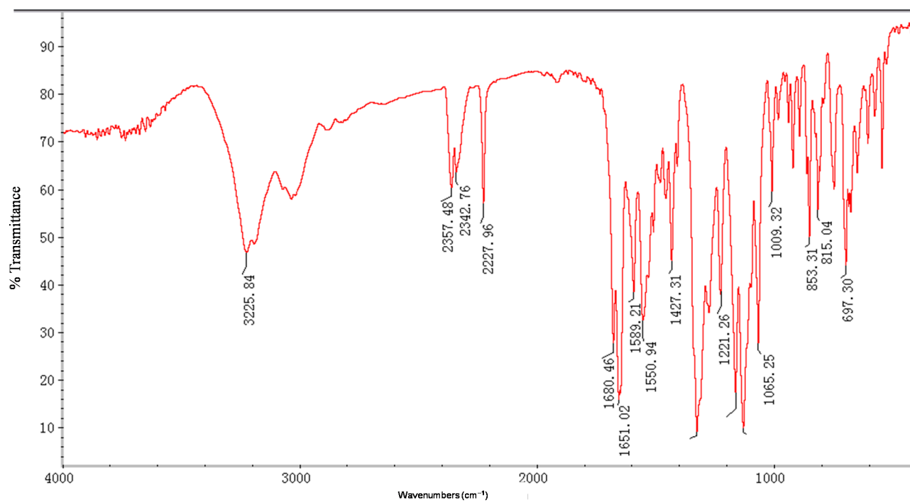
Figure S18. IR of compound 4c.
