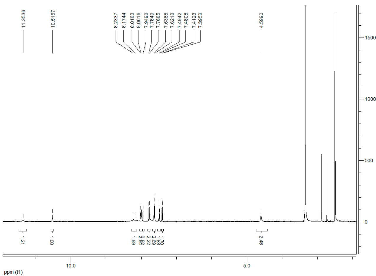
Figure S22. 1 H-NMR spectra of compound 4e.
