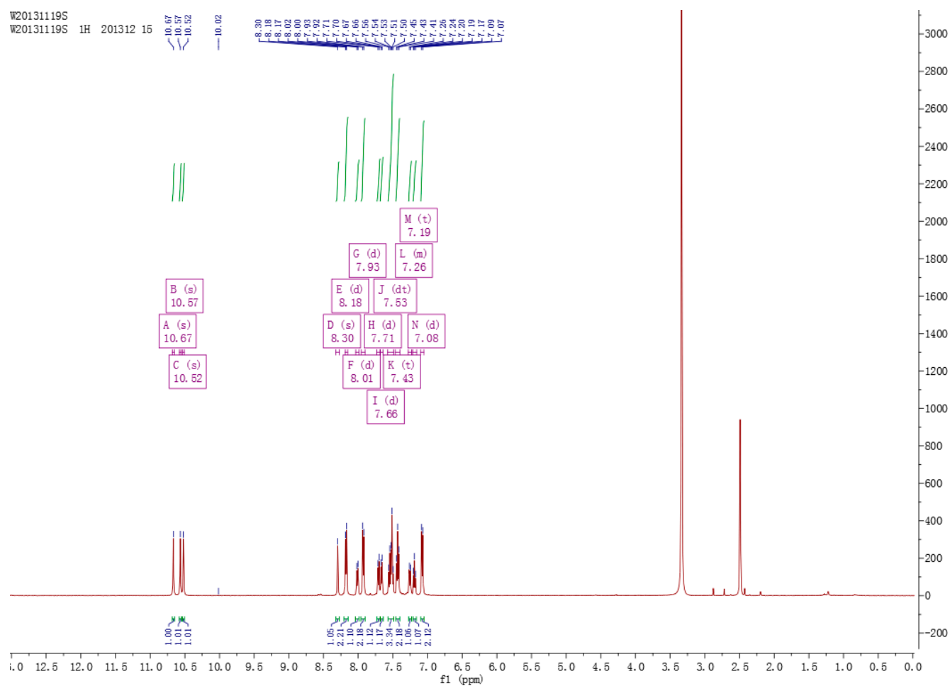
Figure S4. 1 H-NMR of compound 3b.
