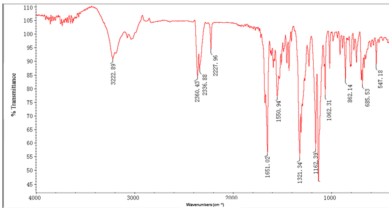
Figure S15. IR spectra of compound 4b.
