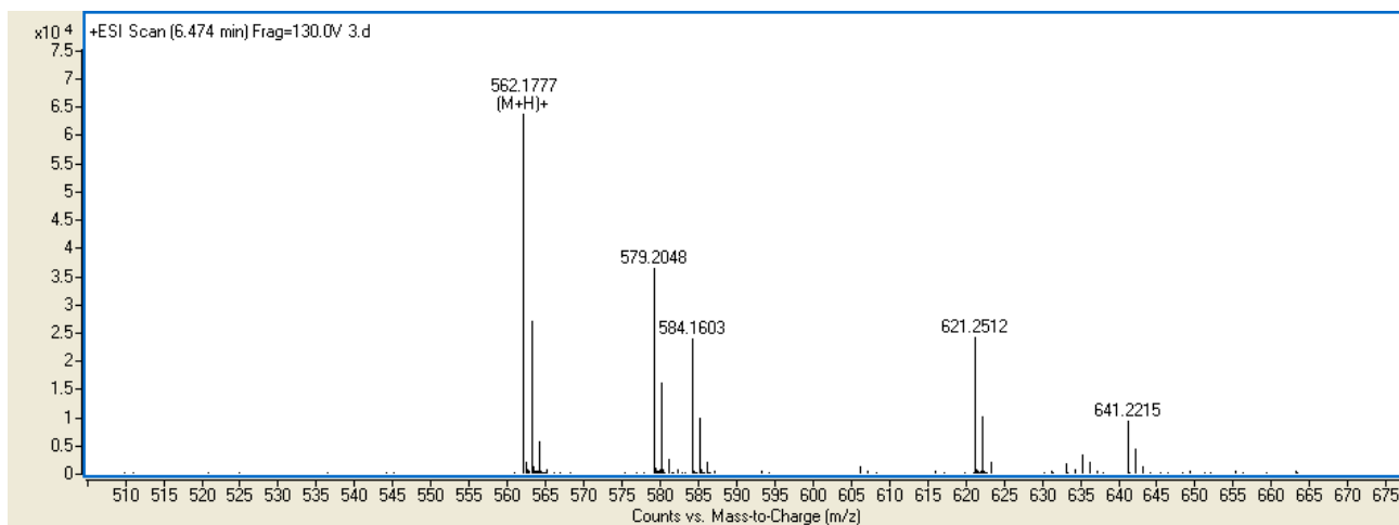
Figure S9. HR-ESI-MS of compound 3d .
