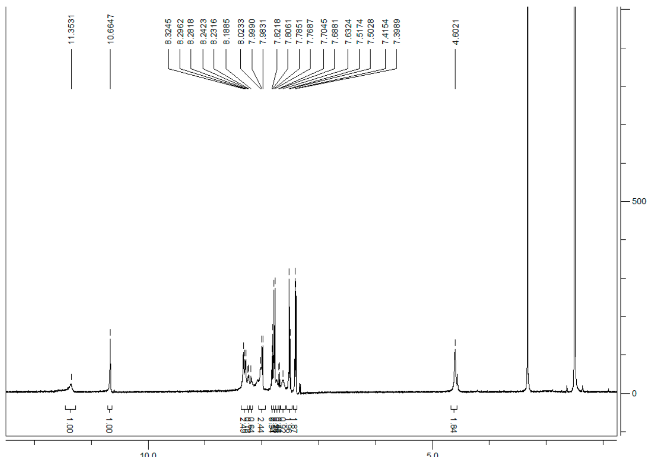
Figure S34. 1 H-NMR spectra of compound 4i.
