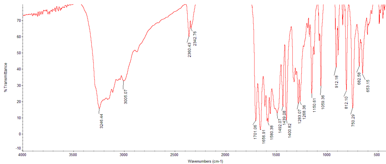
Figure S3. IR of compound 3a.
