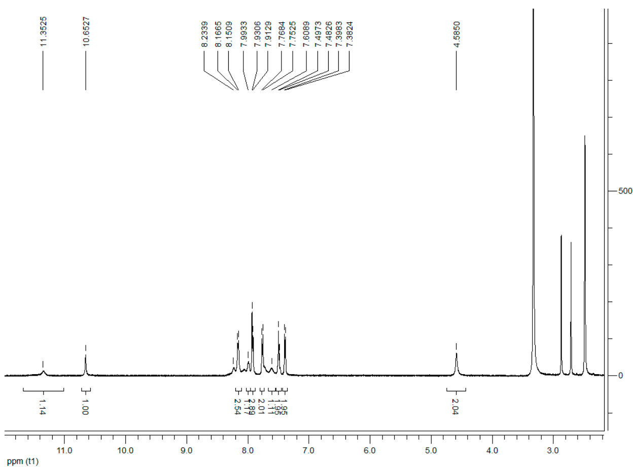
Figure S14. 1 H-NMR spectra of compound 4b.
