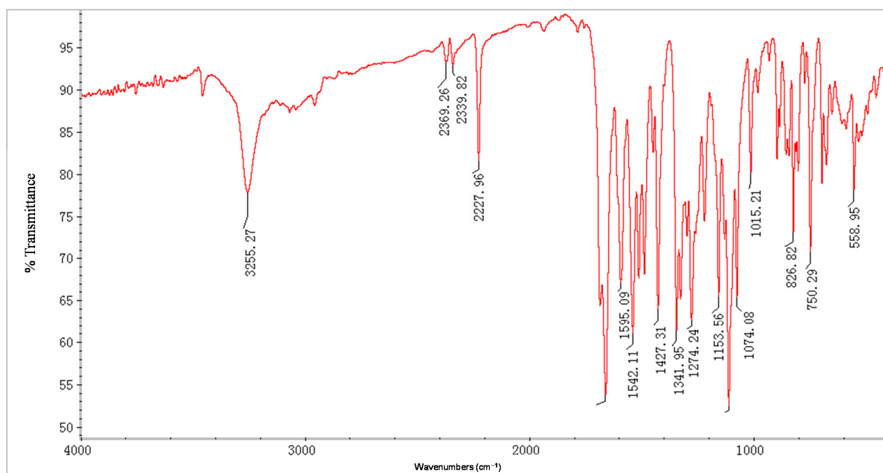
Figure S24. IR of compound 4e.
