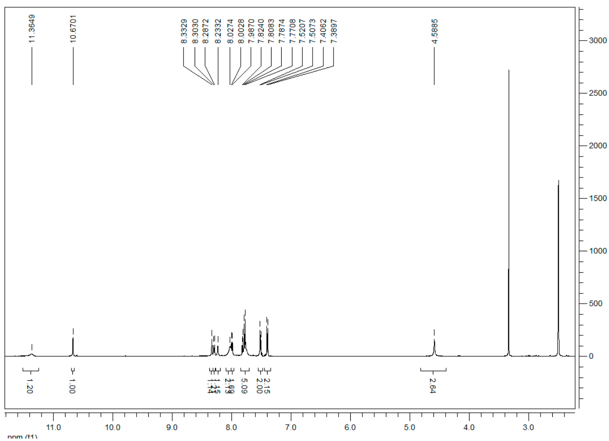
Figure S16. 1 H-NMR spectra of compound 4c.
