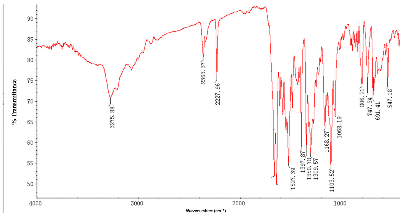
Figure S30. IR spectra of compound 4g .
