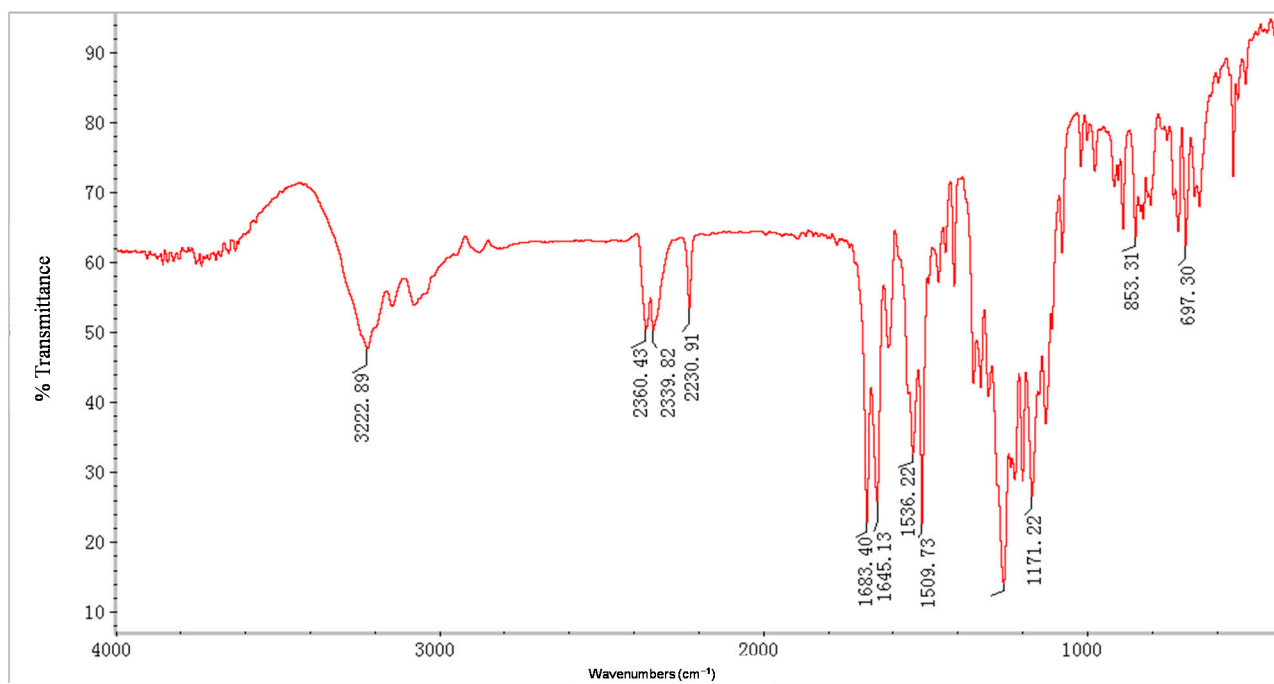
Figure S45. IR of compound 4I .
