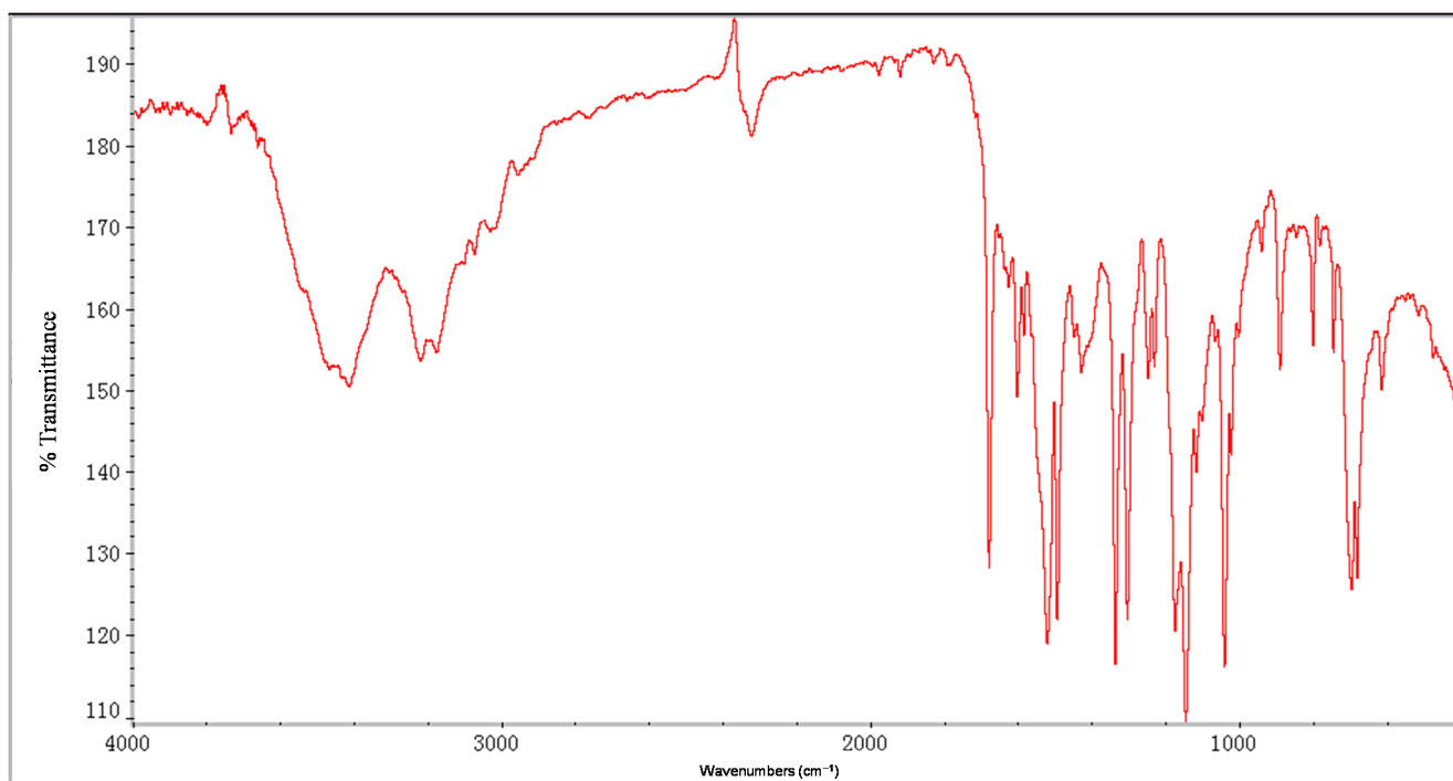
Figure S7. IR of compound 3c.
