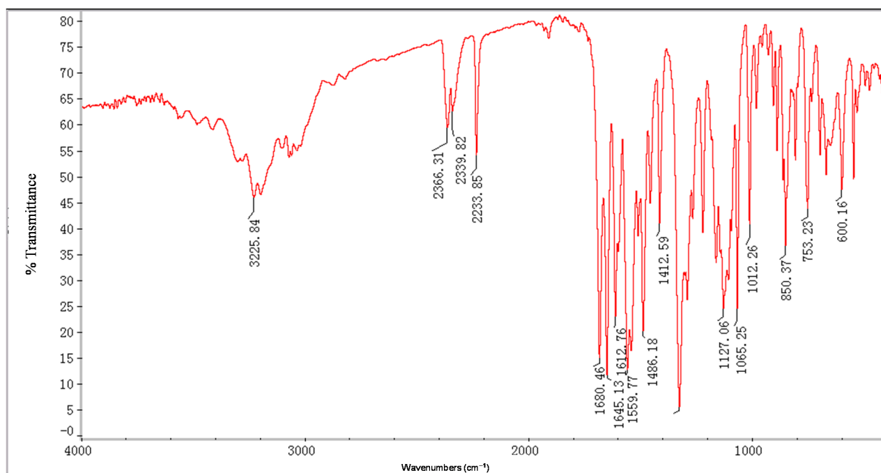
Figure S42. IR of compound 4k.
