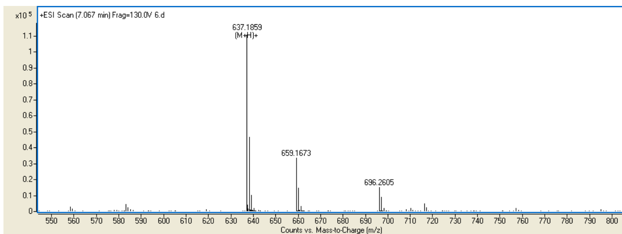
Figure S26. MS of compound 4f .
