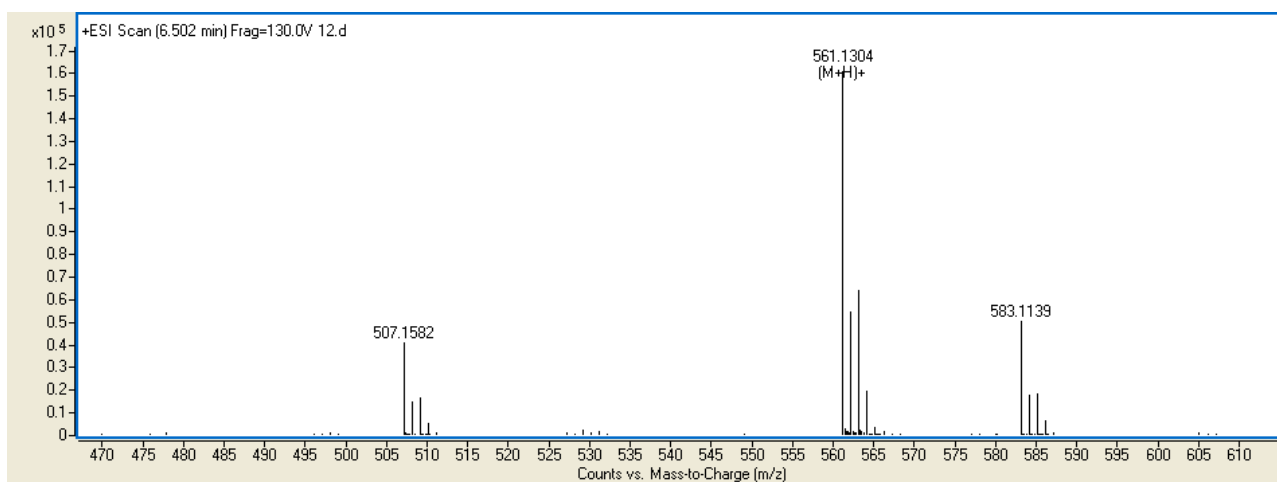
Figure S41. MS of compound 4k w201312111.
