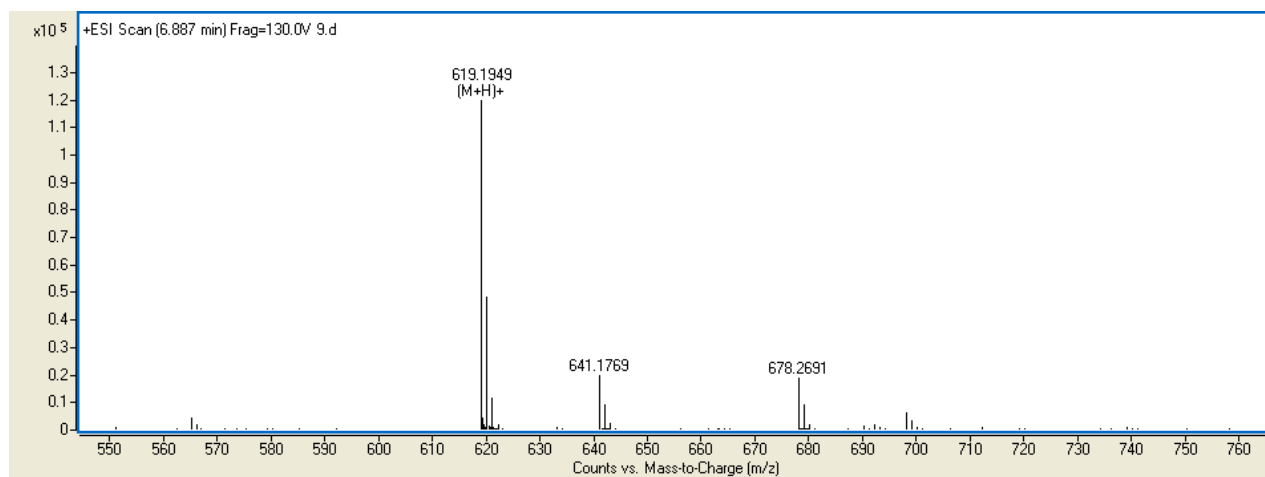
Figure S38. MS of compound 4j .
