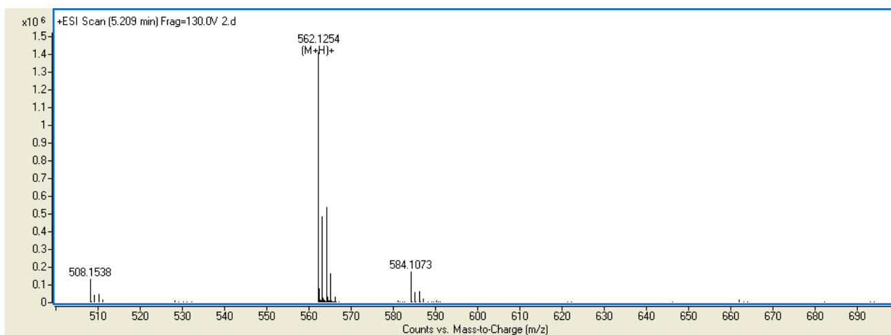
Figure S29. MS spectra of compound 4g .
