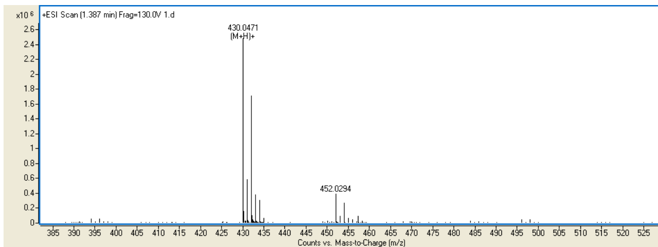
Figure S2. HR-ESI-MS of compound 3a .
