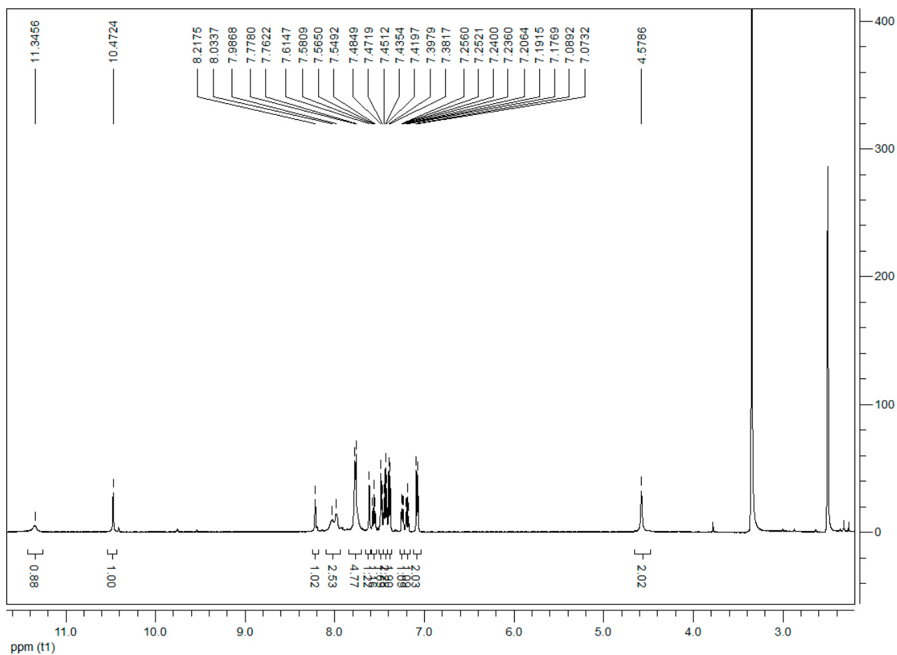
Figure S37. ^1\text{H-NMR} spectra of compound 4j .
