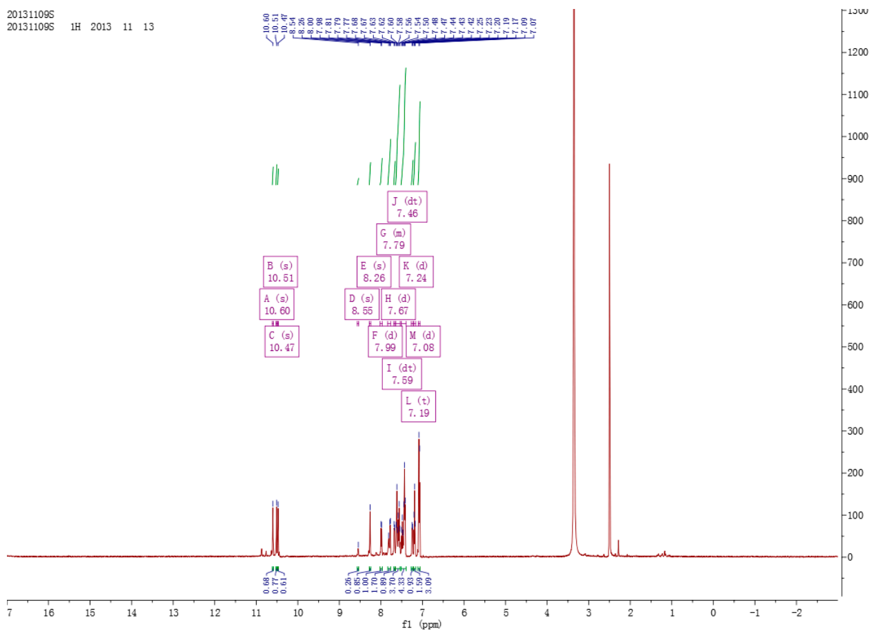
Figure S8. 1 H-NMR of compound 3d.
