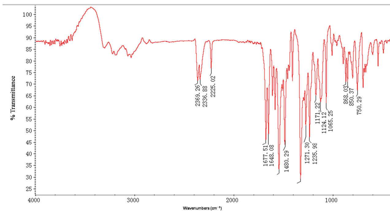
Figure S39. IR of compound 4j.
