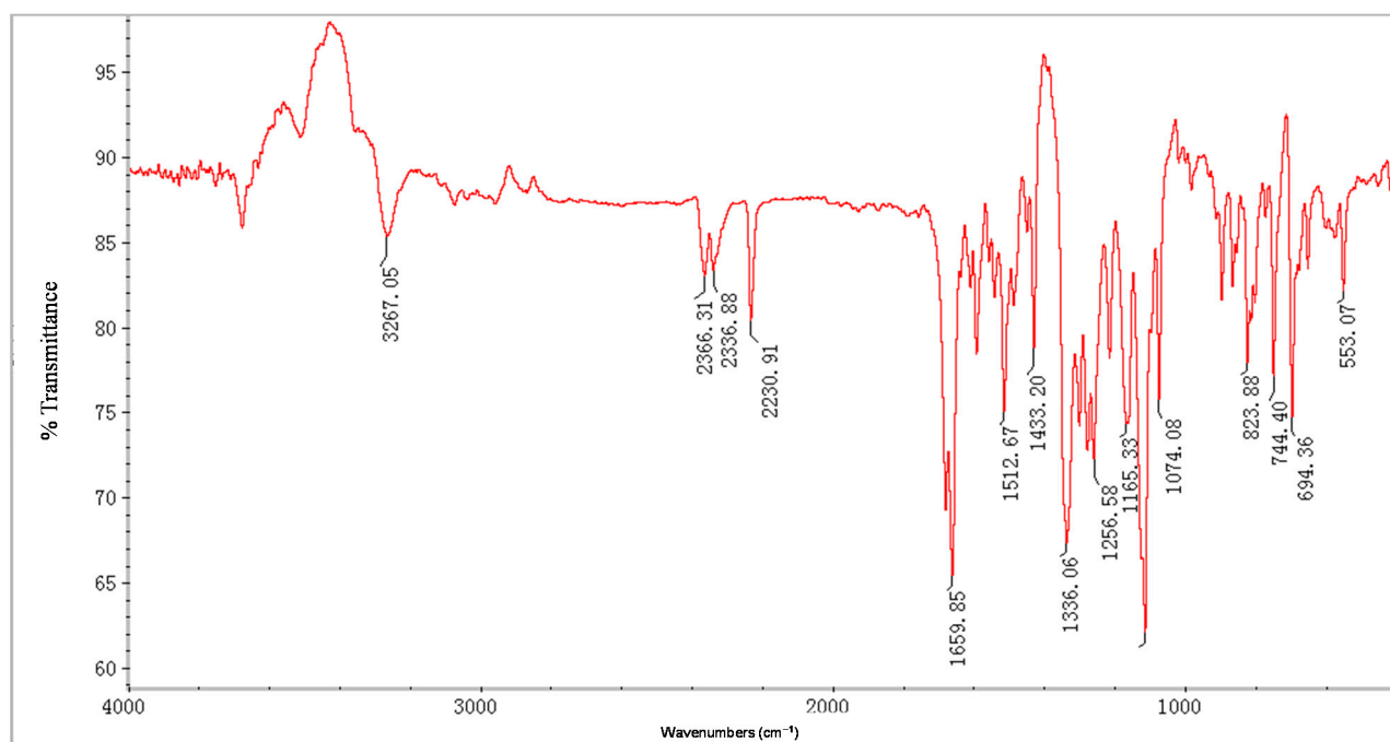
Figure S36. IR spectra of compound 4i.
