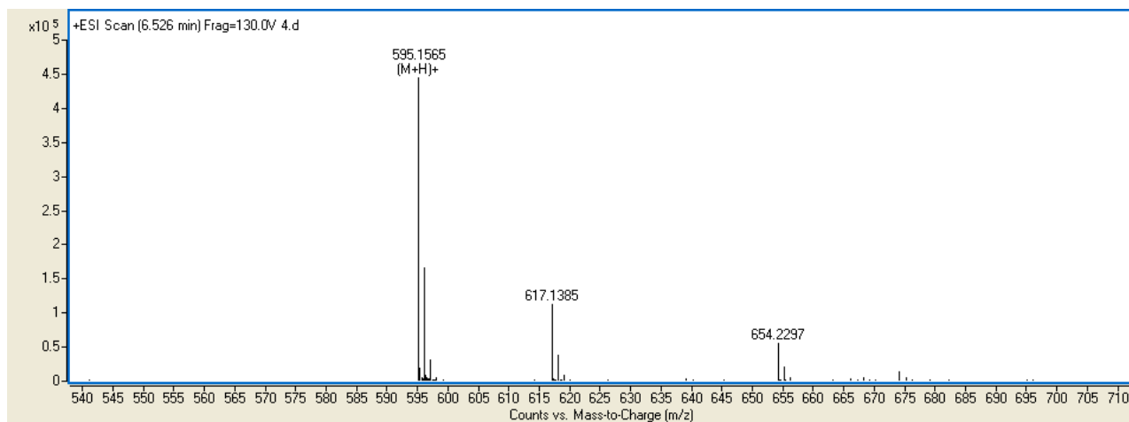
Figure S35. MS spectra of compound 4i.
