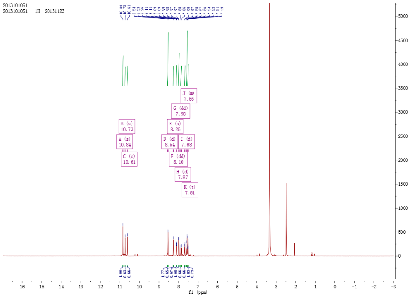
Figure S1. ^1\text{H-NMR} of compound 3a .
