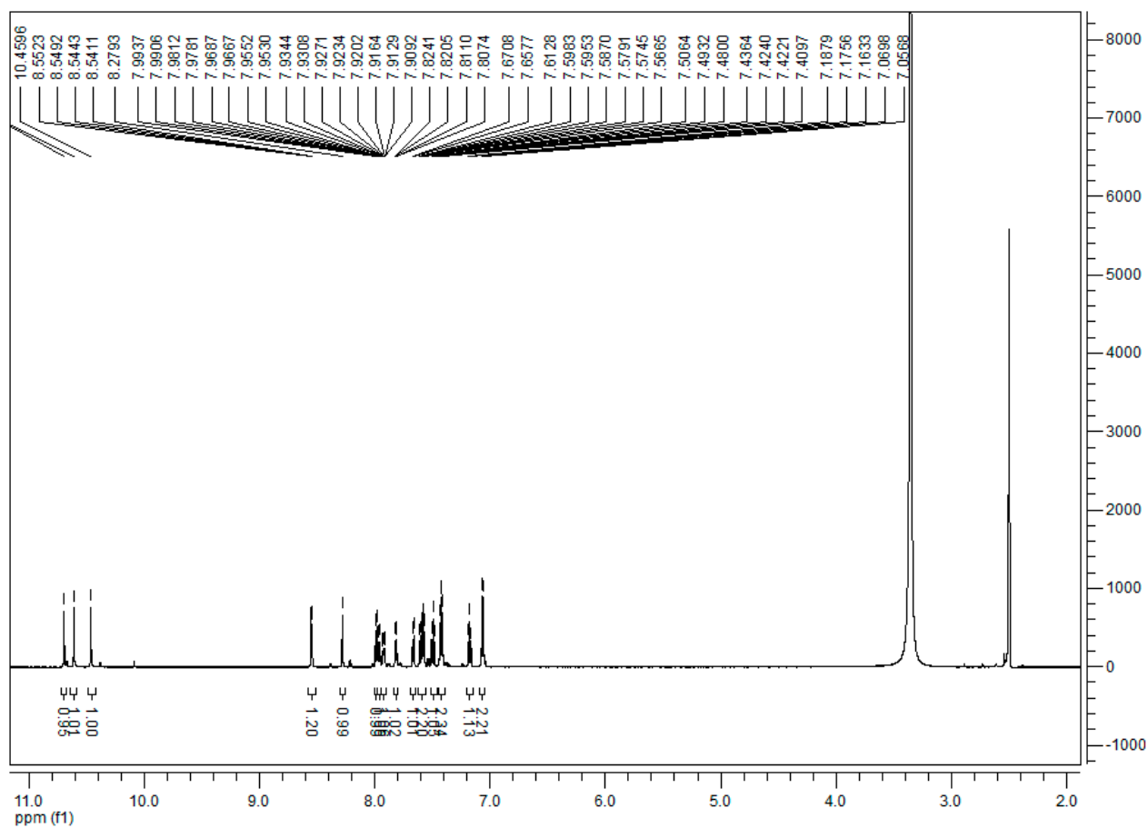
Figure S6. ^1\text{H-NMR} of compound 3c.
