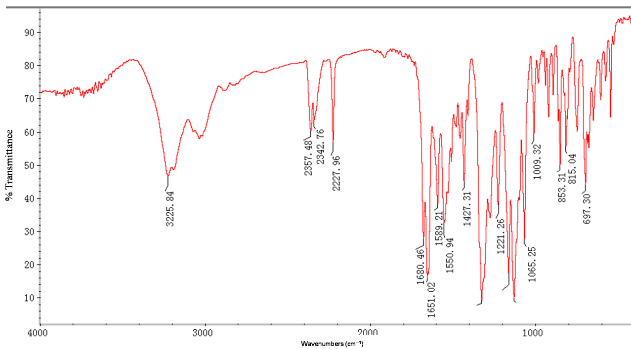
Figure S13. IR spectra of compound 4a.
