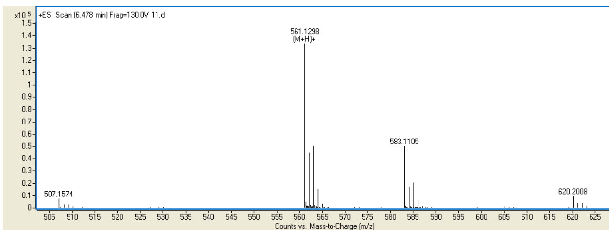
Figure S23. MS of compound 4e.
