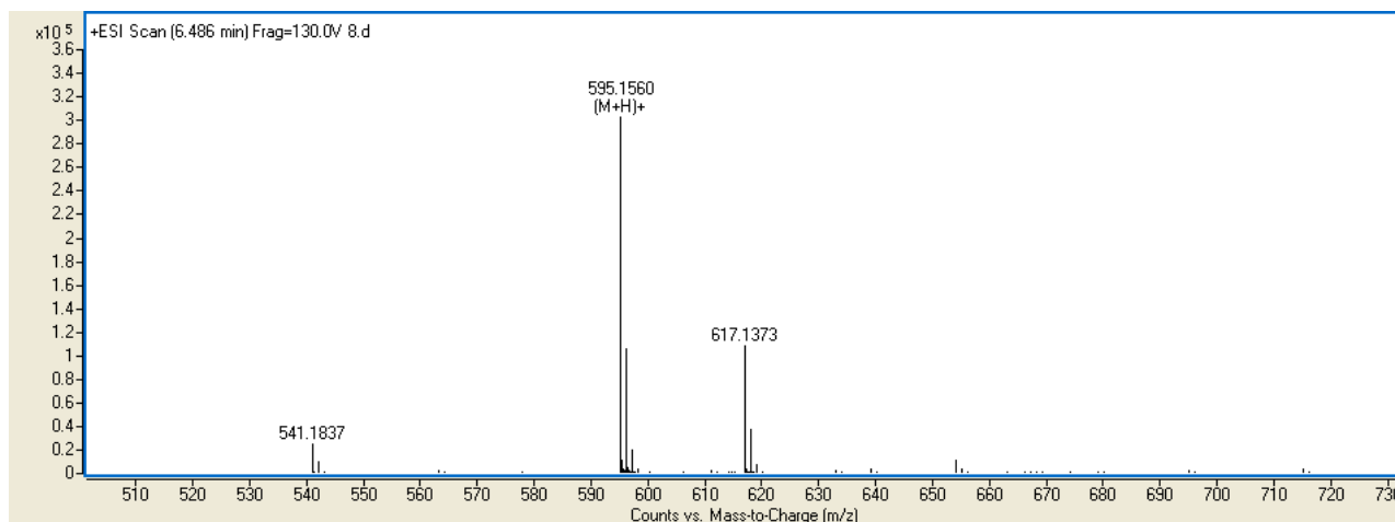
Figure S17. MS of compound 4c.
