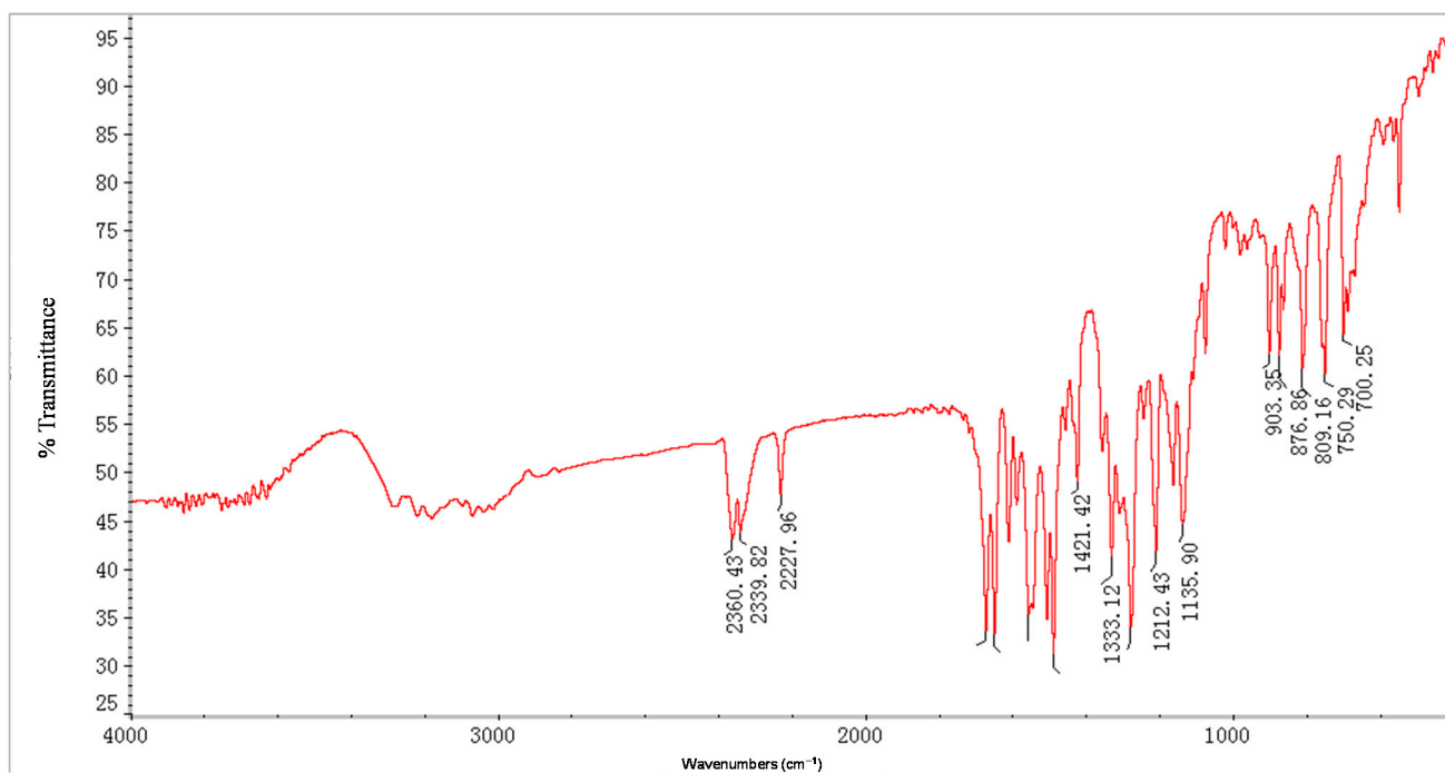
Figure S21. IR of compound 4d.
