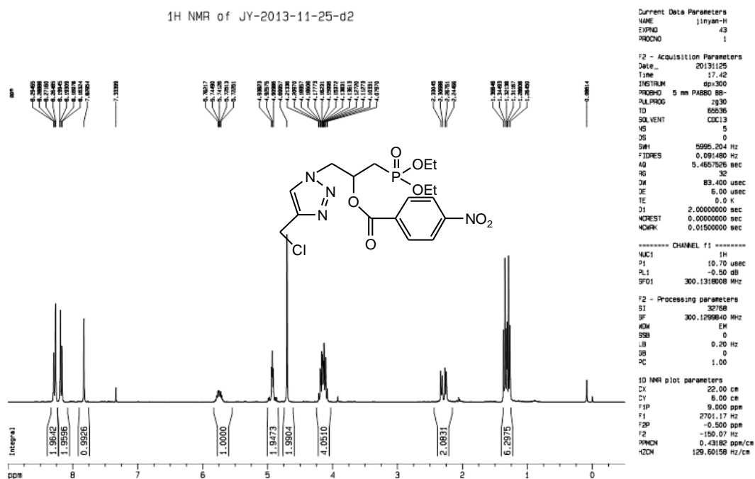
Figure S120. 1 H-NMR spectrum of compound 5-D2.
