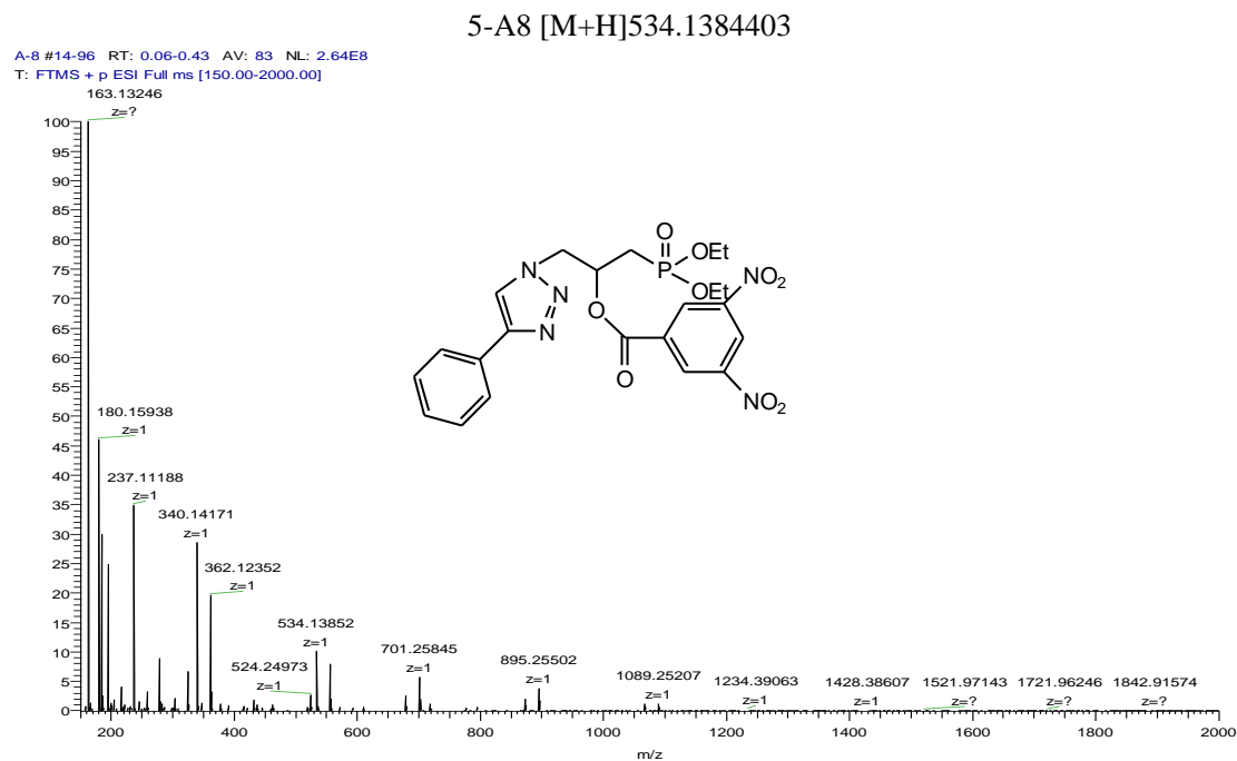
Figure S40. HRMS spectrum of compound 5-A8
