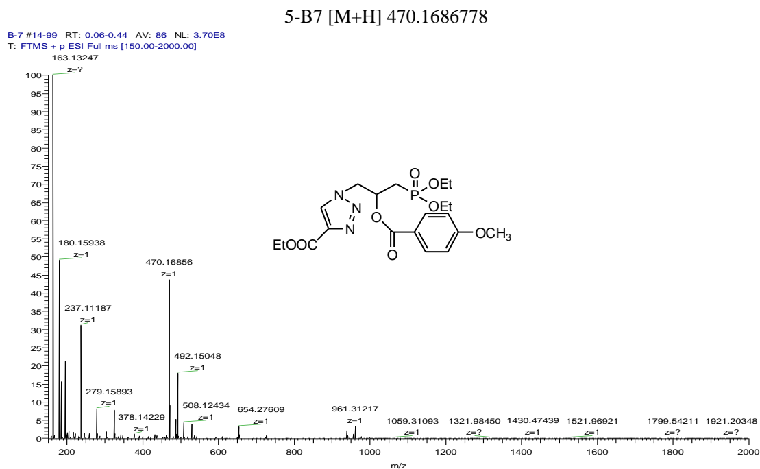
Figure S74. HRMS spectrum of compound 5-B7.
