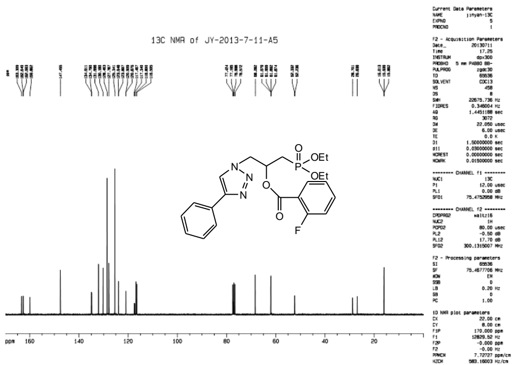
Figure S22. 13 C-NMR spectrum of compound 5-A5.
