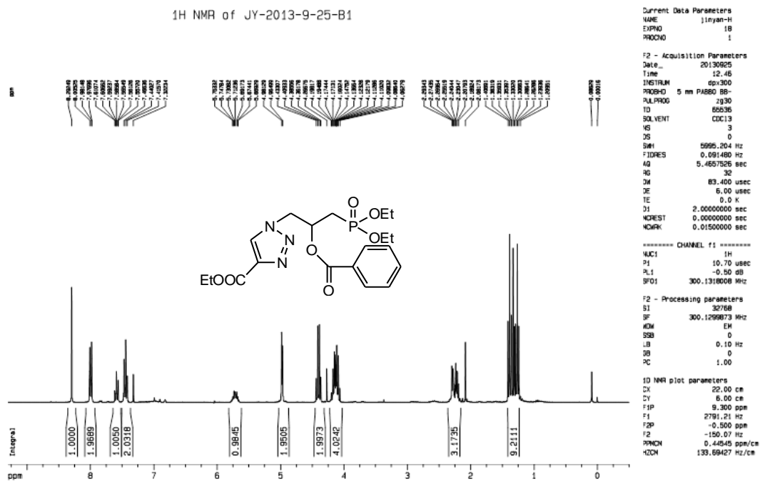
Figure S41. 1 H-NMR spectrum of compound 5-B1.
