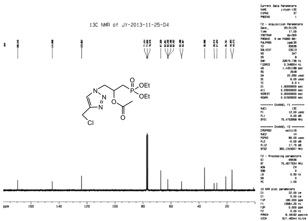
Figure S131. ^{13}\text{C} -NMR spectrum of compound 5-D4.
