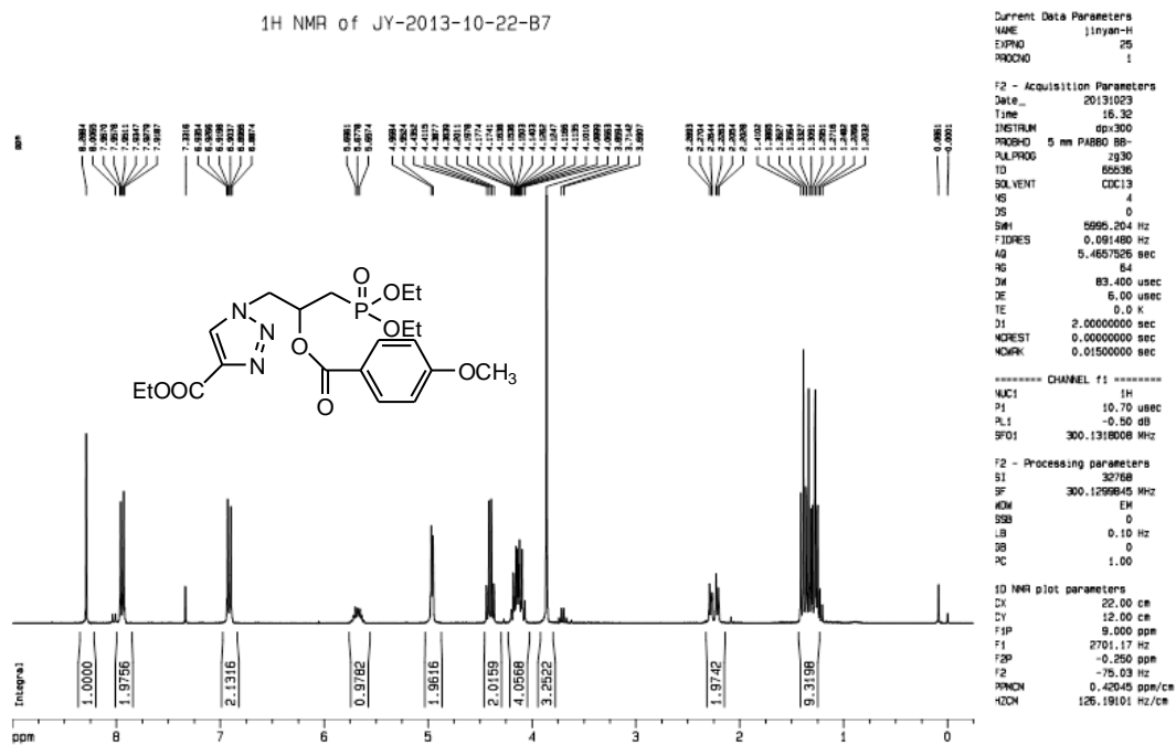
Figure S71. 1 H-NMR spectrum of compound 5-B7.
