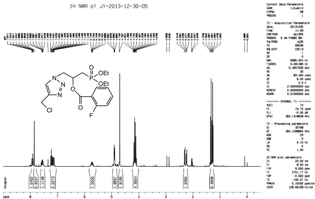
Figure S135. ^1\text{H-NMR} spectrum of compound 5-D5.
