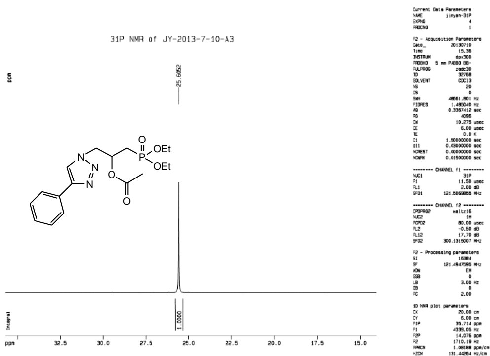
Figure S18. ^{31}\text{P} -NMR spectrum of compound 5-A4.
