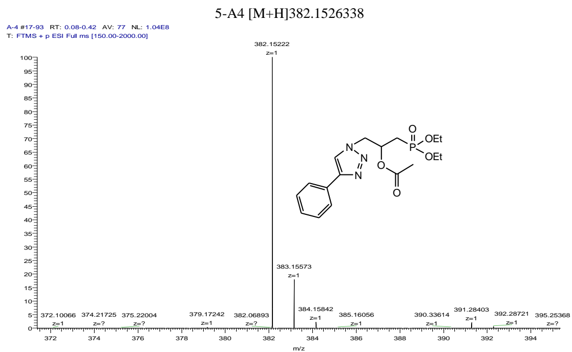
Figure S20. HRMS spectrum of compound 5-A4.
