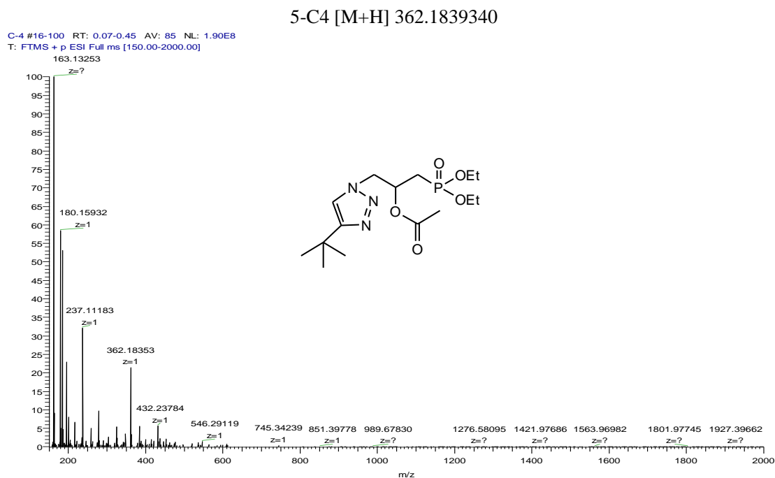
Figure S98. HRMS spectrum of compound 5-C4.
