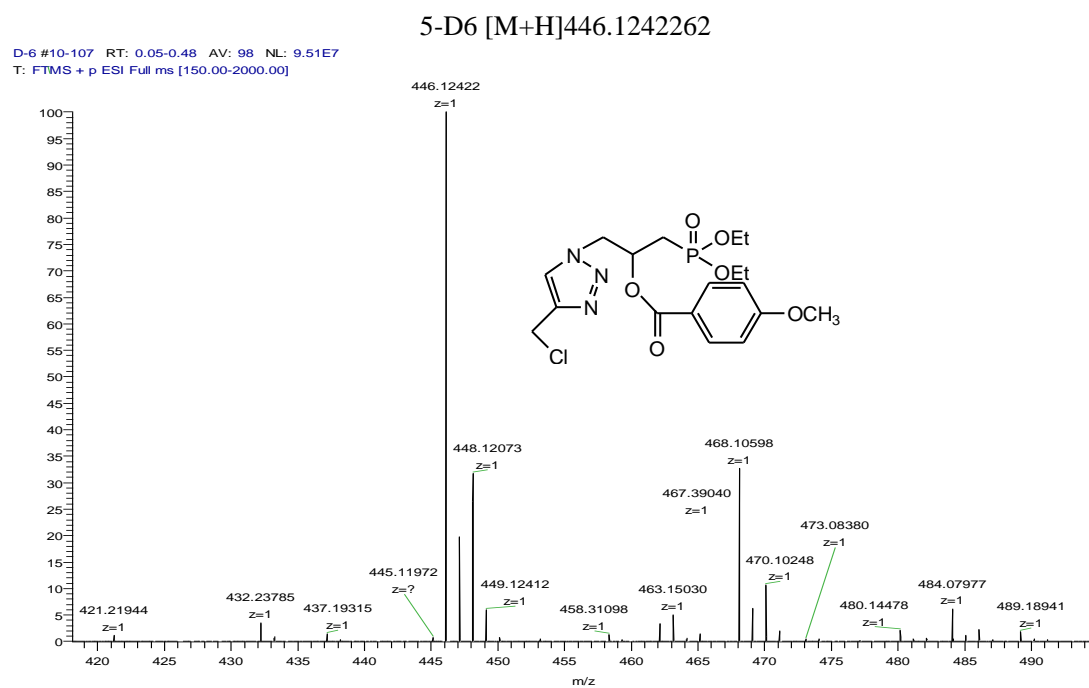
Figure S144. HRMS spectrum of compound 5-D6.
