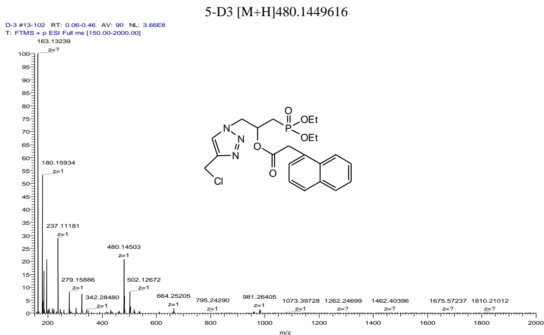
Figure S128. HRMS spectrum of compound 5-D3.
