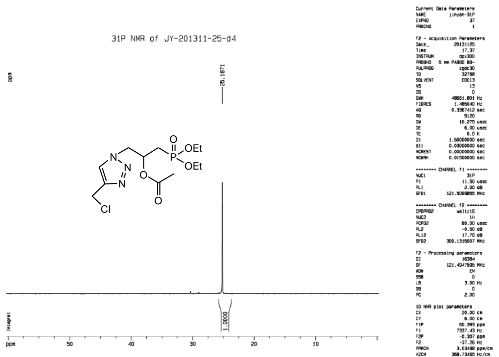
Figure S132. ^{31}\text{P} -NMR spectrum of compound 5-D4.
