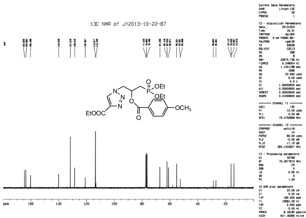
Figure S72. 13 C-NMR spectrum of compound 5-B7.
