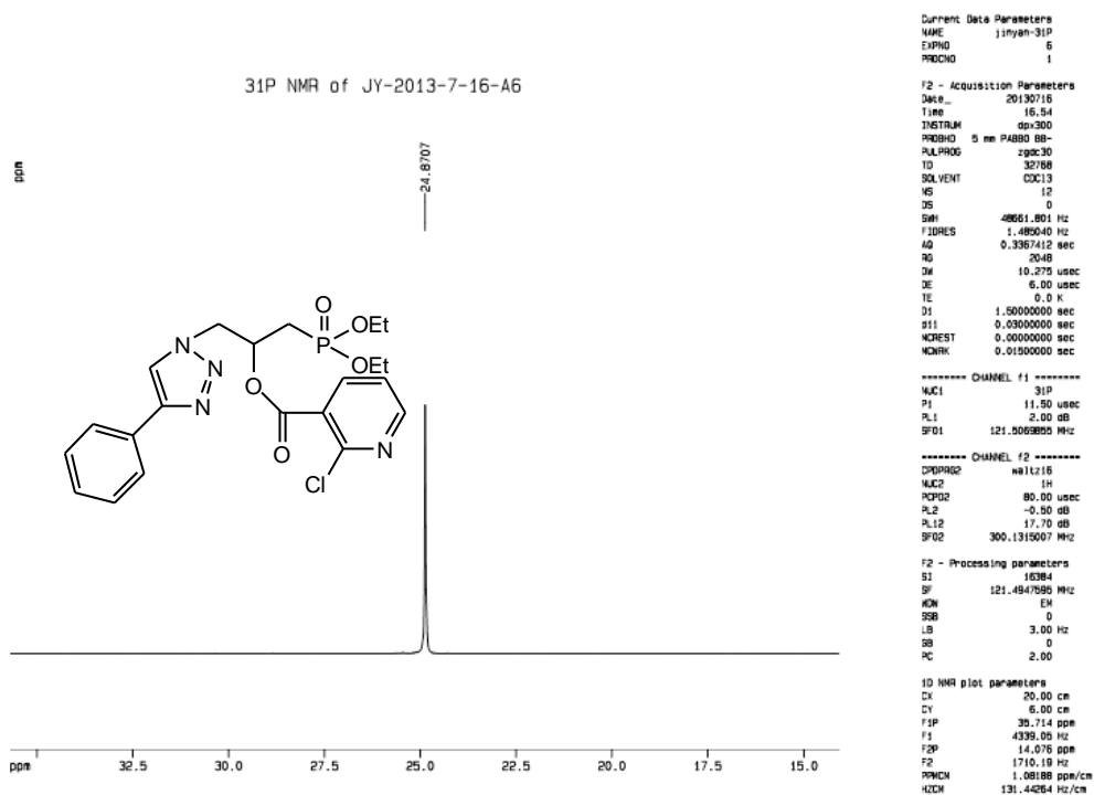
Figure S28. ^{31}\text{P} -NMR spectrum of compound 5-A6.
