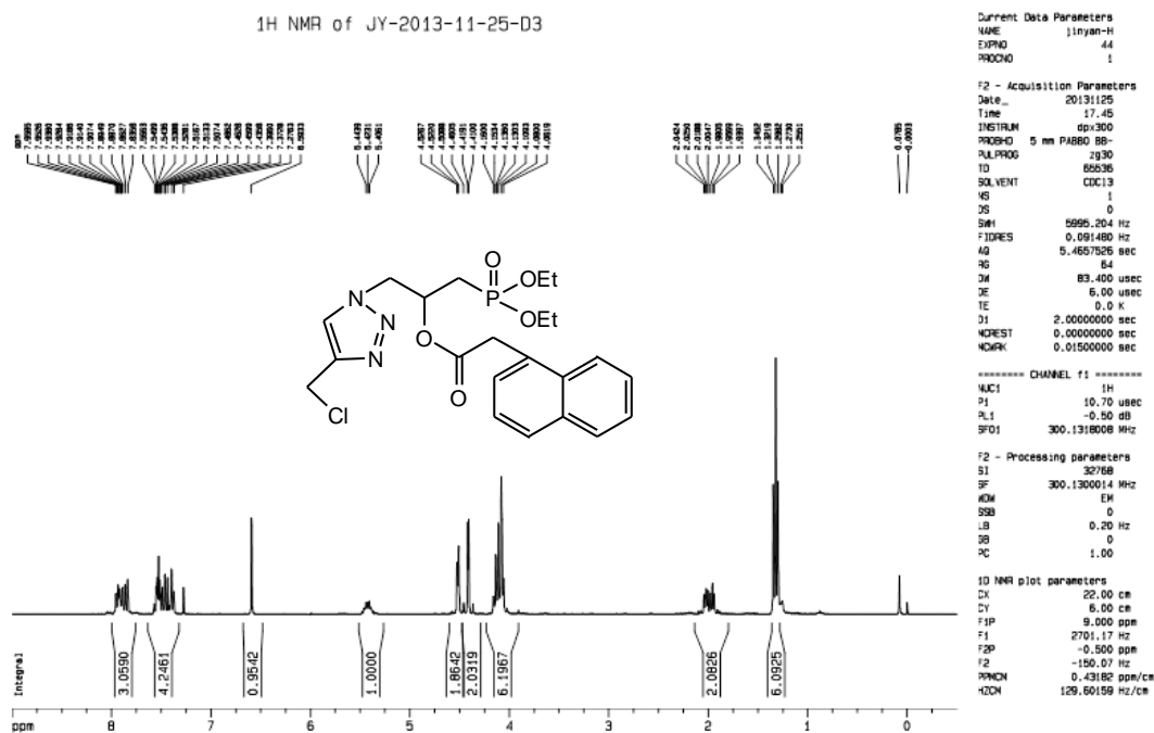
Figure S125. ^1\text{H} -NMR spectrum of compound 5-D3.
