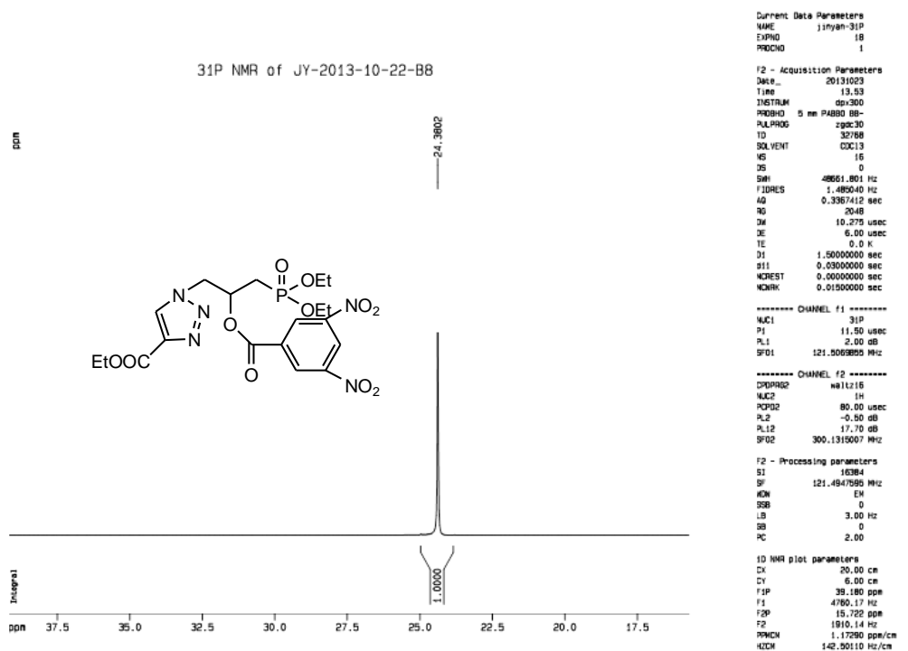
Figure S78. ^{31}\text{P} -NMR spectrum of compound 5-B8.
