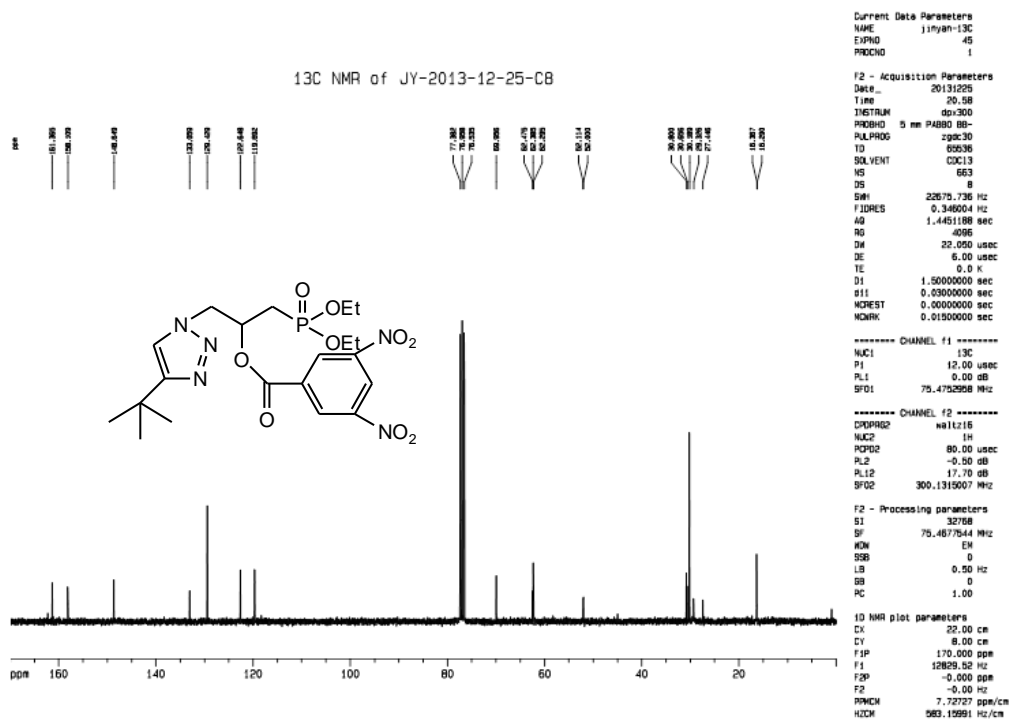
Figure S111. ^{13}\text{C} -NMR spectrum of compound 5-C7.
