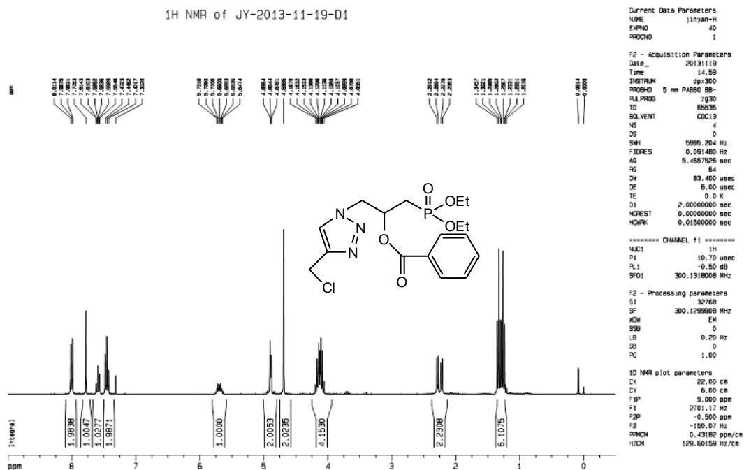
Figure S115. 1 H-NMR spectrum of compound 5-D1.
