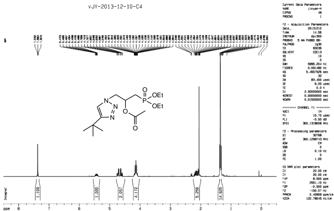
Figure S95. 1 H-NMR spectrum of compound 5-C4.
