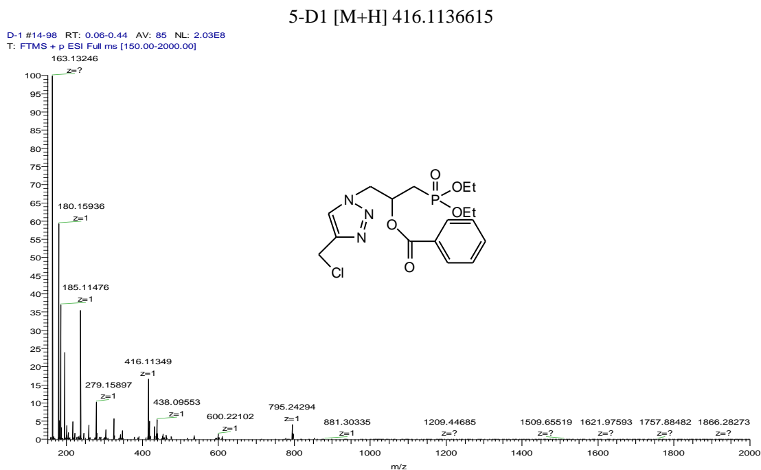
Figure S118. HRMS spectrum of compound 5-D1.
