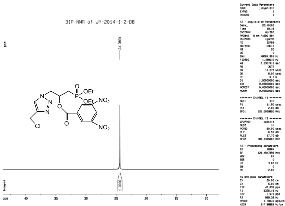
Figure S147. ^{31}\text{P} -NMR spectrum of compound 5-D7.
