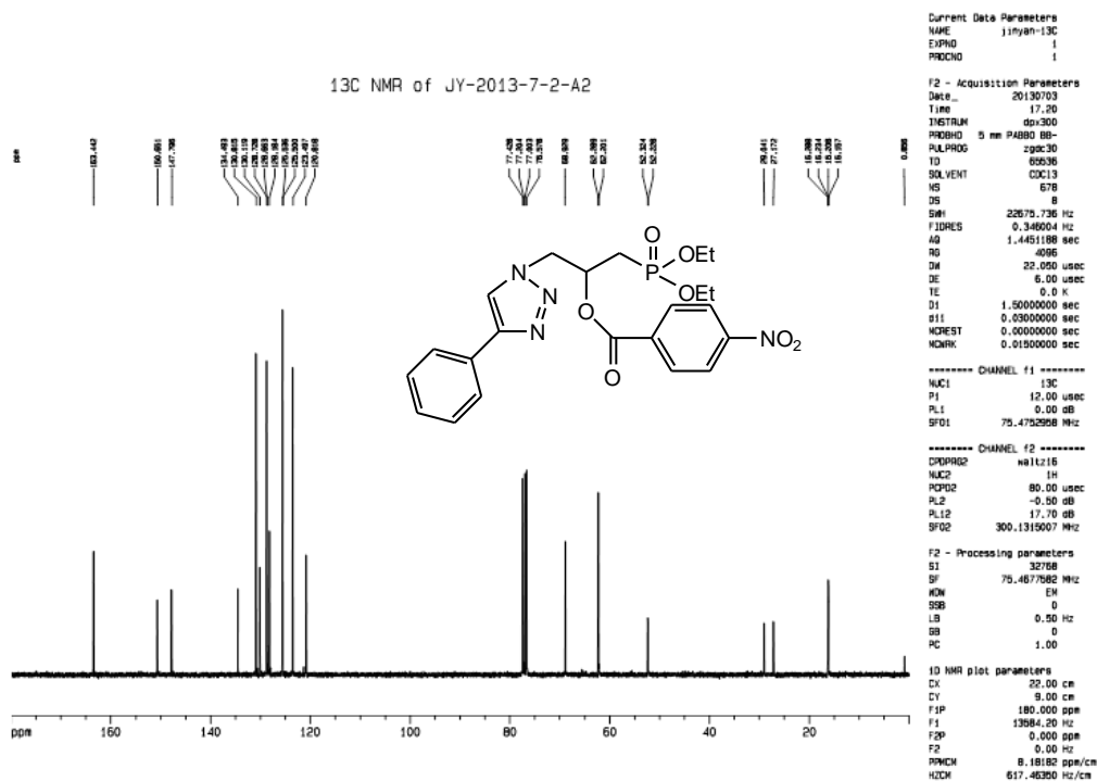
Figure S7. ^{13}\text{C} -NMR spectrum of compound 5-A2.
