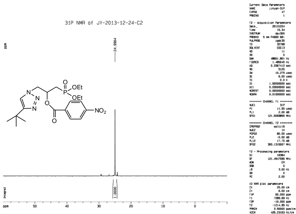
Figure S87. ^{31}\text{P} -NMR spectrum of compound 5-C2.
