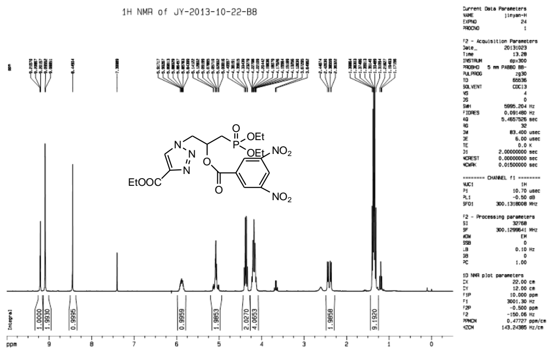
Figure S76. 1 H-NMR spectrum of compound 5-B8.
