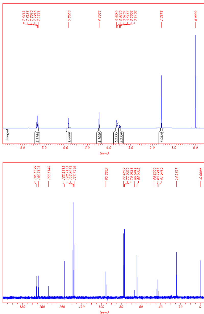
Figure S1. (E)-3-Benzyl-4,4-dimethyl-5-(2-morpholin-4-yl-2-oxoethylidene)oxazolidin-2-one (3aa-E). Top: 1 H-NMR (CDCl 3 ); bottom: 13 C-NMR (CDCl 3 ).
