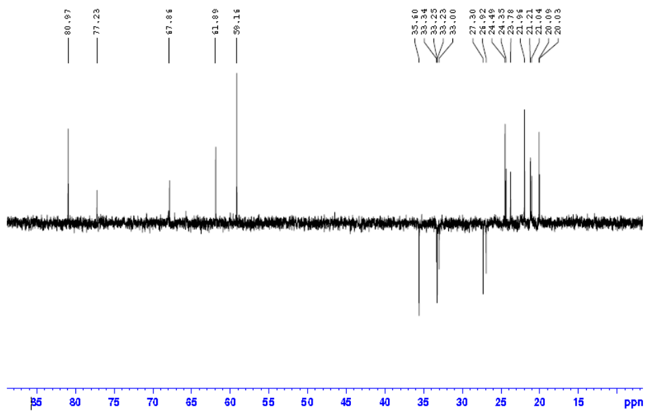
Figure S3. DEPT 135 of Compound 8.
