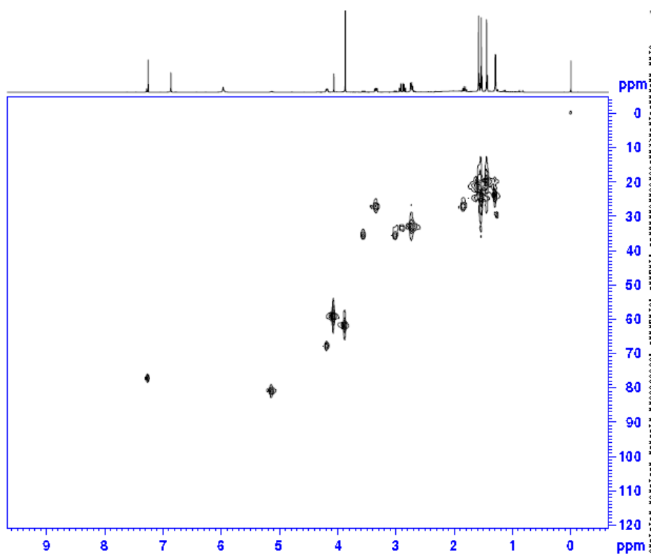
Figure S5. HSQC of Compound 8.
