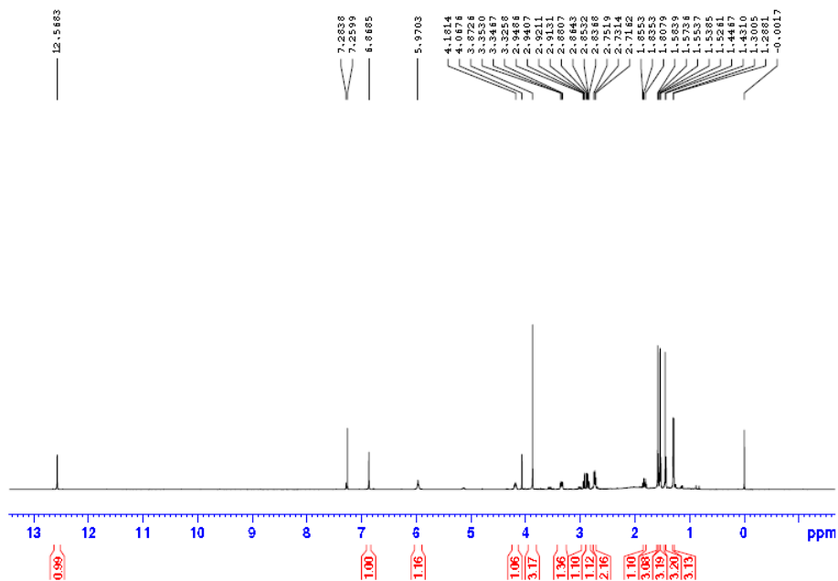
Figure S1. ^1\text{H-NMR} of Compound 8.
