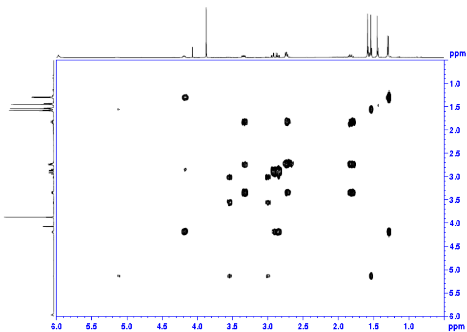
Figure S4. ^1\text{H} - ^1\text{H} COSY of Compound 8.
