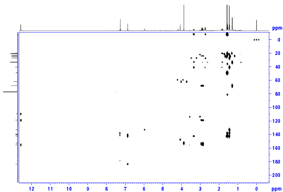
Figure S6. HMBC of Compound 8.
