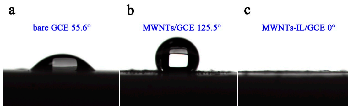
Figure S1. Water contact angle of bare GCE (a), MWNTs/GCE (b) and MWNTs-IL/GCE (c).
