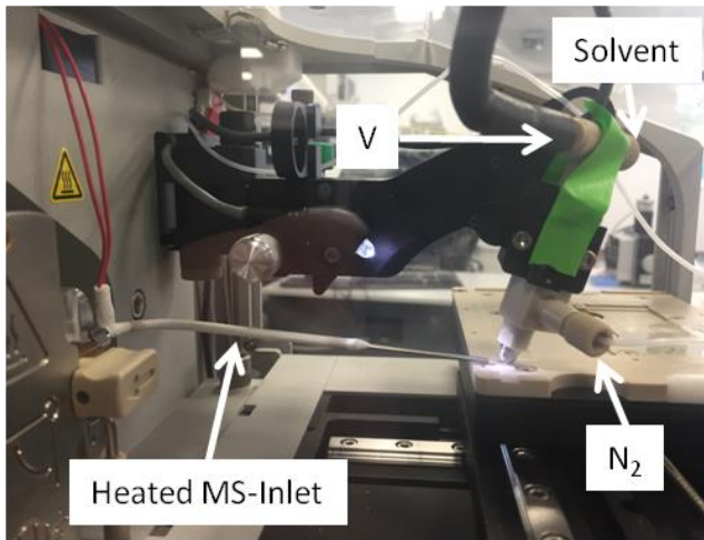
On line resource 1. Modified sprayer setup, showing additional t-junction isolating the voltage from the sprayer body and the heated MS-inlet.
