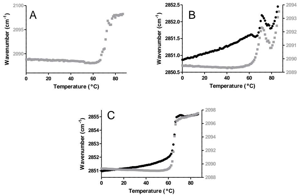
Supplemental Figure S3 \nu curves of (A) dFFA, (B) LB-dNS/dC24 and (C) LB-dNS/dFFA. CD 2 curves (■) and CH 2 curves (●) show transition from ordered to disordered phase at the same temperature for each sample.
