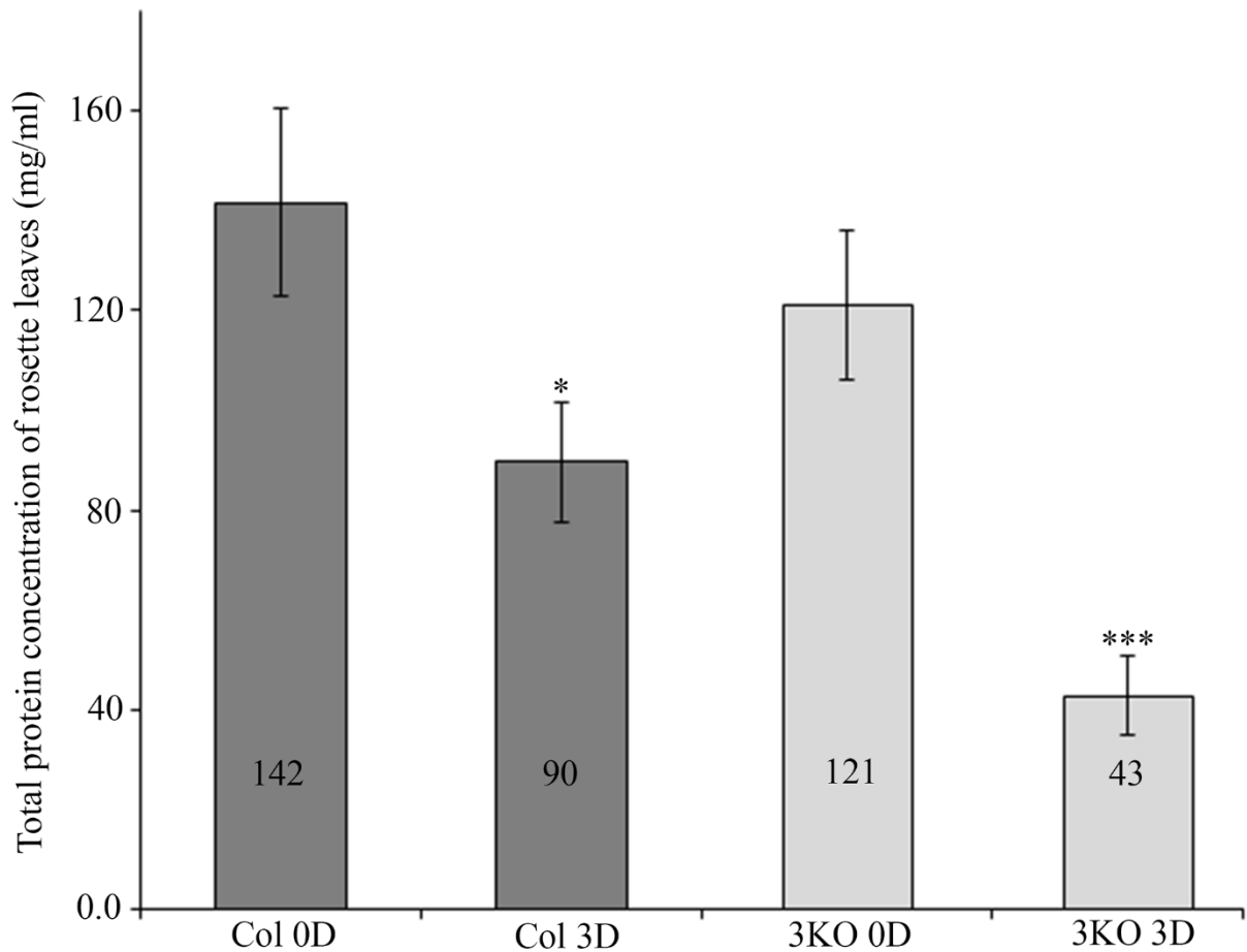
Supplementary Figure 5. The total protein content of leaf extracts before and after dark treatment. After dark-treatment, the total protein concentration of Col leaves was 1.6-fold lower (Col 3D) and the one of 3KO leaves was 2.8-fold lower (3KO 3D), in comparison with untreated controls
