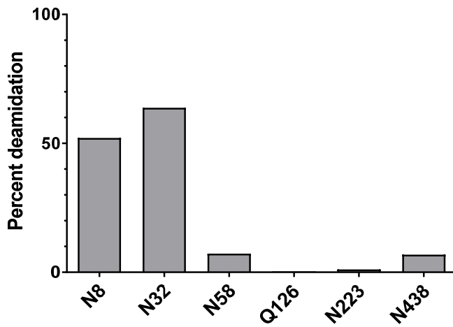
Figure S2. Deamidation frequencies in non-AAV proteins. Deamidation percentages are shown for two non-AAV recombinant proteins containing NG motifs likely to be deamidated, human carbonic anhydrase (A) and rat phenylalanine-hydroxylase (B), for comparison with AAV deamidation percentages.
