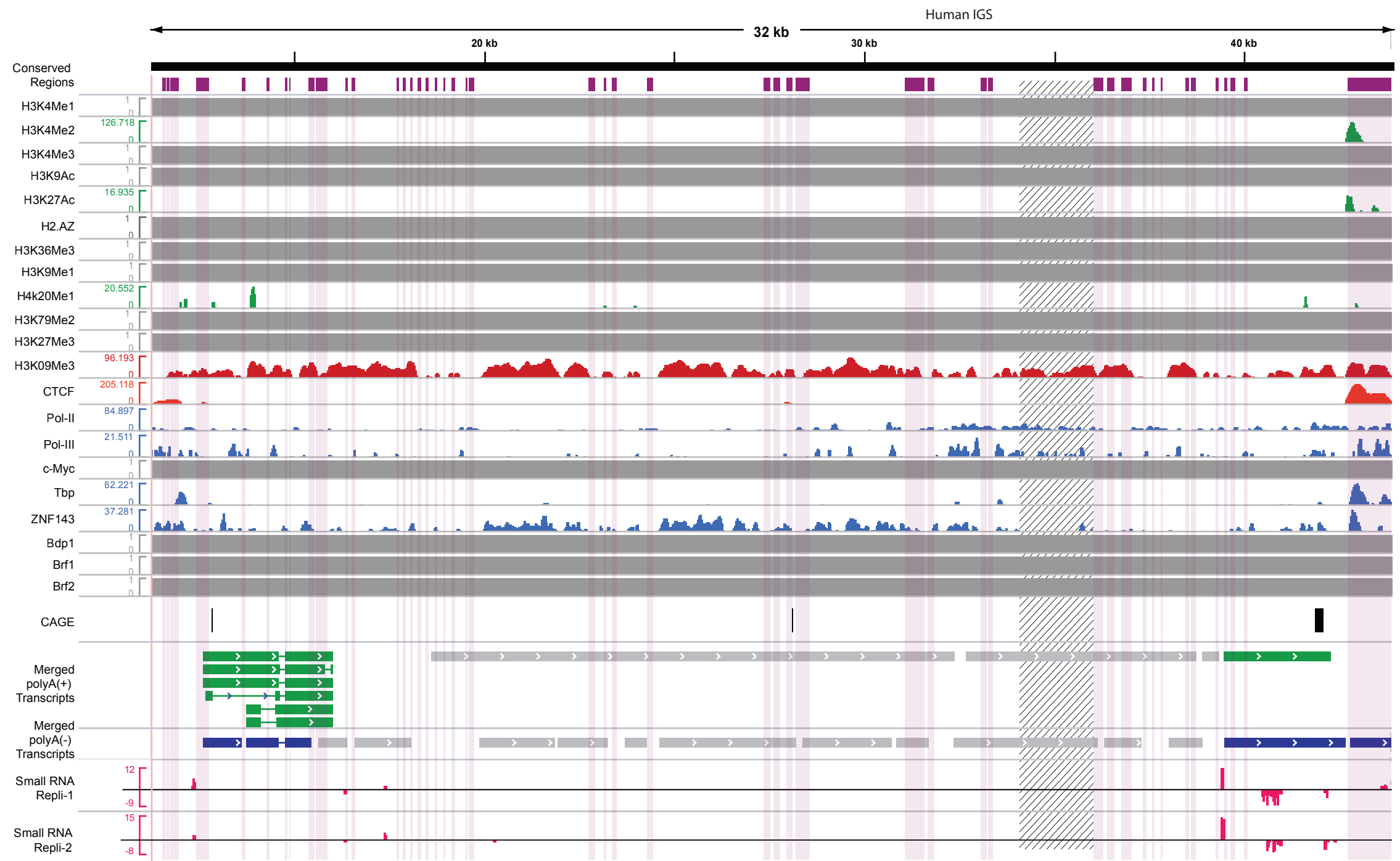
S7 Figure: Chromatin, transcription factor and transcript landscape of the IGS in the lymphoblastoid cell line, GM12878. Figure as for S6 Figure, except that the blue signals represent transcription factors and RNA polymerases, and pink signals indicated small RNA transcripts.
