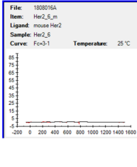
Figure S2. Complete sensorgrams for single-cycle kinetic analysis of V H Hs binding to HER2 by surface plasmon resonance.
