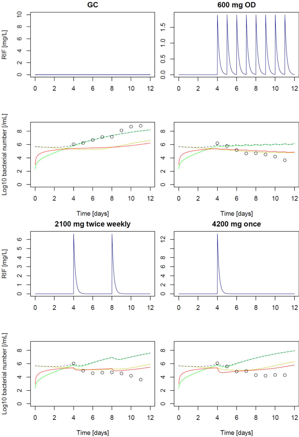
Figure S1: Sensitivity analysis of the translational Multistate Tuberculosis Pharmacometric (MTP) model and prediction of the hollow-fiber experiment; exclusion of the post-antibiotic effect (PAE) model, i.e. direct link of pharmacokinetic and pharmacodynamic. For a detailed figure legend, refer to Figure 2.
